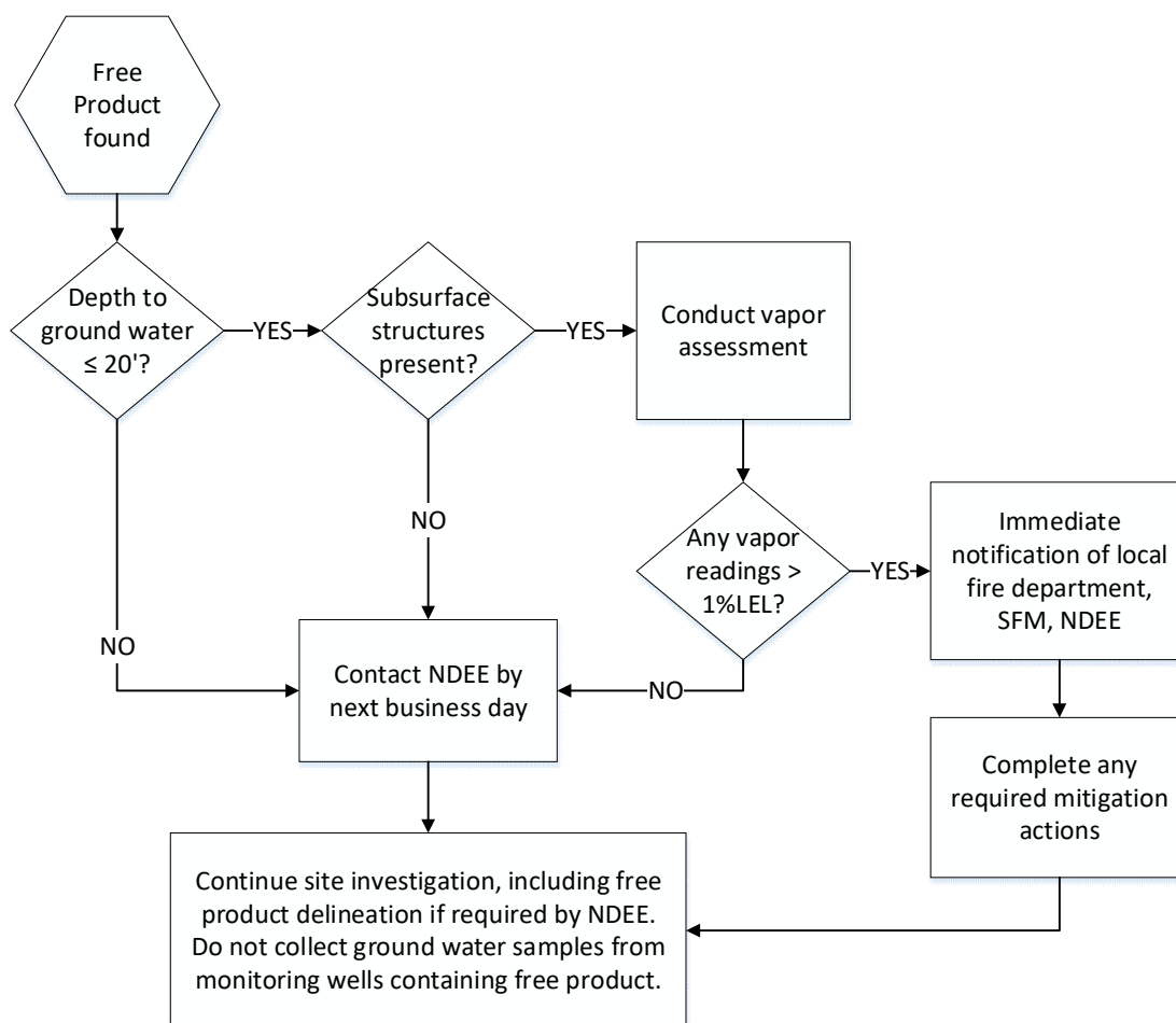
Figure 4-1. Free Product Response Process
