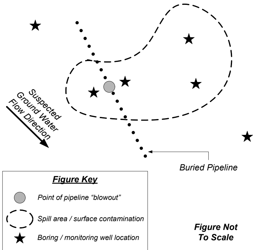
Figure 3-1e. Generalized high-volume pipeline "blowout" resulting in large volume petroleum release with an area of contaminated surface soils. This release would be ineligible for Title 200 reimbursement. The actual number of source area borings/monitoring wells (denoted by the stars within the spill area) will vary based on the size of the spill area and consultation with the Department. For such a surface release, low-lying areas where product may pool are likely candidates for boring placement. Upgradient and downgradient monitoring wells should be included.
