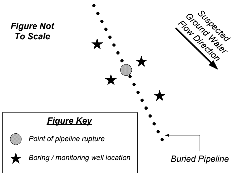
Figure 3-1f. Generalized high-volume pipeline release with limited or no contaminated surface soils. The immediate vicinity of the point of pipeline rupture would be considered the source area. A minimum of four borings/monitoring wells would be placed around the point of release, including upgradient, downgradient, and both cross-gradient locations. This release would be ineligible for Title 200 reimbursement.
