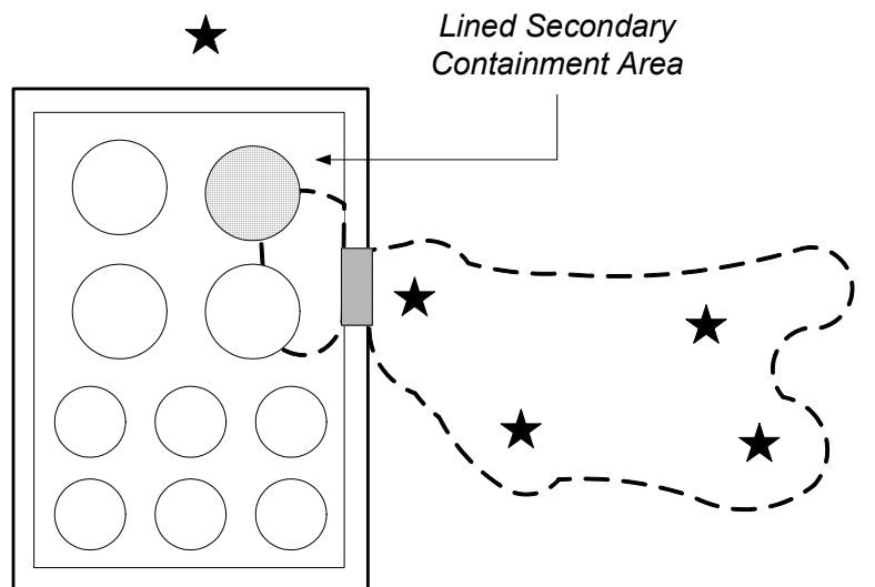
Figure 3-1c. Generalized AST bulk facility with lined secondary containment. To maintain the integrity of the liner, borings are generally not required within the secondary containment area. The actual number of source area borings/monitoring wells (denoted by the stars within the spill area) will vary based on the size of the spill area and consultation with the Department. For such a surface release, low-lying areas where product may pool are likely candidates for boring placement. Note the placement of an upgradient and down gradient monitoring well.
