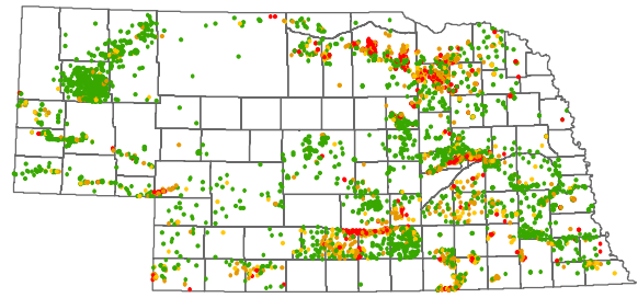
2011 (4118 wells, 4616 analyses)
