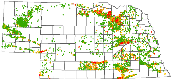
2012 (4744 wells, 5440 analyses)
