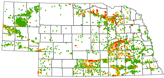
2010 (4492 wells, 5045 analyses)
