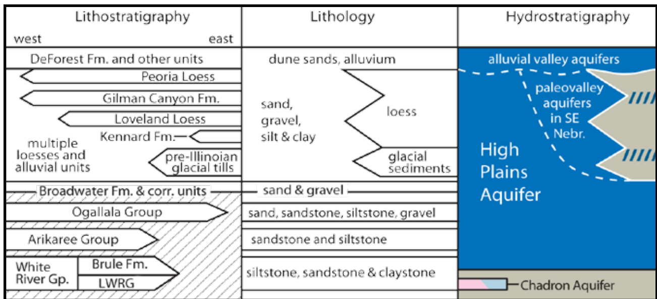
Figure 5. Excerpts from the generalized geologic and hydrostratigraphic framework of Nebraska. (Source: University of NE, Conservation and Survey Division, 2013)
