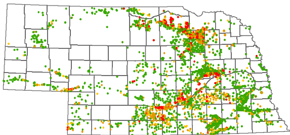
2014 (4339 wells, 4793 analyses)
