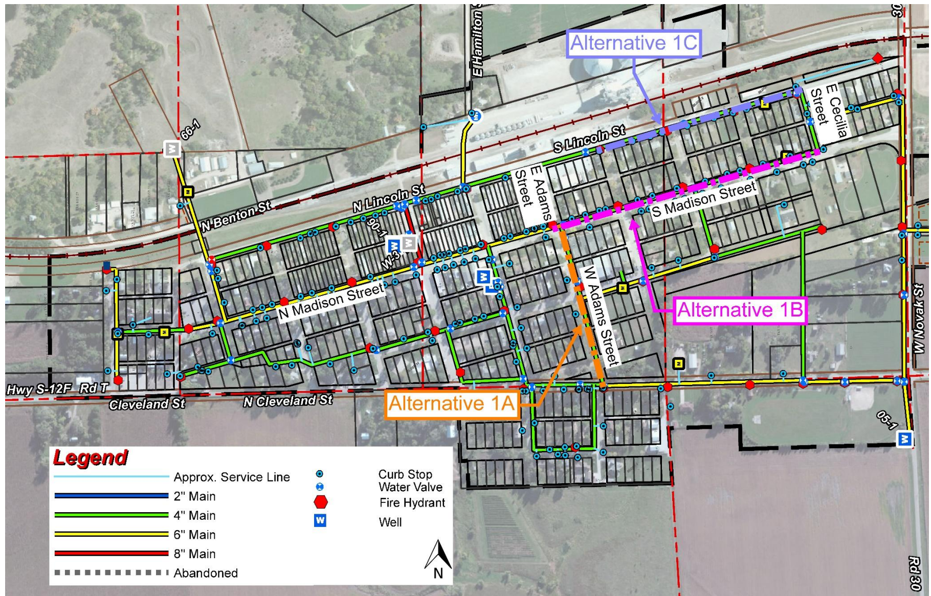
Figure 1: Map of Brainard's Distribution System Showing Locations of Water Main Replacements (Alternatives 1A, 1B, and 1C)
