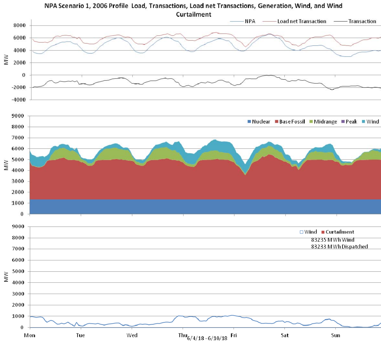
Figure 23: Nebraska 10% wind Penetration, 2006 Profile week of 6/4/2018
