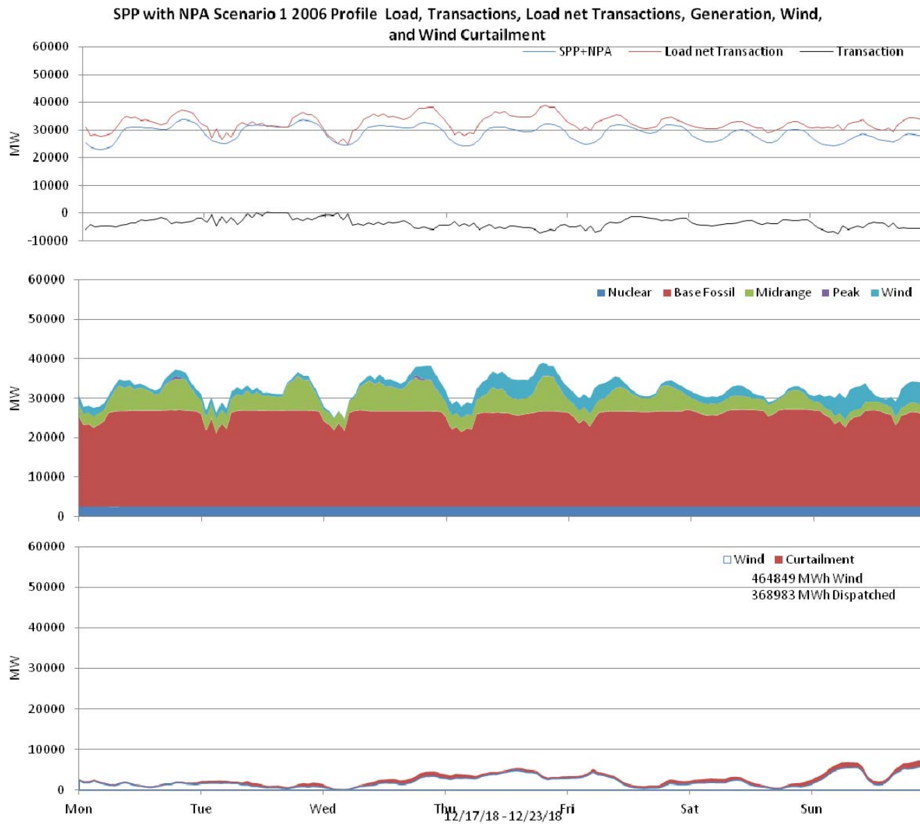
Figure 103: SPP 10% wind Penetration, 2006 Profile week of 12/17/2018
