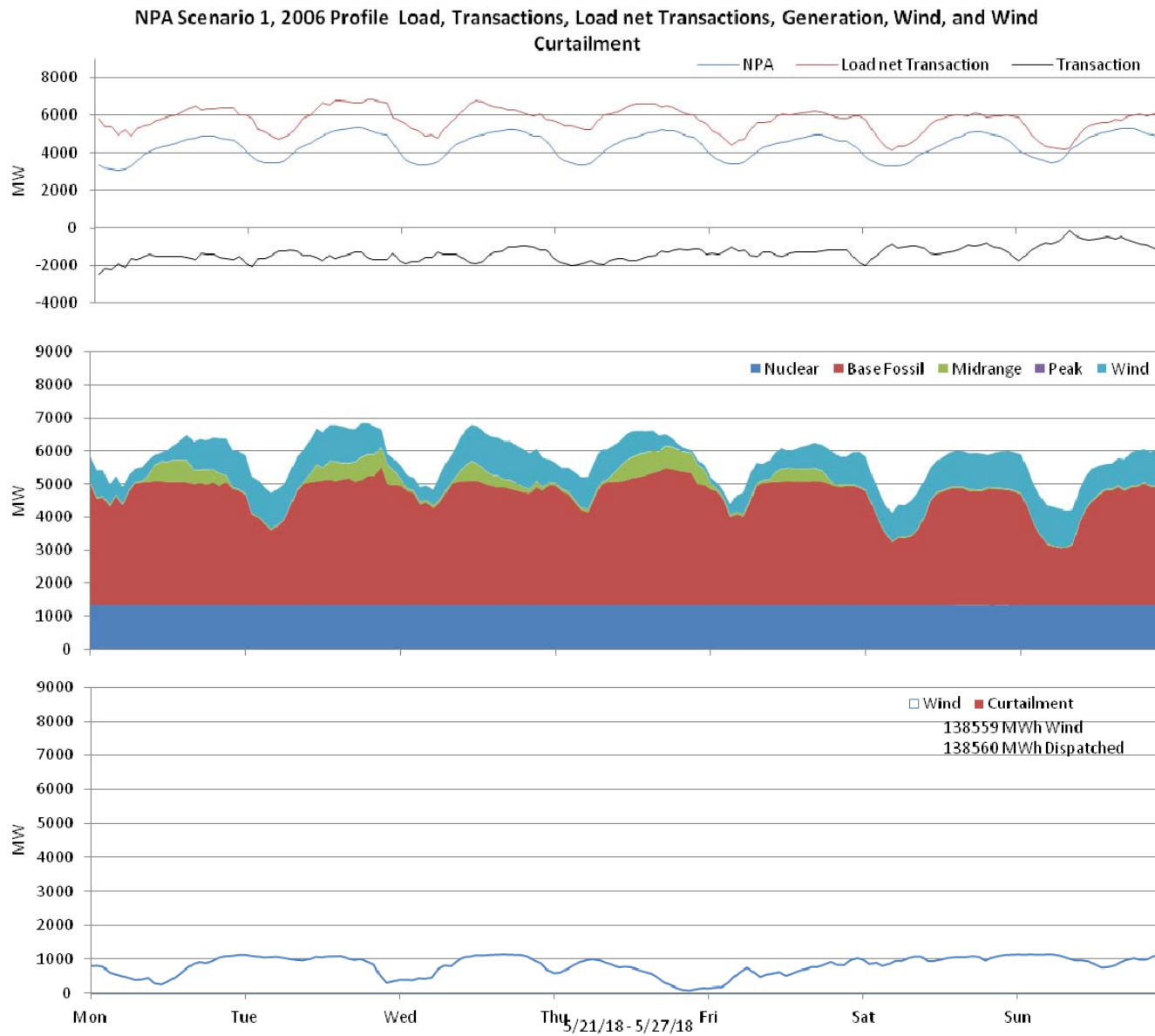
Figure 21: Nebraska 10% wind Penetration, 2006 Profile week of 5/21/2018
