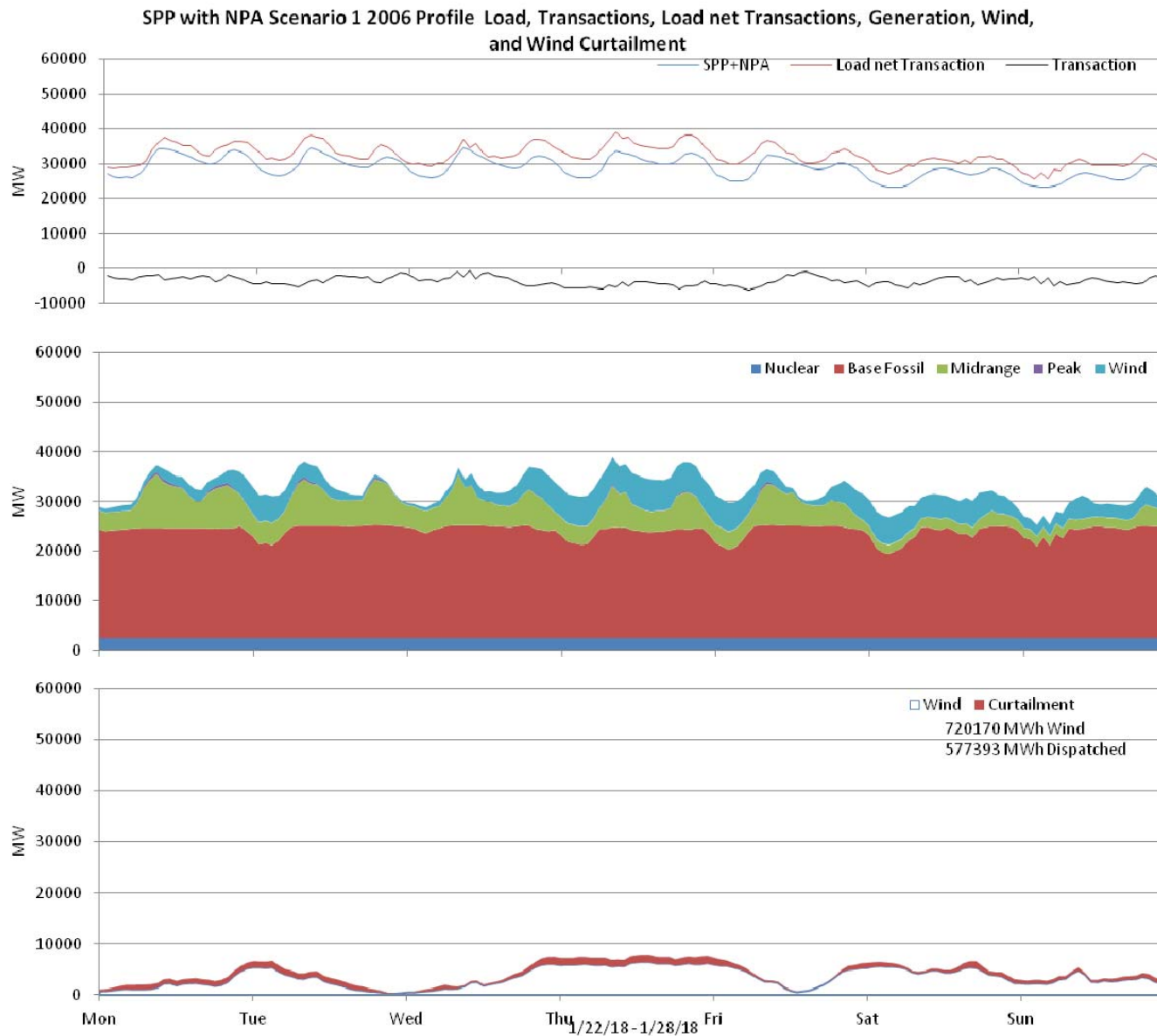
Figure 56: SPP 10% wind Penetration, 2006 Profile week of 1/22/2018
