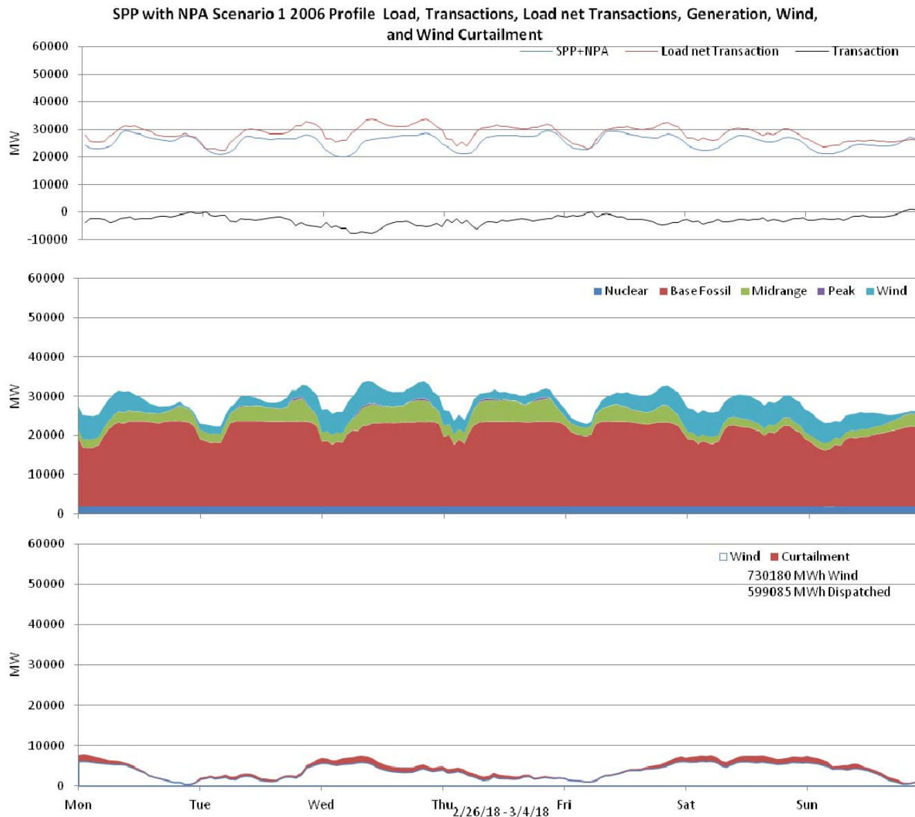
Figure 61: SPP 10% wind Penetration, 2006 Profile week of 2/26/2018
