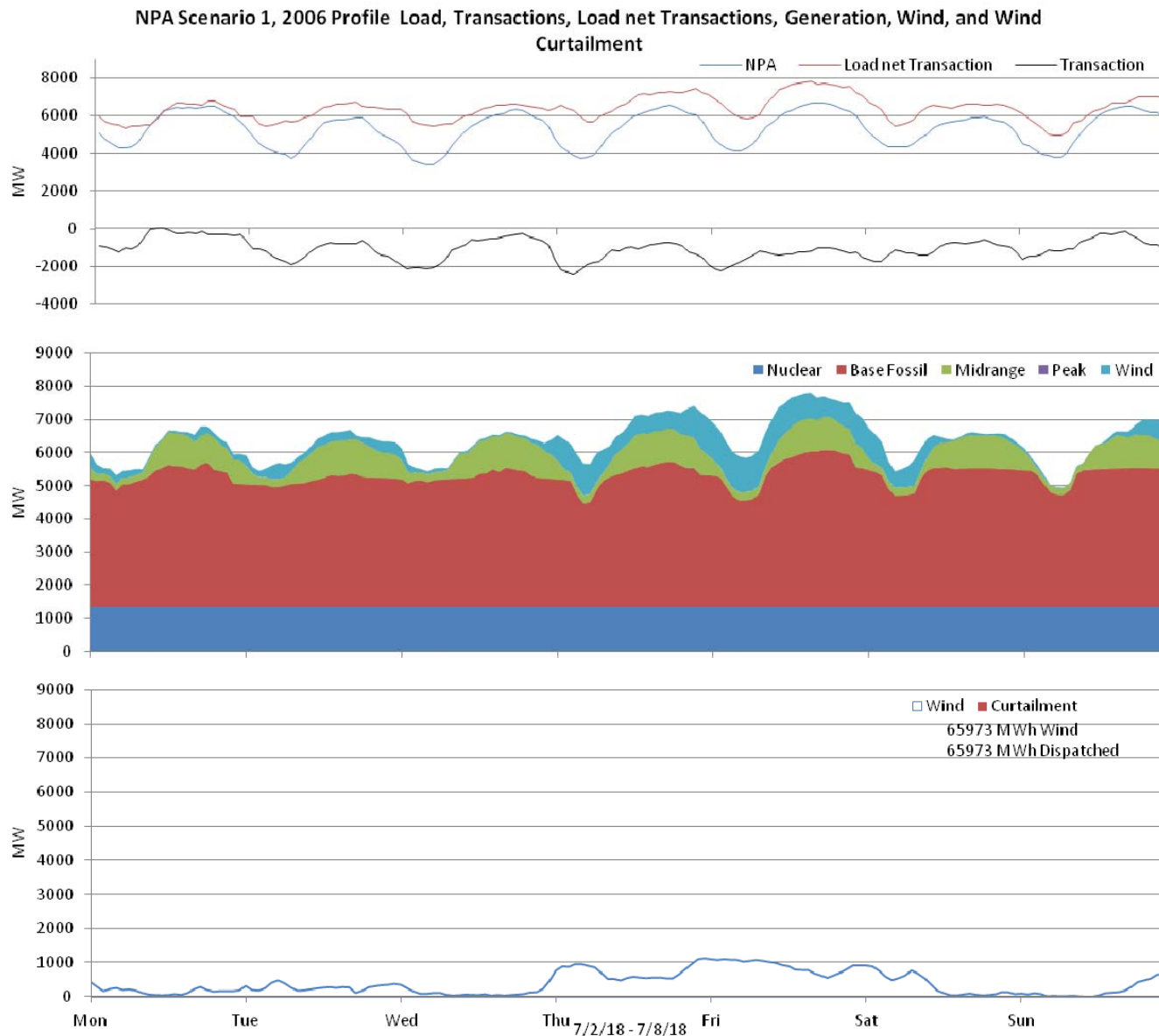
Figure 27: Nebraska 10% wind Penetration, 2006 Profile week of 7/2/2018
