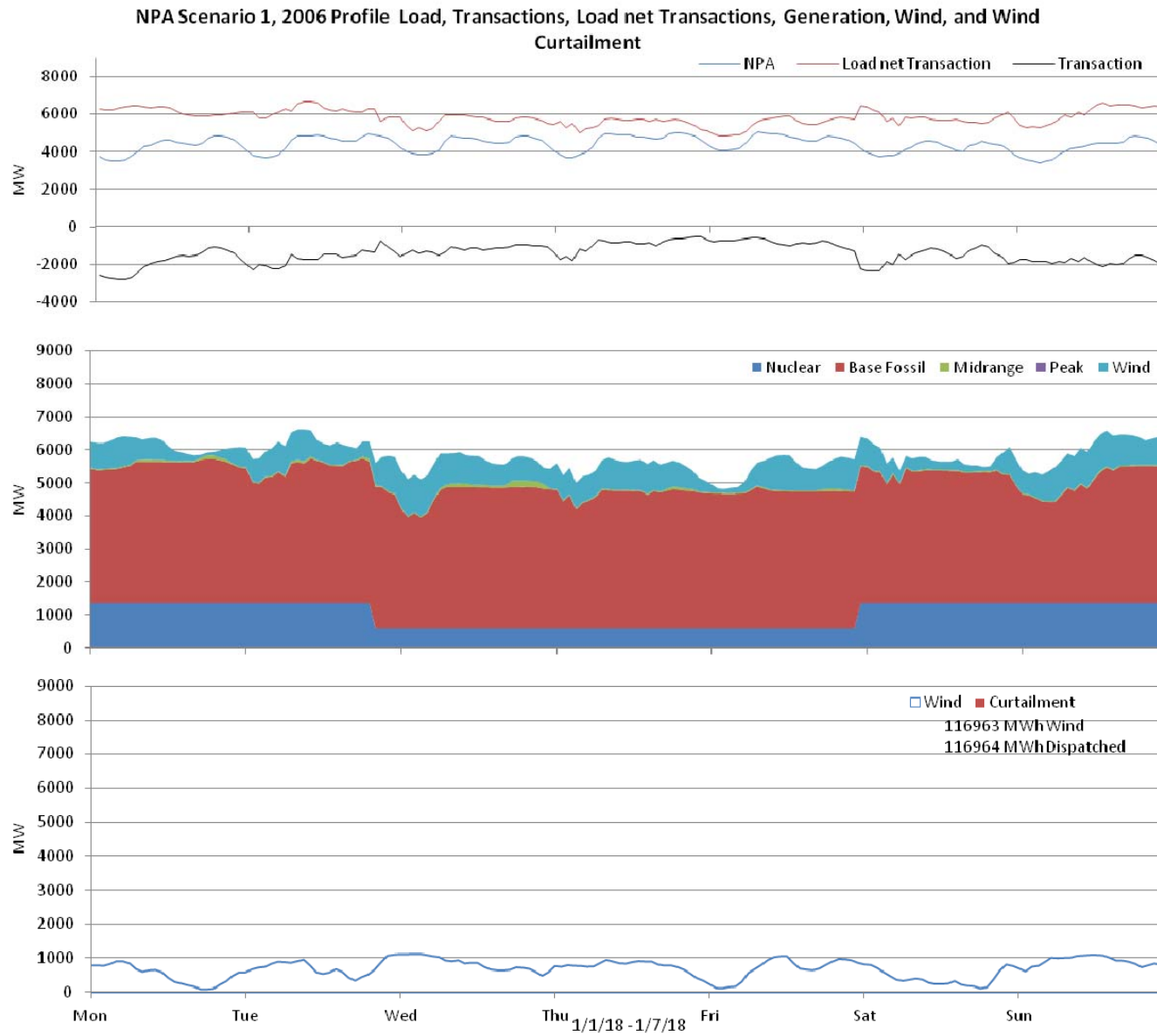
Figure 1: Nebraska 10% wind Penetration, 2006 Profile week of 1/1/2018
