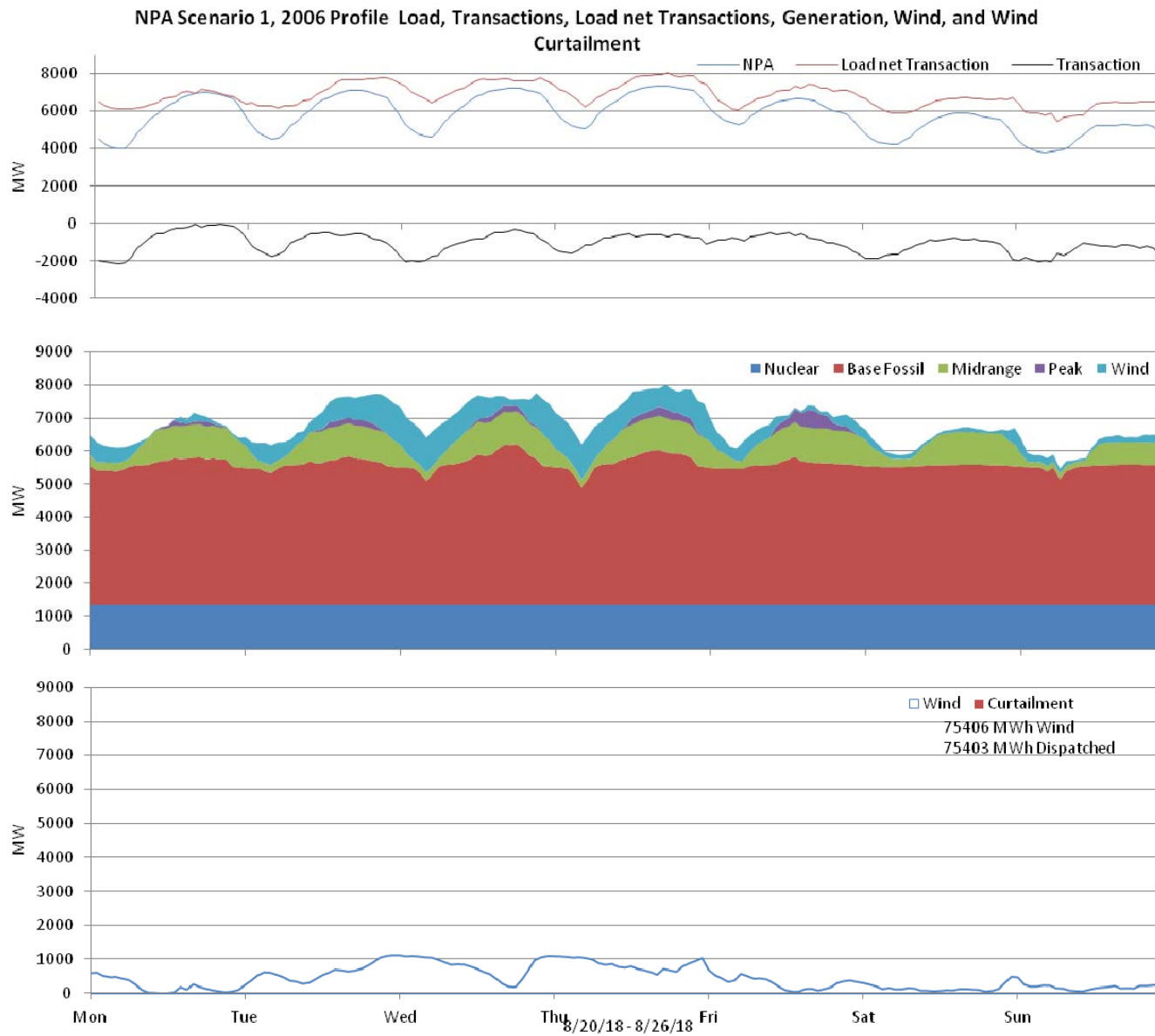
Figure 34: Nebraska 10% wind Penetration, 2006 Profile week of 8/20/2018
