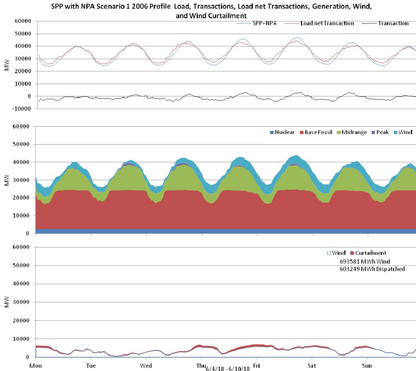
Figure 75: SPP 10% wind Penetration, 2006 Profile week of 6/4/2018
