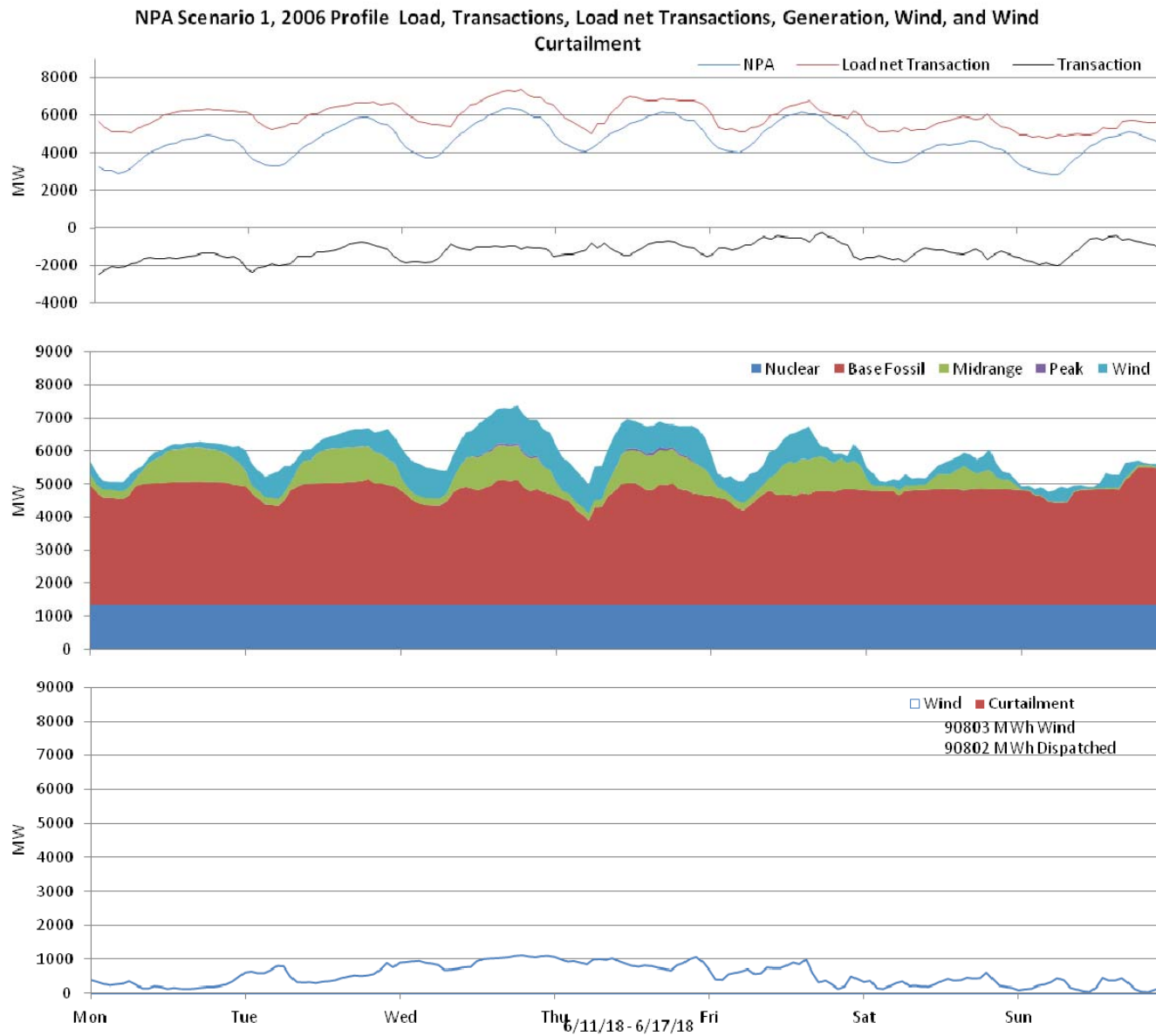
Figure 24: Nebraska 10% wind Penetration, 2006 Profile week of 6/11/2018
