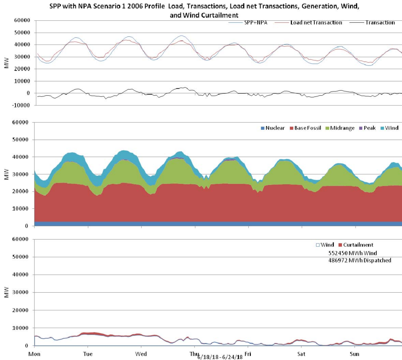
Figure 77: SPP 10% wind Penetration, 2006 Profile week of 6/18/2018
