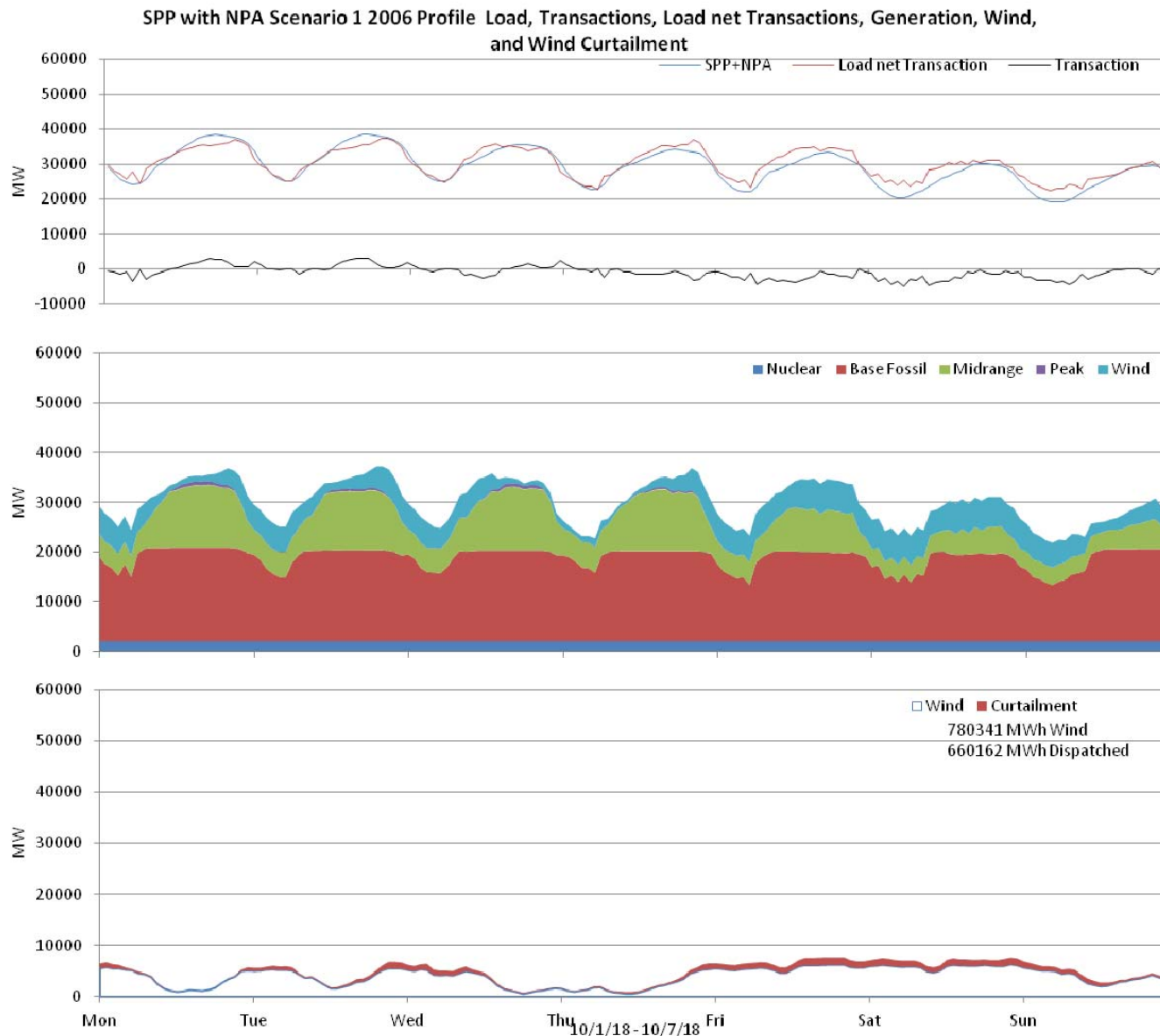
Figure 92: SPP 10% wind Penetration, 2006 Profile week of 10/1/2018
