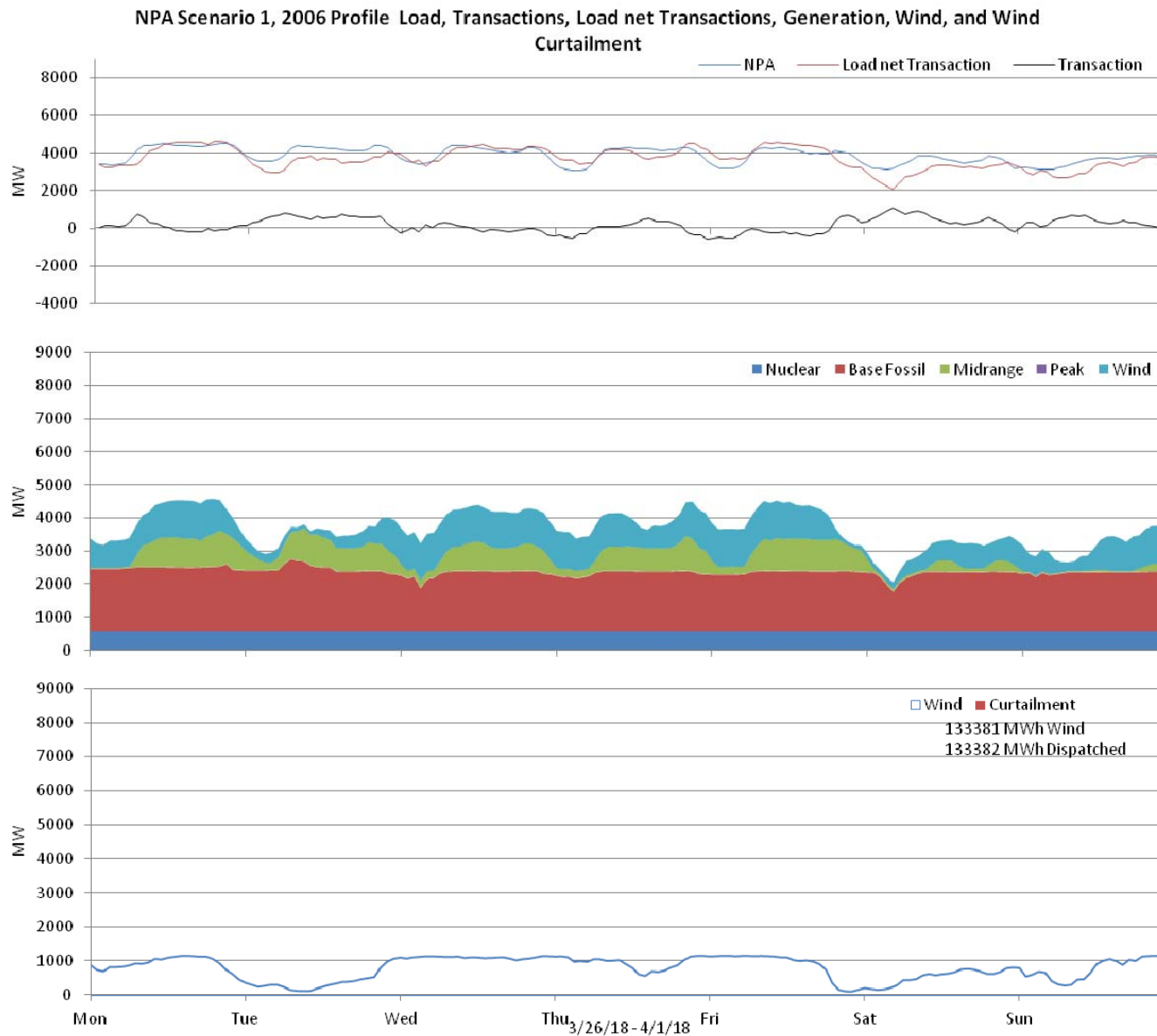
Figure 13: Nebraska 10% wind Penetration, 2006 Profile week of 3/26/2018
