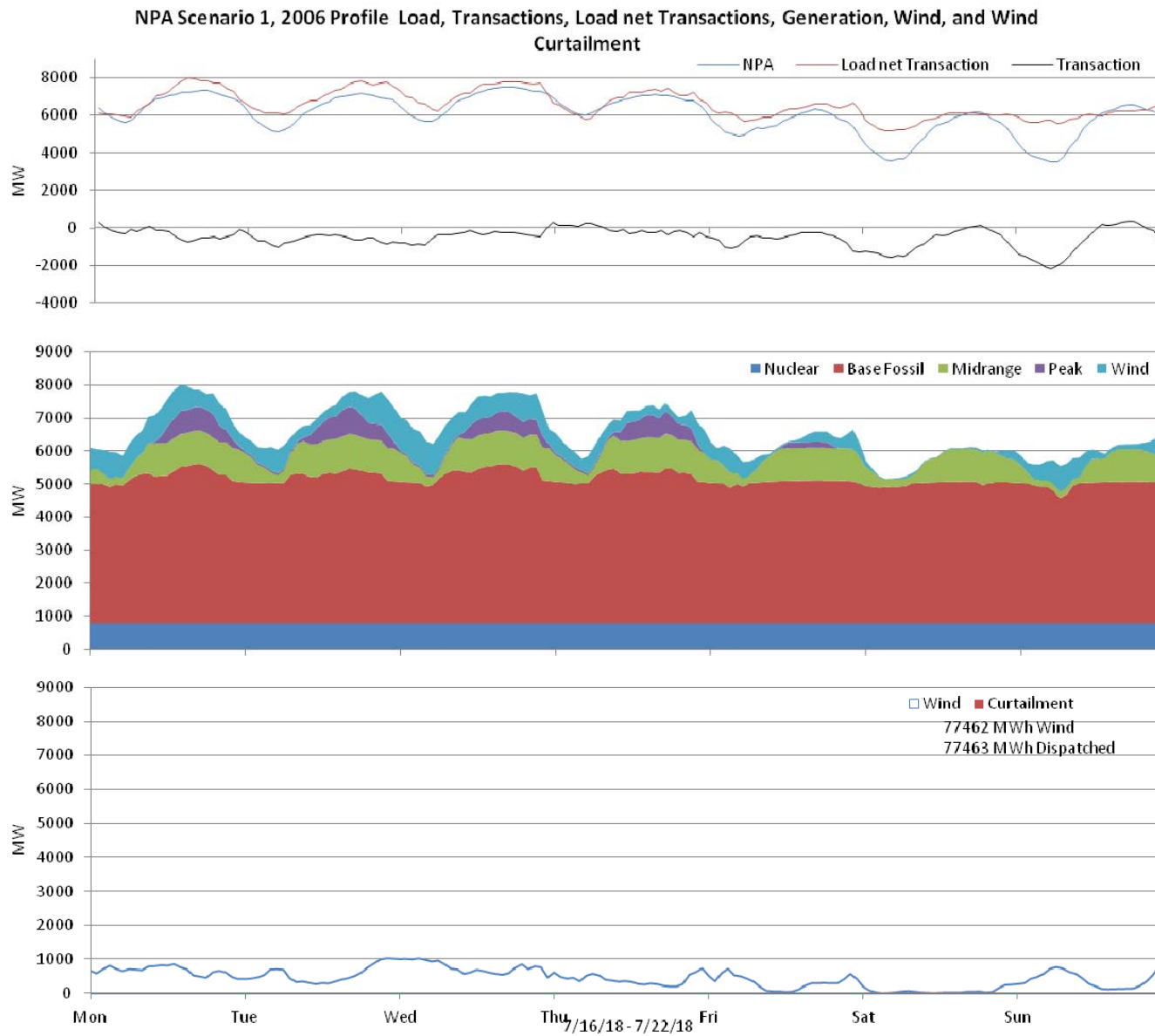
Figure 29: Nebraska 10% wind Penetration, 2006 Profile week of 7/16/2018
