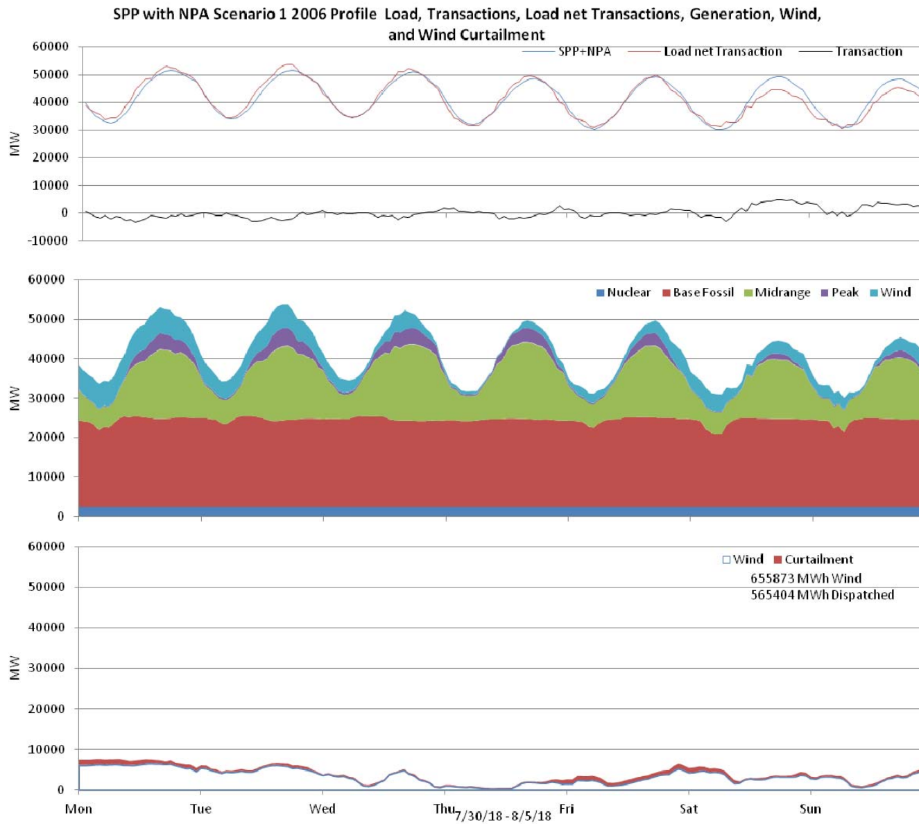
Figure 83: SPP 10% wind Penetration, 2006 Profile week of 7/30/2018
