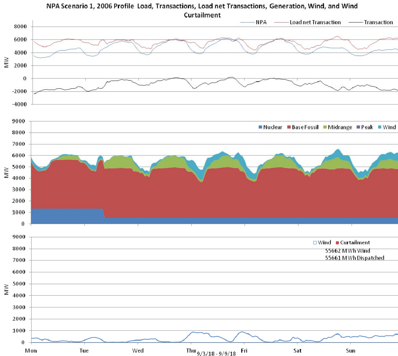
Figure 36: Nebraska 10% wind Penetration, 2006 Profile week of 9/3/2018
