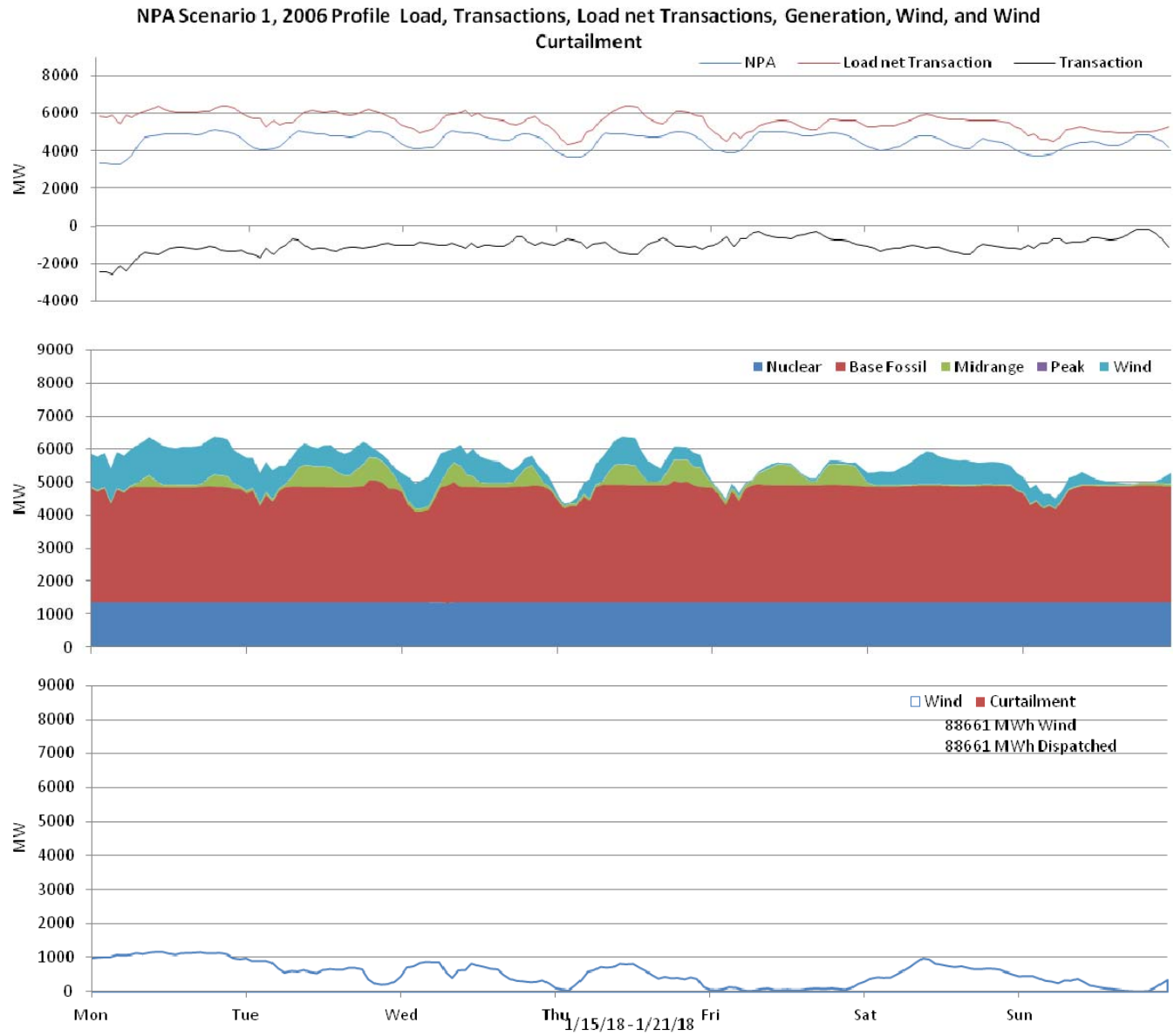
Figure 3: Nebraska 10% wind Penetration, 2006 Profile week of 1/15/2018
