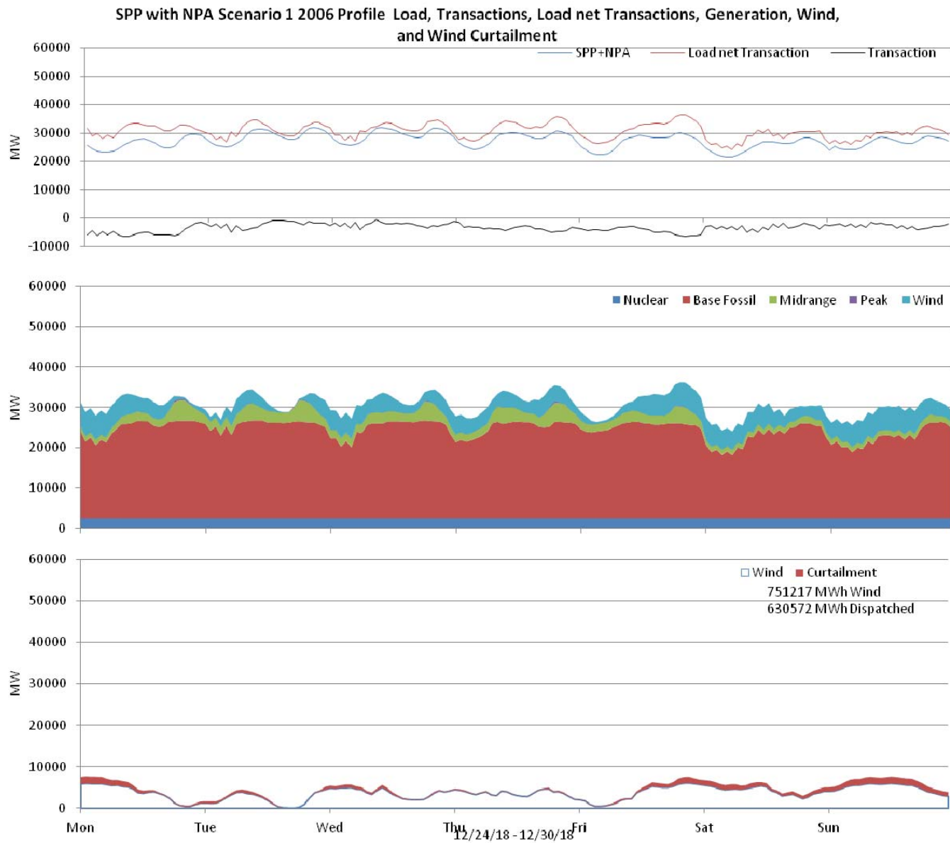
Figure 104: SPP 10% wind Penetration, 2006 Profile week of 12/24/2018
