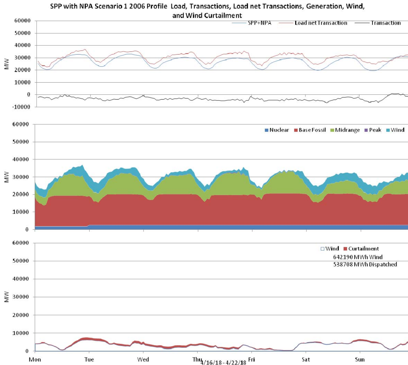
Figure 68: SPP 10% wind Penetration, 2006 Profile week of 4/16/2018
