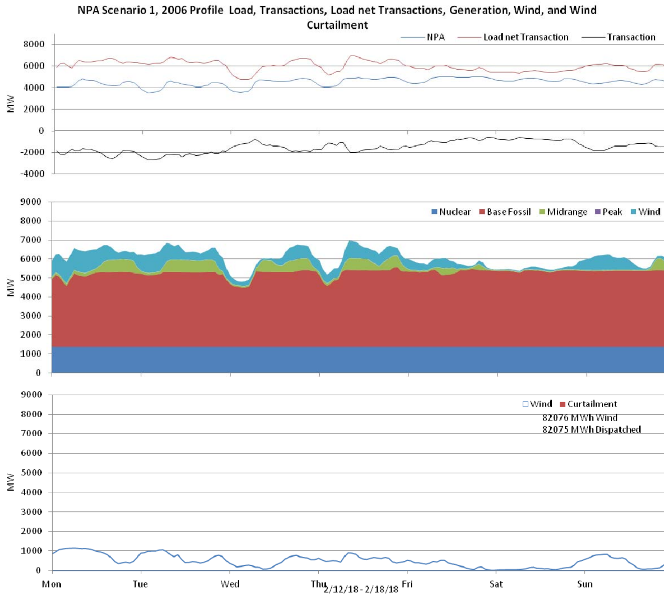
Figure 7: Nebraska 10% wind Penetration, 2006 Profile week of 2/12/2018
