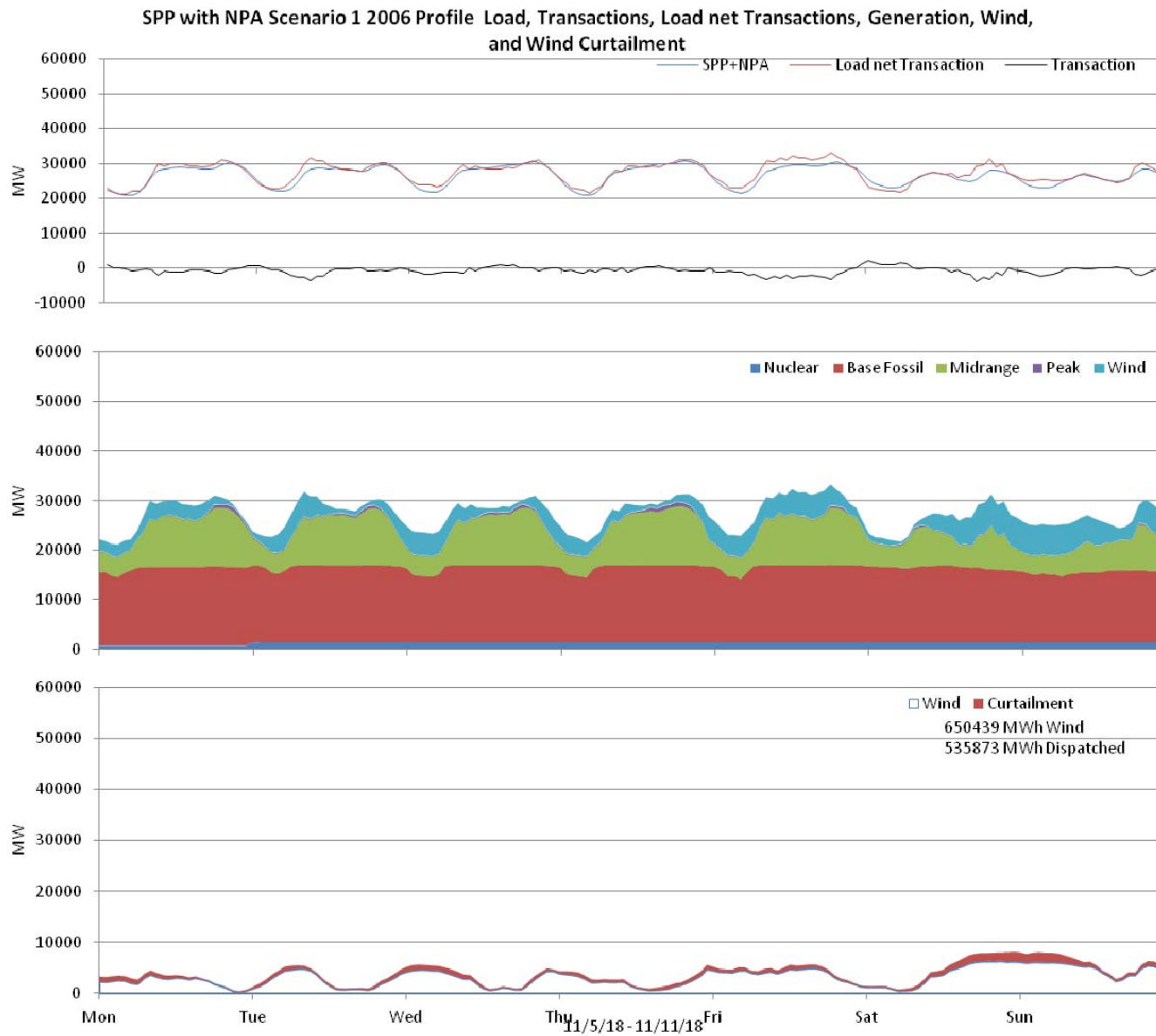
Figure 97: SPP 10% wind Penetration, 2006 Profile week of 11/5/2018
