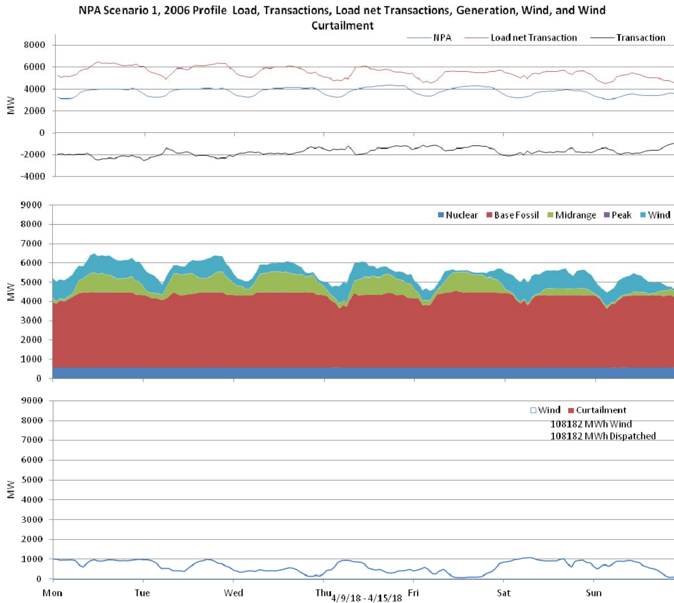
Figure 15: Nebraska 10% wind Penetration, 2006 Profile week of 4/9/2018
