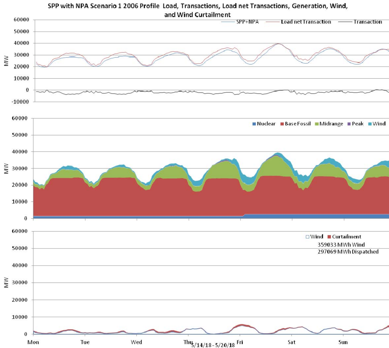
Figure 72: SPP 10% wind Penetration, 2006 Profile week of 5/14/2018
