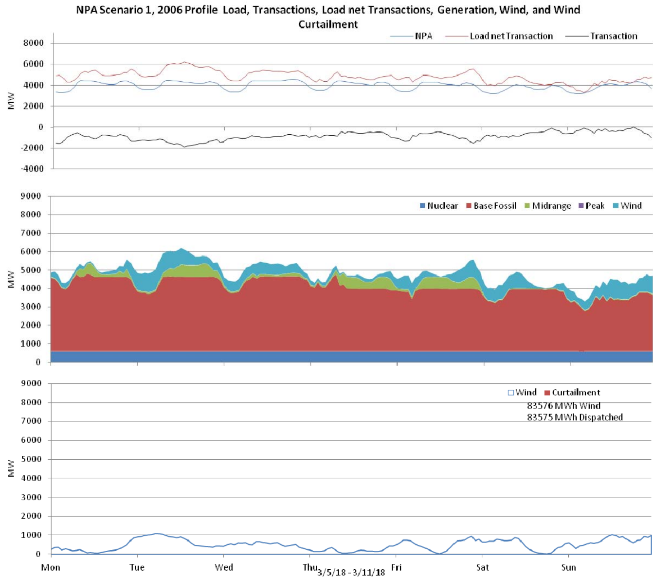
Figure 10: Nebraska 10% wind Penetration, 2006 Profile week of 3/5/2018
