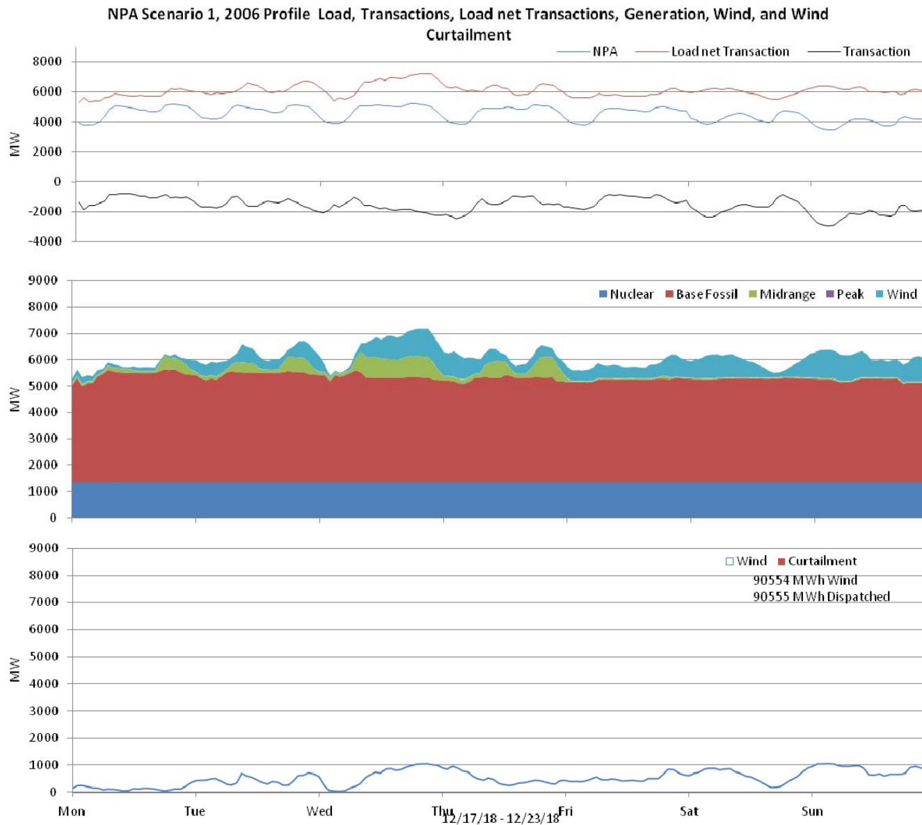
Figure 51: Nebraska 10% wind Penetration, 2006 Profile week of 12/17/2018
