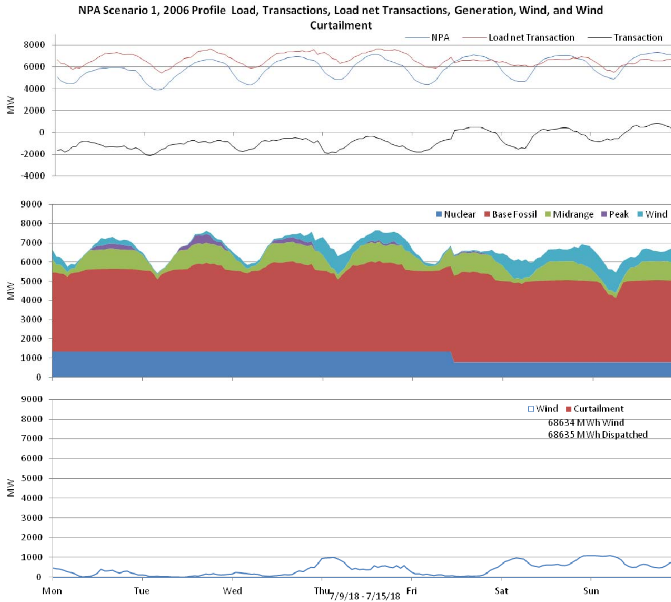
Figure 28: Nebraska 10% wind Penetration, 2006 Profile week of 7/9/2018
