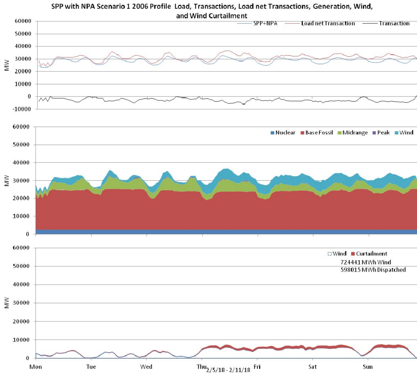
Figure 58: SPP 10% wind Penetration, 2006 Profile week of 2/5/2018
