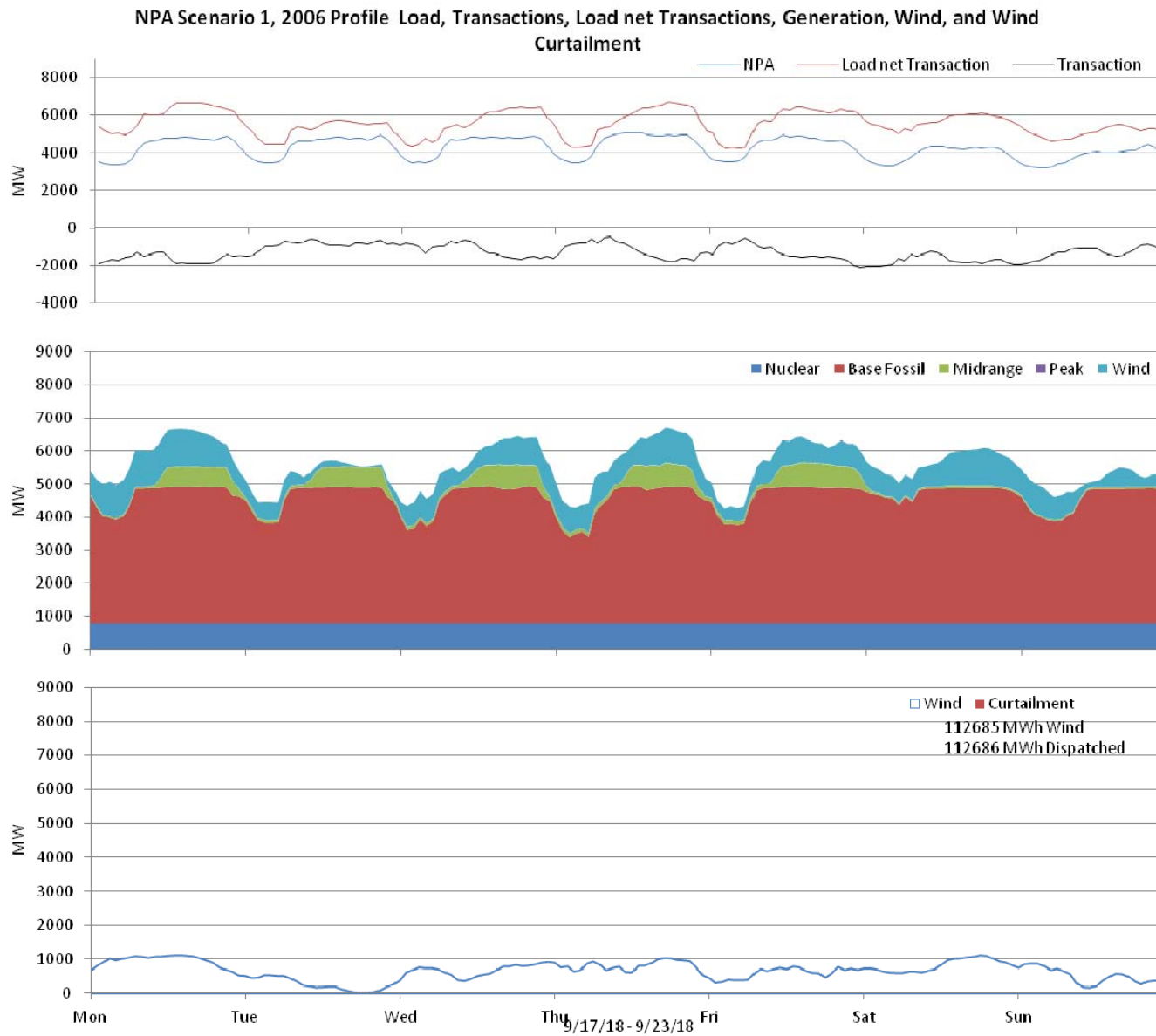
Figure 38: Nebraska 10% wind Penetration, 2006 Profile week of 9/17/2018
