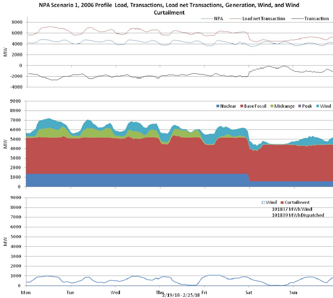
Figure 8: Nebraska 10% wind Penetration, 2006 Profile week of 2/19/2018
