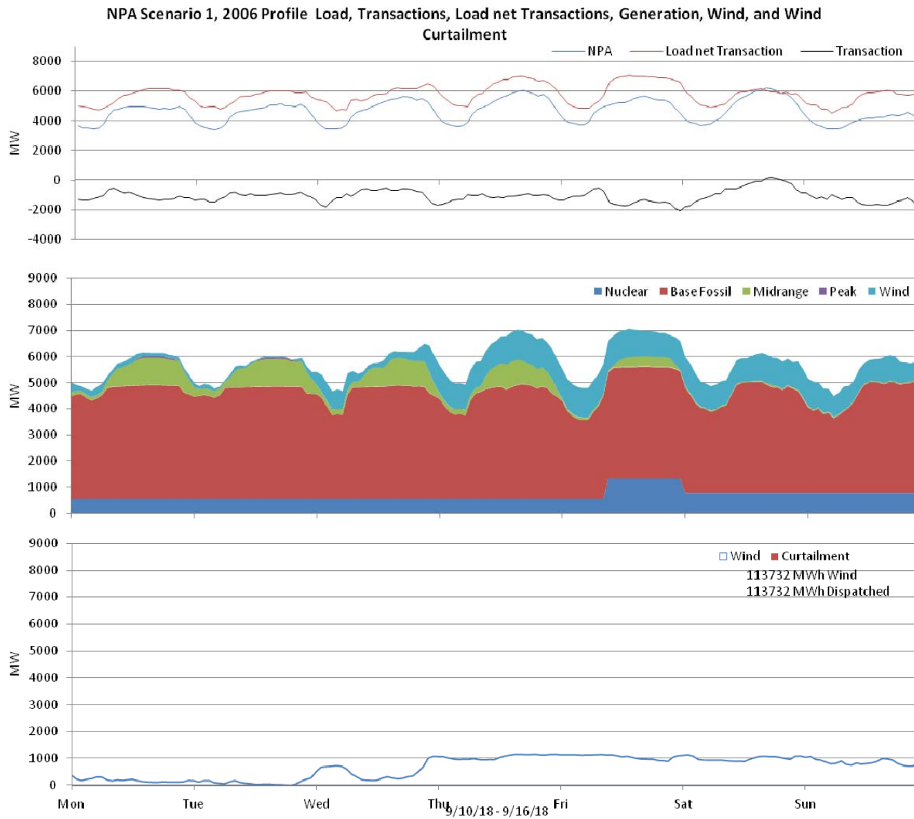
Figure 37: Nebraska 10% wind Penetration, 2006 Profile week of 9/10/2018
