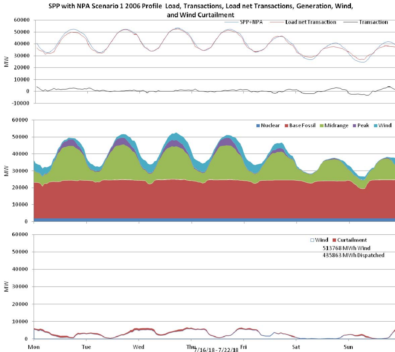
Figure 81: SPP 10% wind Penetration, 2006 Profile week of 7/16/2018
