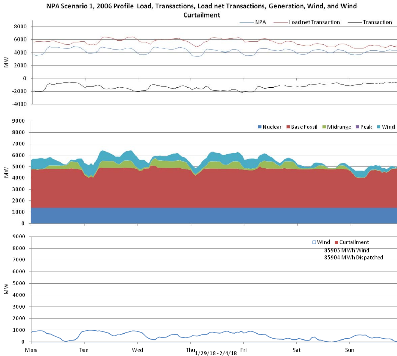
Figure 5: Nebraska 10% wind Penetration, 2006 Profile week of 1/29/2018
