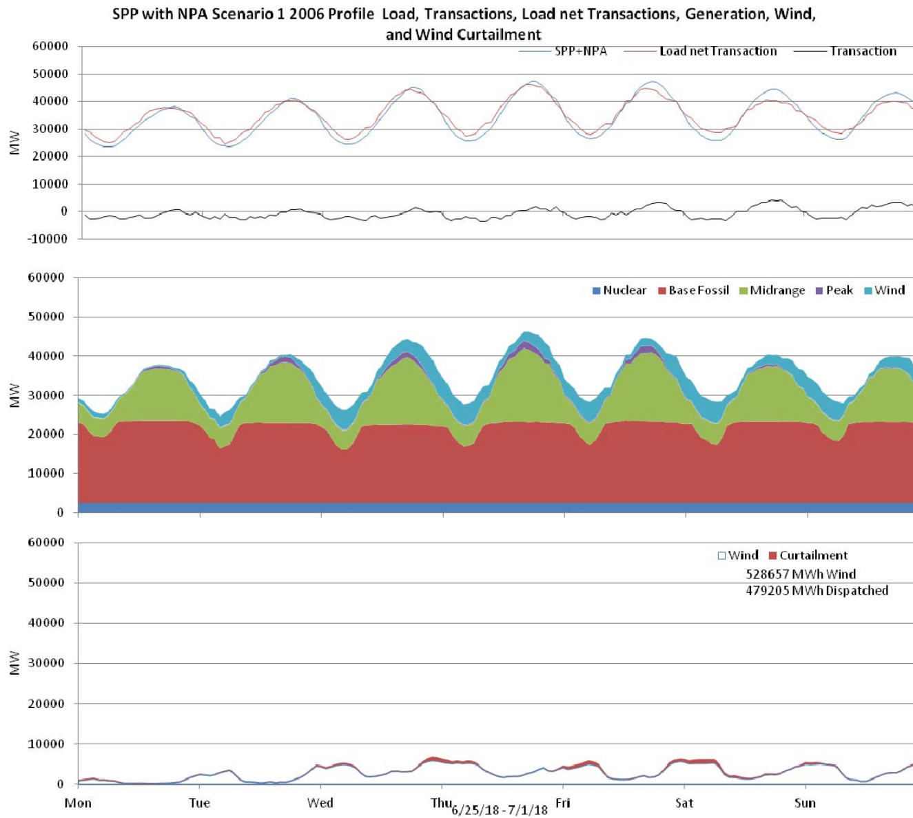
Figure 78: SPP 10% wind Penetration, 2006 Profile week of 6/25/2018
