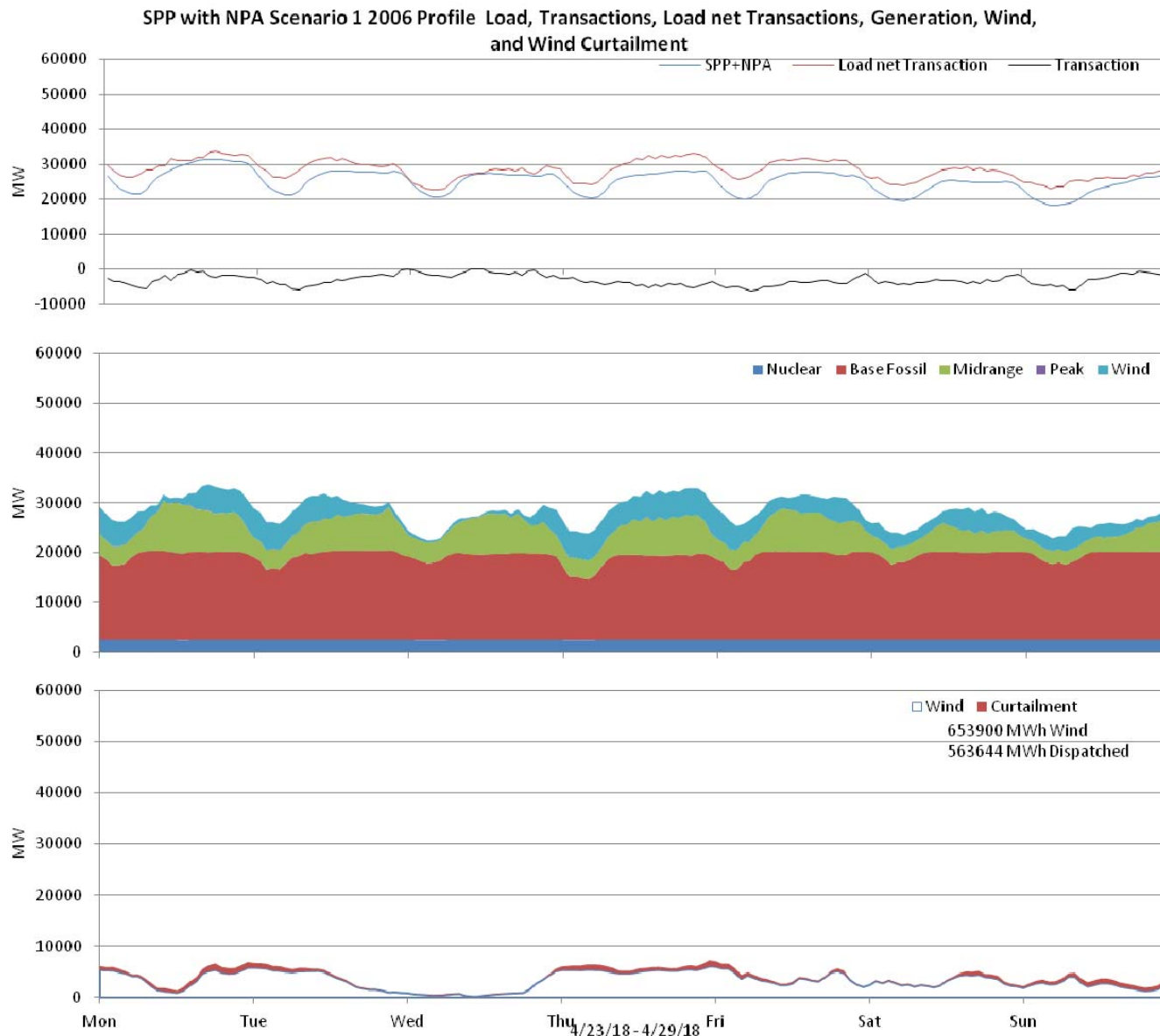
Figure 69: SPP 10% wind Penetration, 2006 Profile week of 4/23/2018
