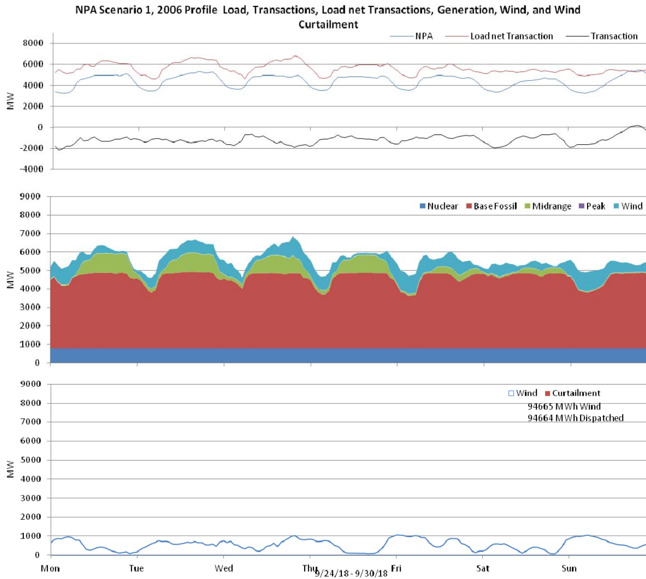
Figure 39: Nebraska 10% wind Penetration, 2006 Profile week of 9/24/2018
