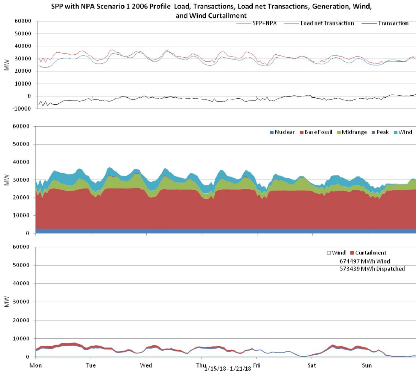
Figure 55: SPP 10% wind Penetration, 2006 Profile week of 1/15/2018
