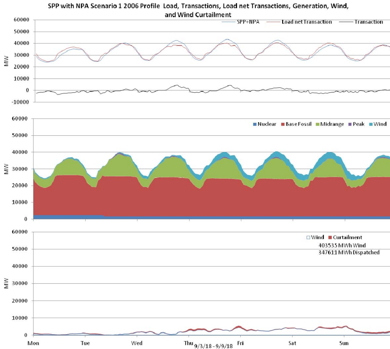
Figure 88: SPP 10% wind Penetration, 2006 Profile week of 9/3/2018
