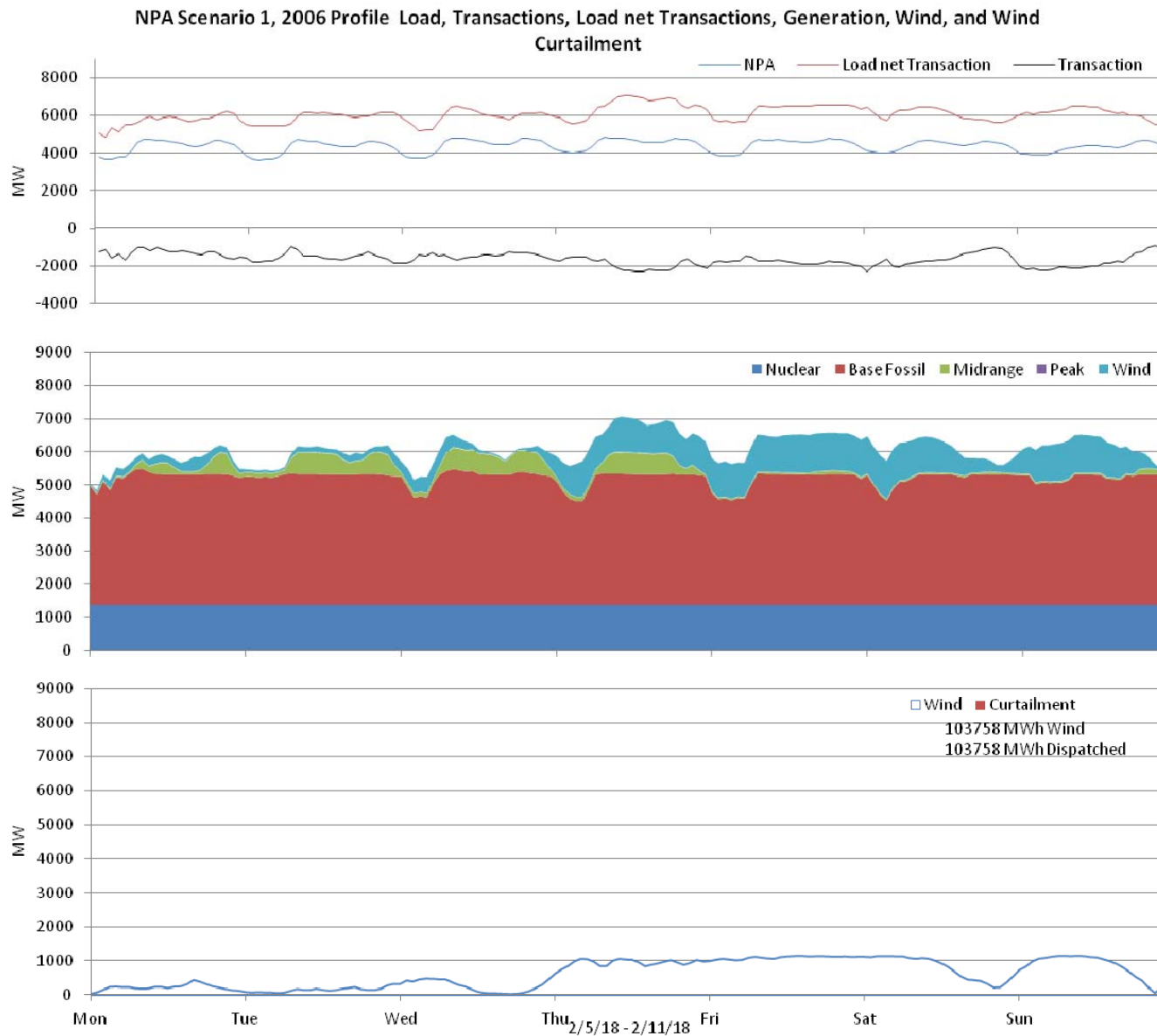
Figure 6: Nebraska 10% wind Penetration, 2006 Profile week of 2/5/2018
