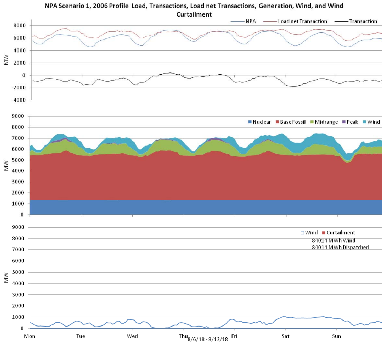
Figure 32: Nebraska 10% wind Penetration, 2006 Profile week of 8/6/2018
