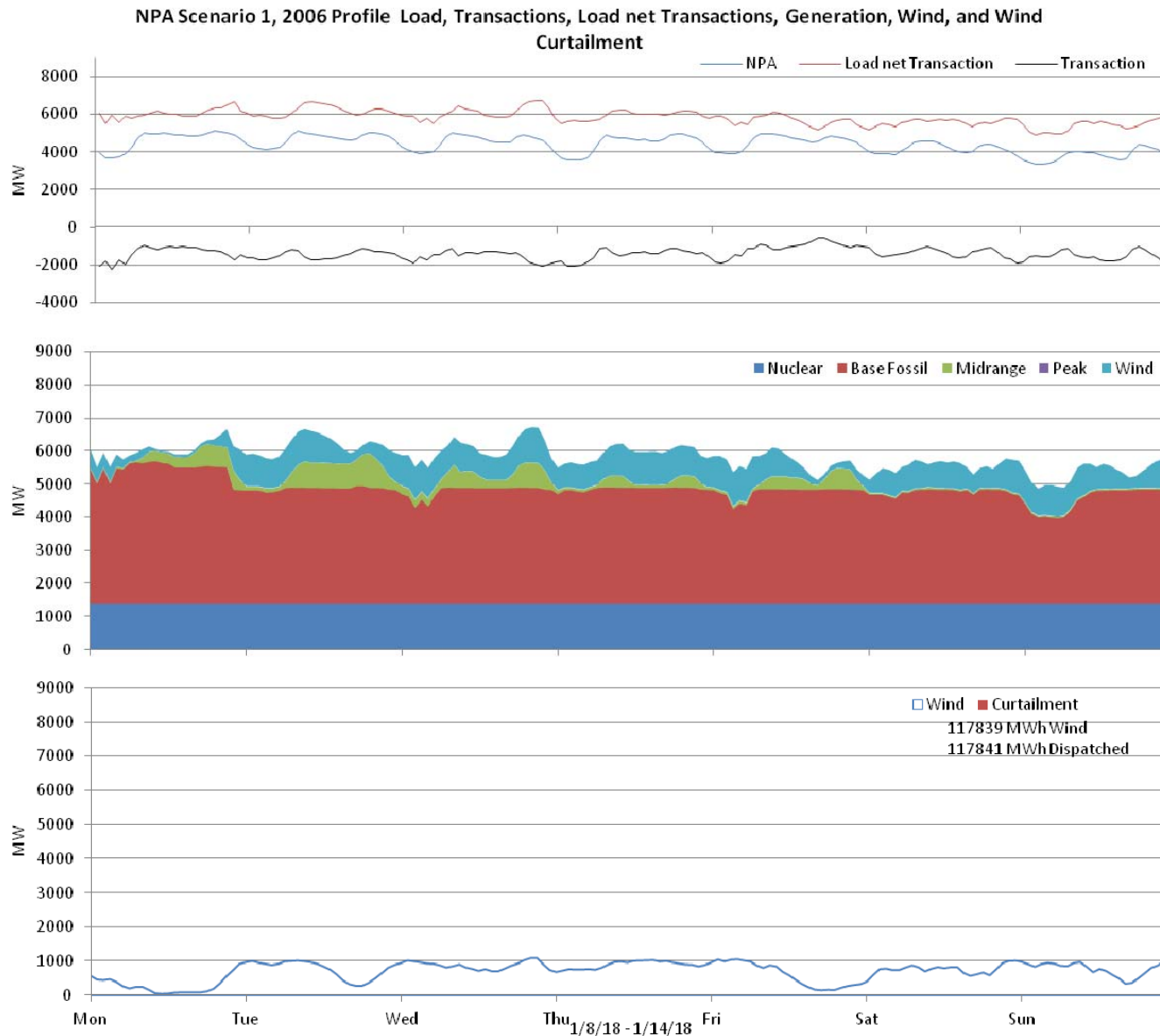
Figure 2: Nebraska 10% wind Penetration, 2006 Profile week of 1/8/2018
