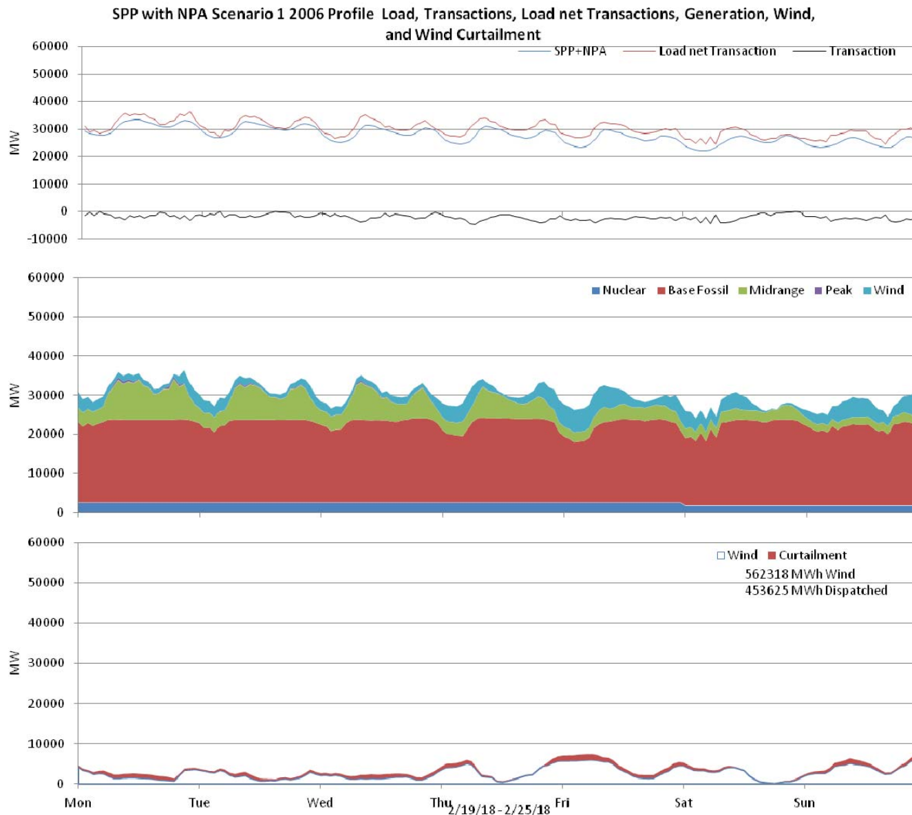
Figure 60: SPP 10% wind Penetration, 2006 Profile week of 2/19/2018
