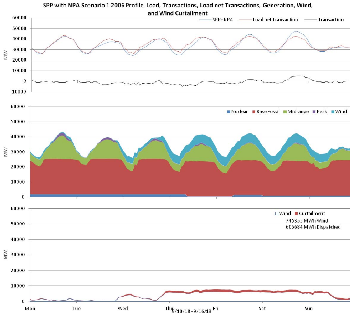
Figure 89: SPP 10% wind Penetration, 2006 Profile week of 9/10/2018
