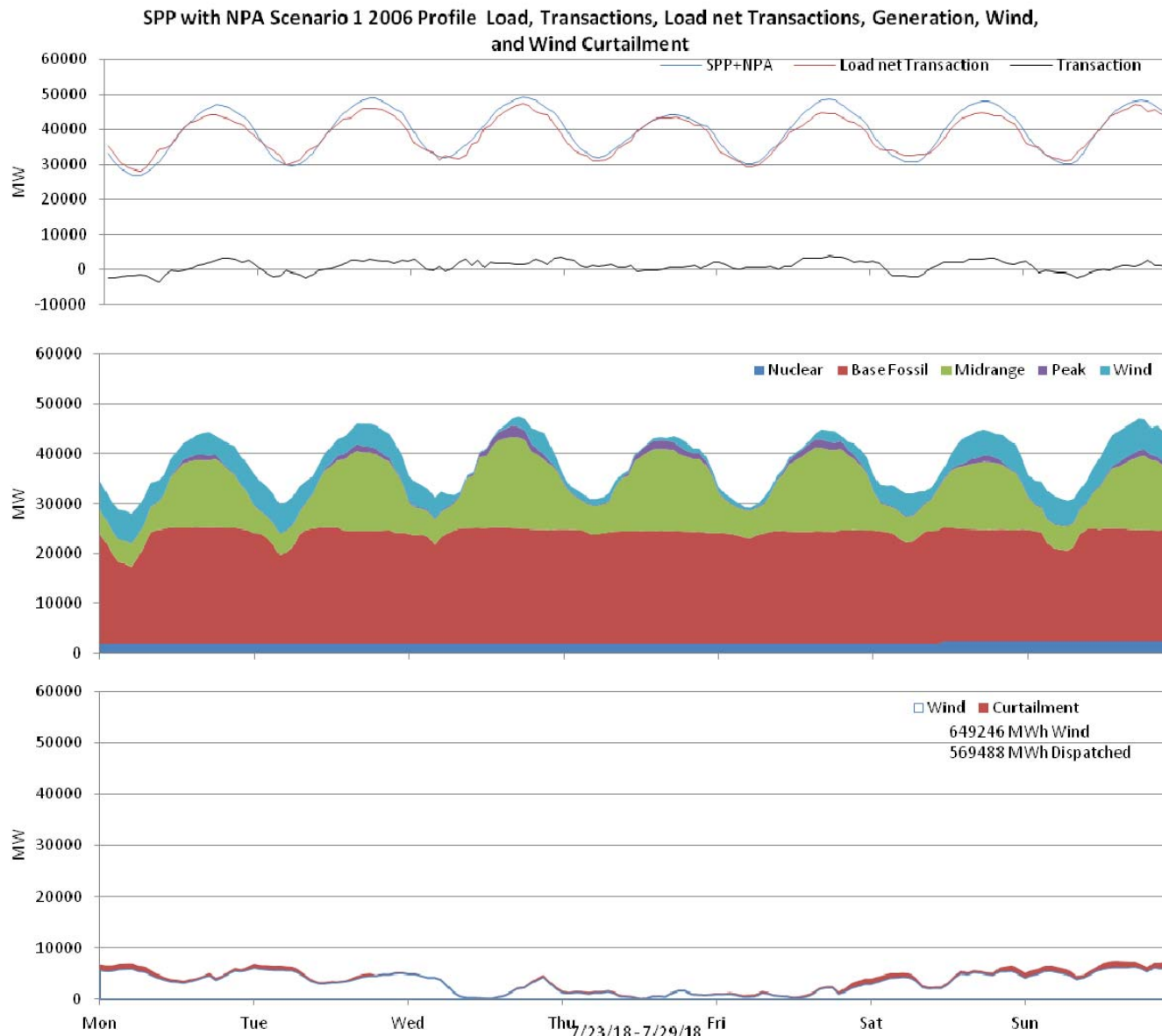
Figure 82: SPP 10% wind Penetration, 2006 Profile week of 7/23/2018
