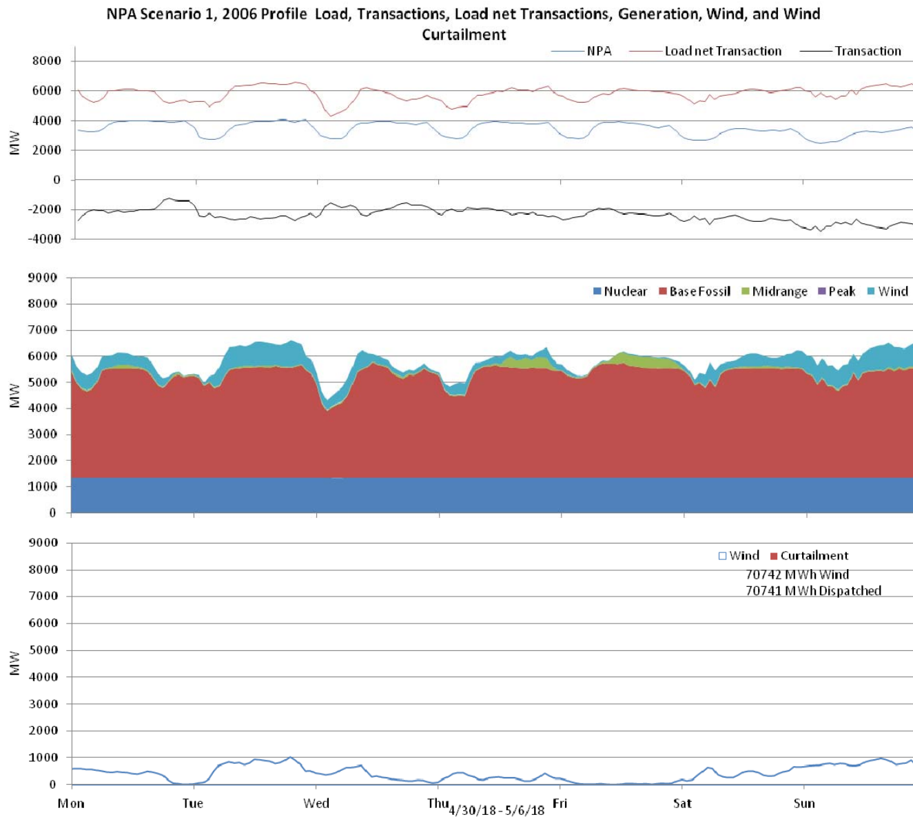
Figure 18: Nebraska 10% wind Penetration, 2006 Profile week of 4/30/2018
