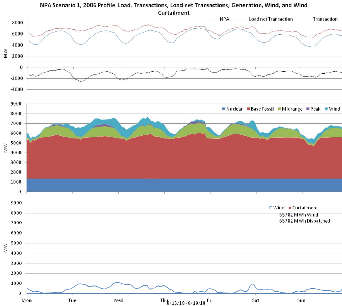
Figure 33: Nebraska 10% wind Penetration, 2006 Profile week of 8/13/2018
