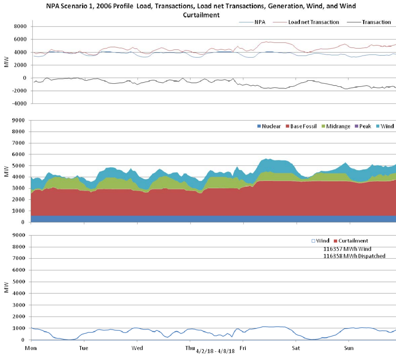
Figure 14: Nebraska 10% wind Penetration, 2006 Profile week of 4/2/2018
