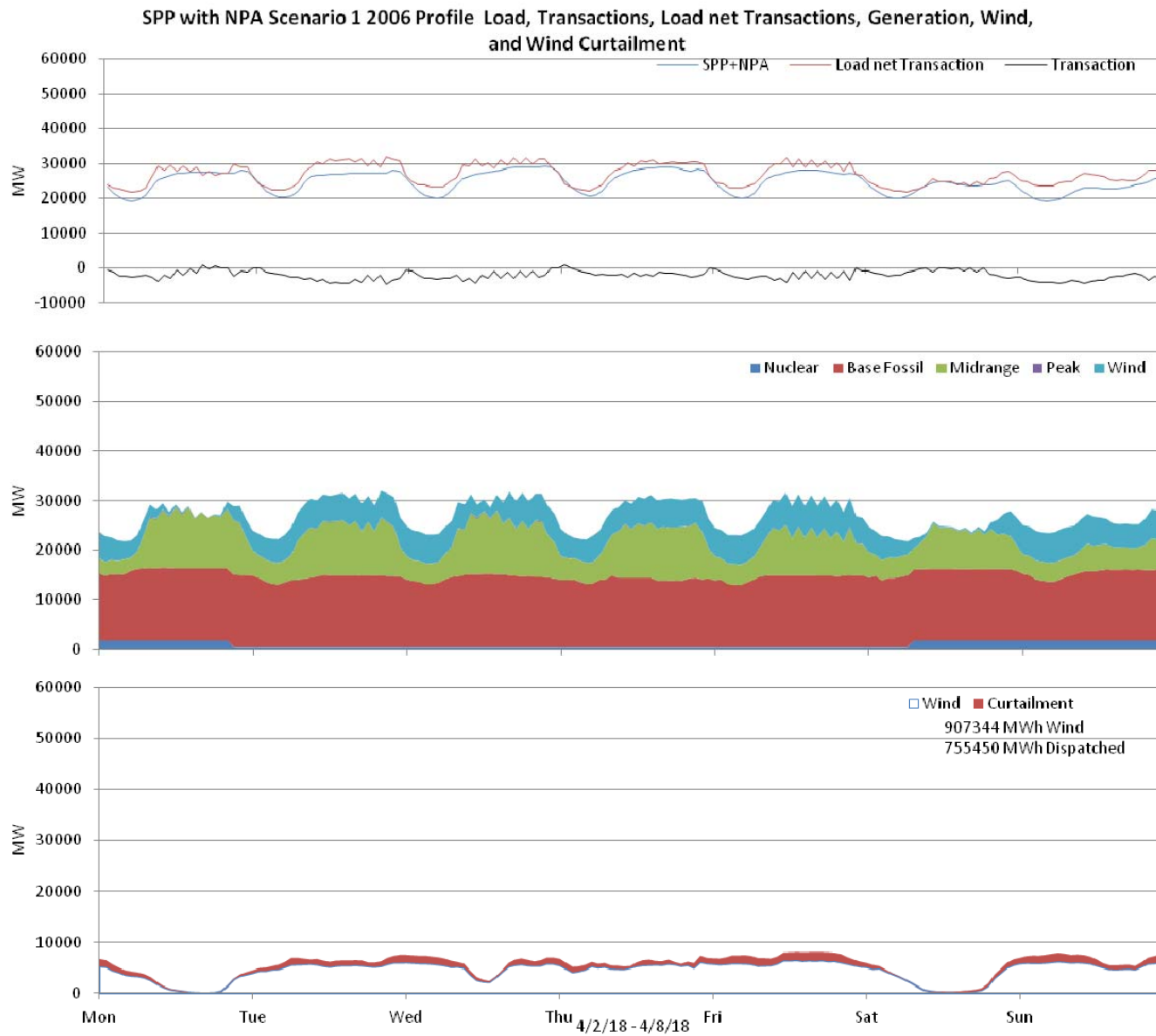
Figure 66: SPP 10% wind Penetration, 2006 Profile week of 4/2/2018
