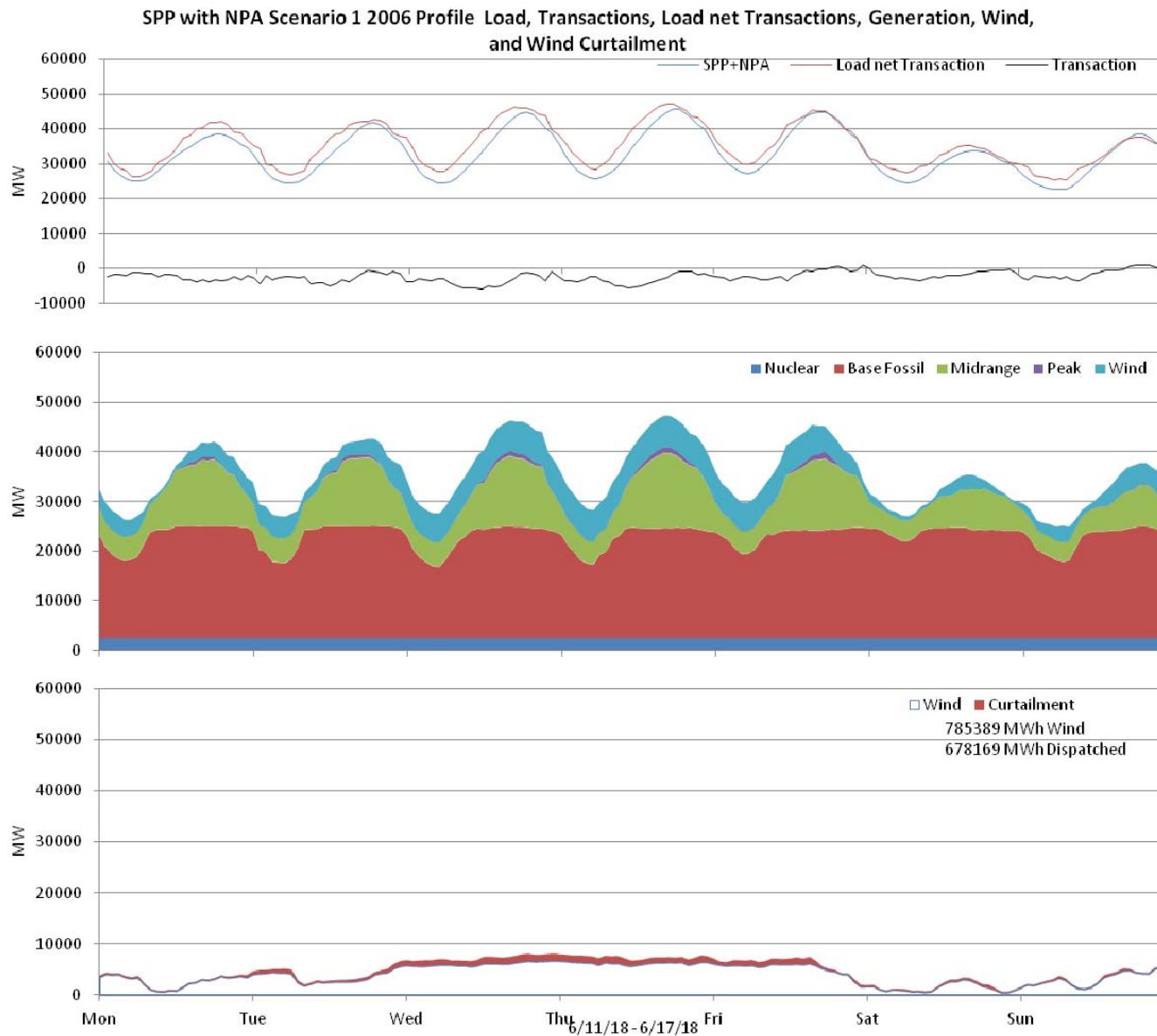
Figure 76: SPP 10% wind Penetration, 2006 Profile week of 6/11/2018
