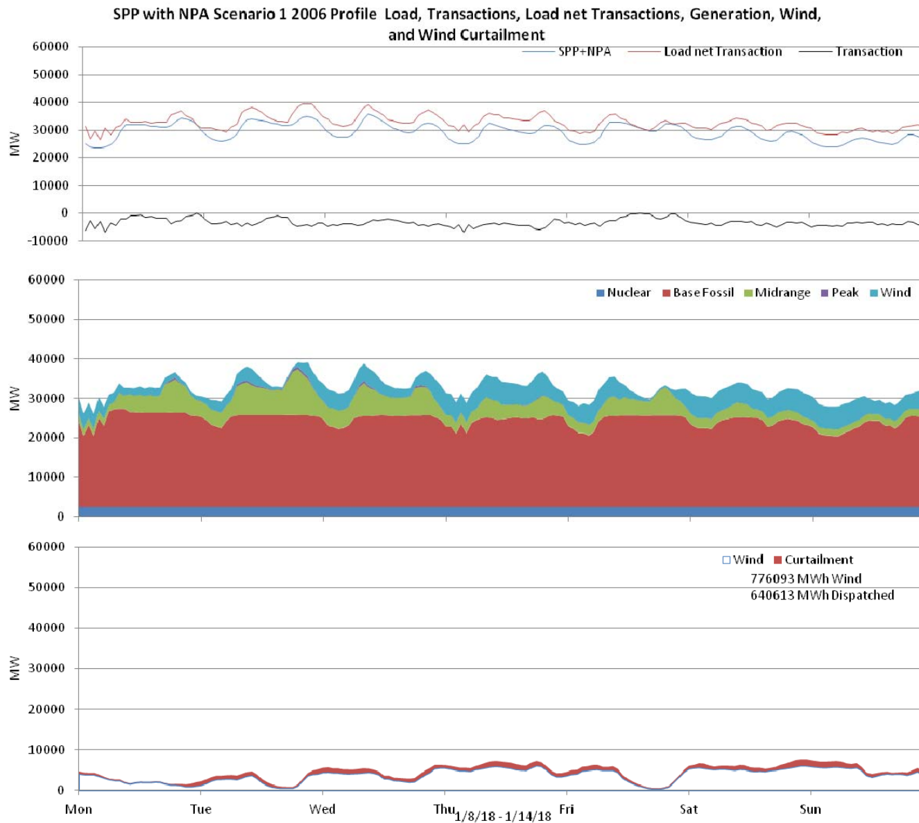
Figure 54: SPP 10% wind Penetration, 2006 Profile week of 1/8/2018
