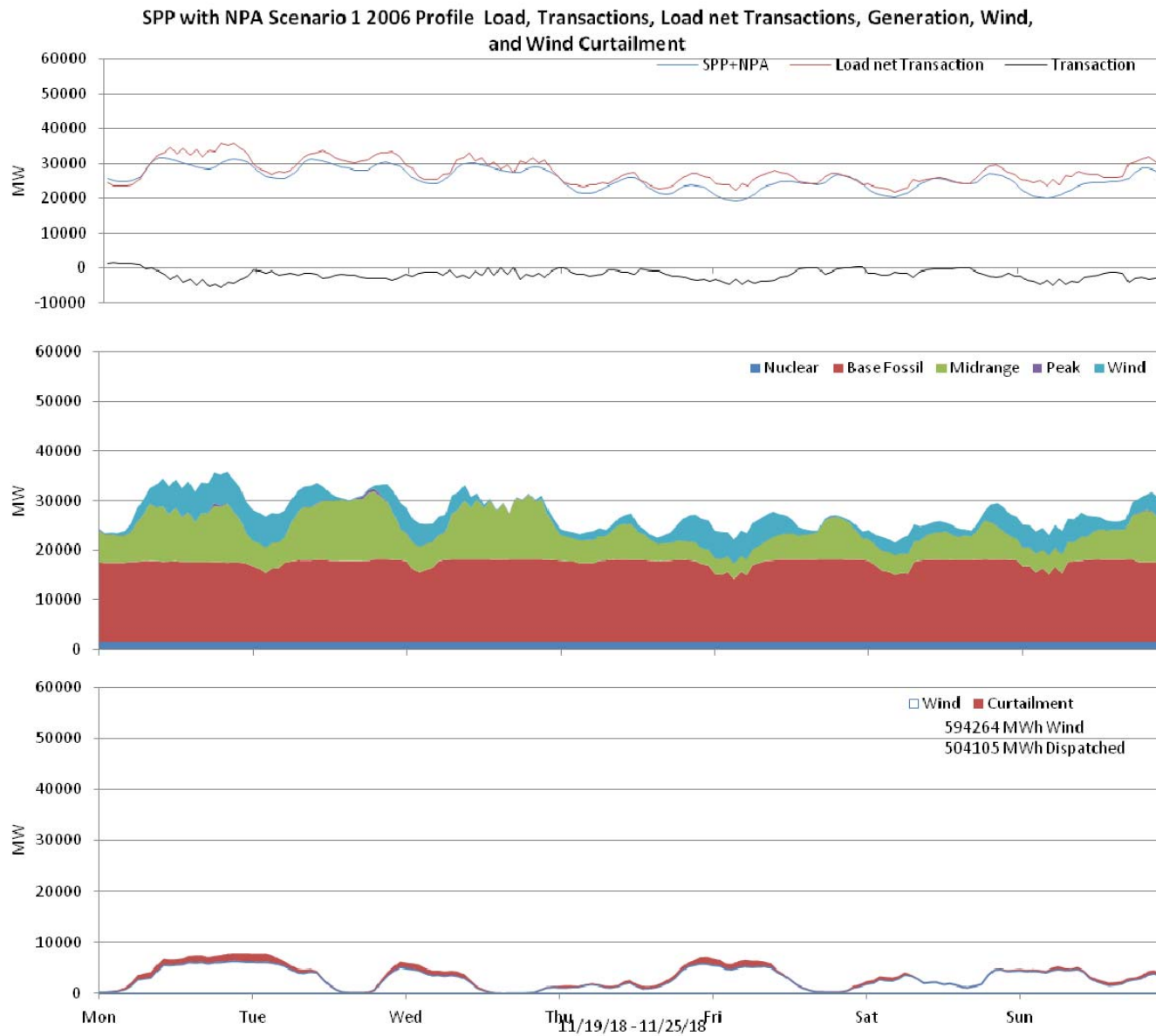
Figure 99: SPP 10% wind Penetration, 2006 Profile week of 11/19/2018
