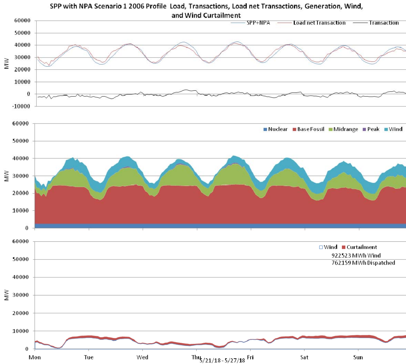
Figure 73: SPP 10% wind Penetration, 2006 Profile week of 5/21/2018
