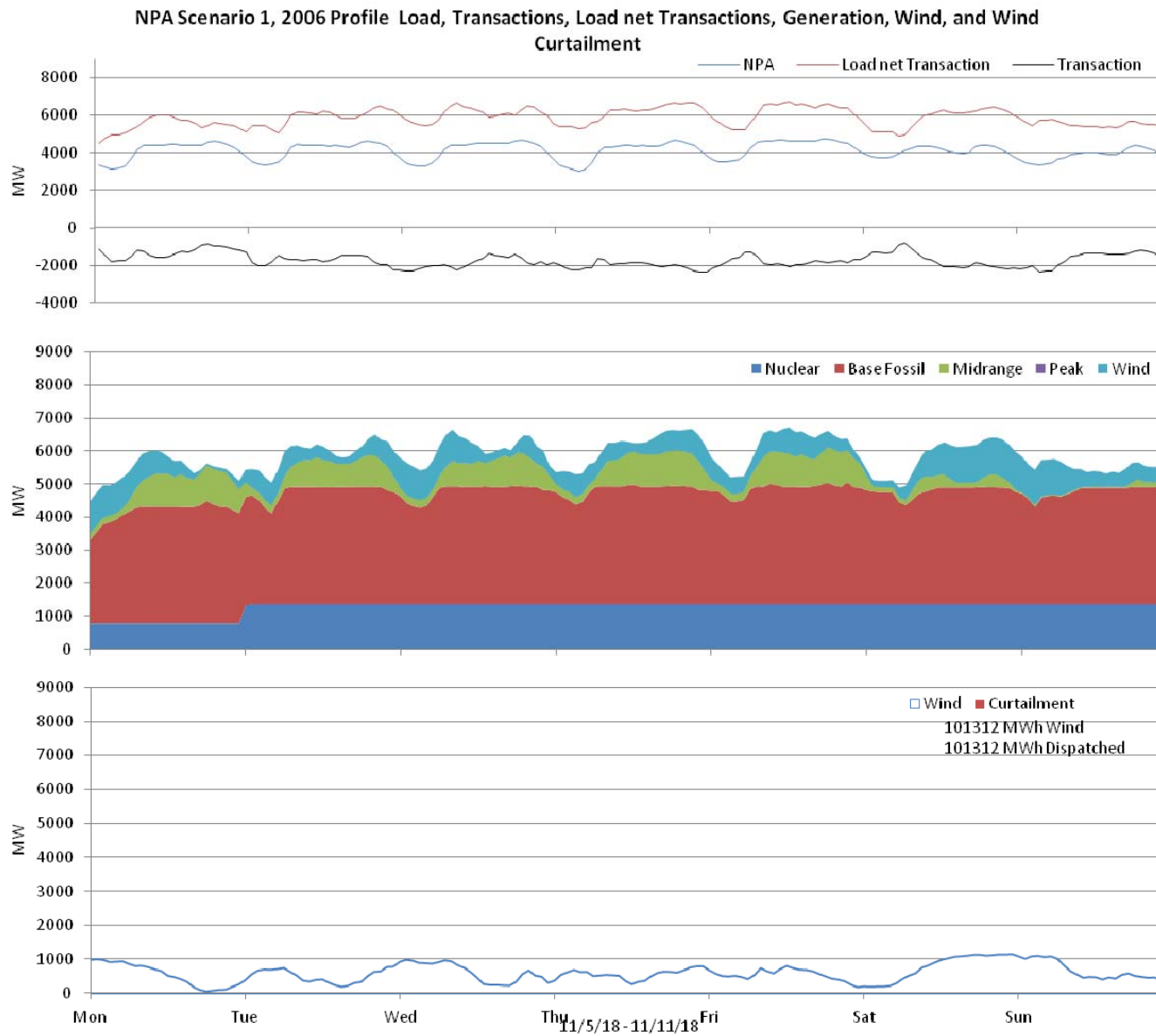
Figure 45 Nebraska 10% wind Penetration, 2006 Profile week of 11/5/2018
