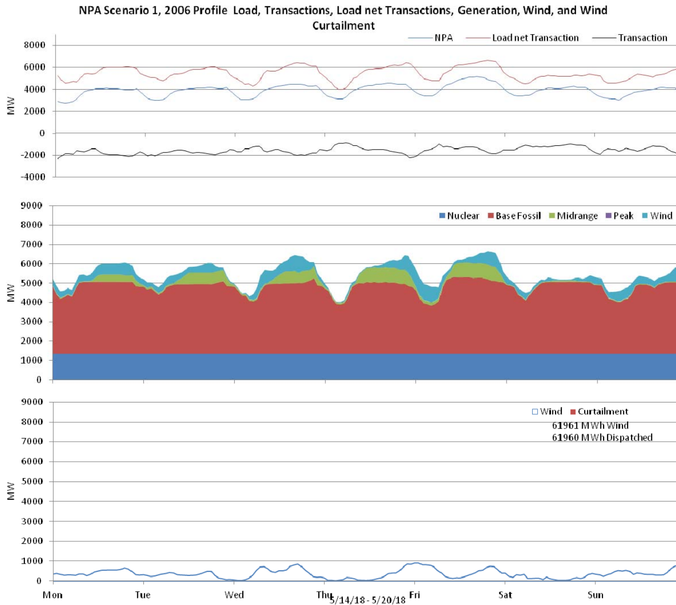
Figure 20: Nebraska 10% wind Penetration, 2006 Profile week of 5/14/2018
