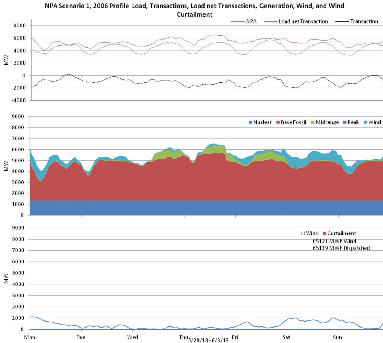
Figure 22: Nebraska 10% wind Penetration, 2006 Profile week of 5/28/2018
