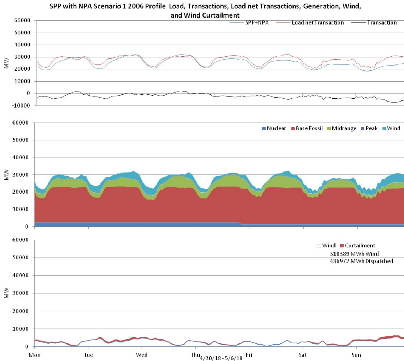
Figure 70: SPP 10% wind Penetration, 2006 Profile week of 4/30/2018
