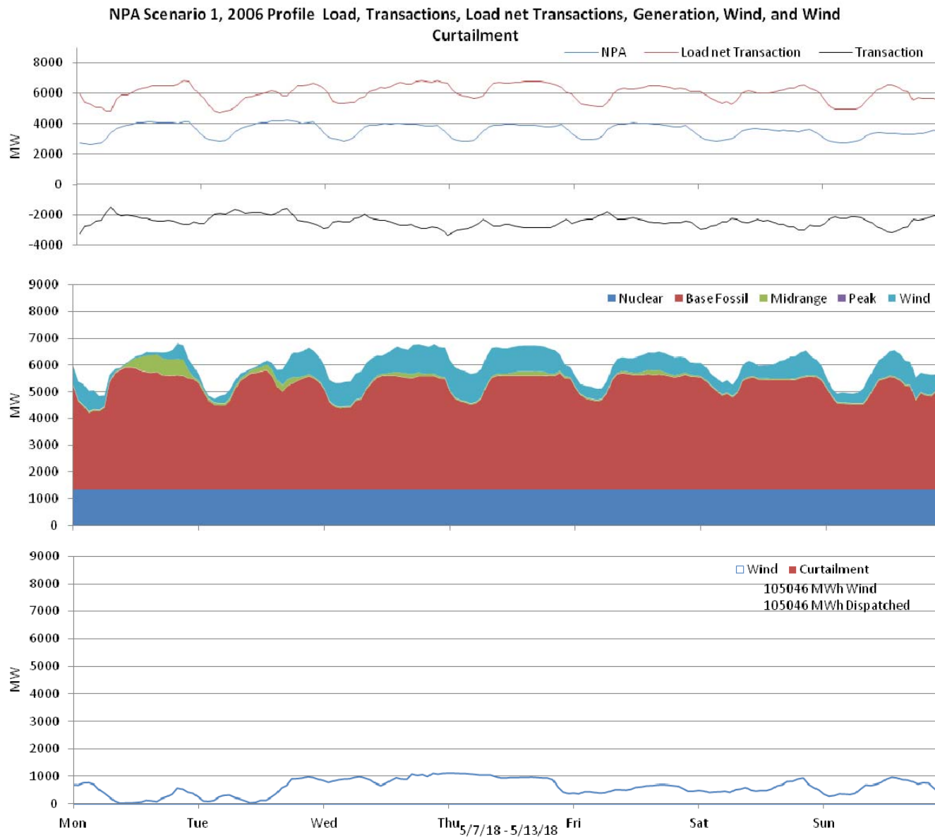
Figure 19: Nebraska 10% wind Penetration, 2006 Profile week of 5/7/2018
