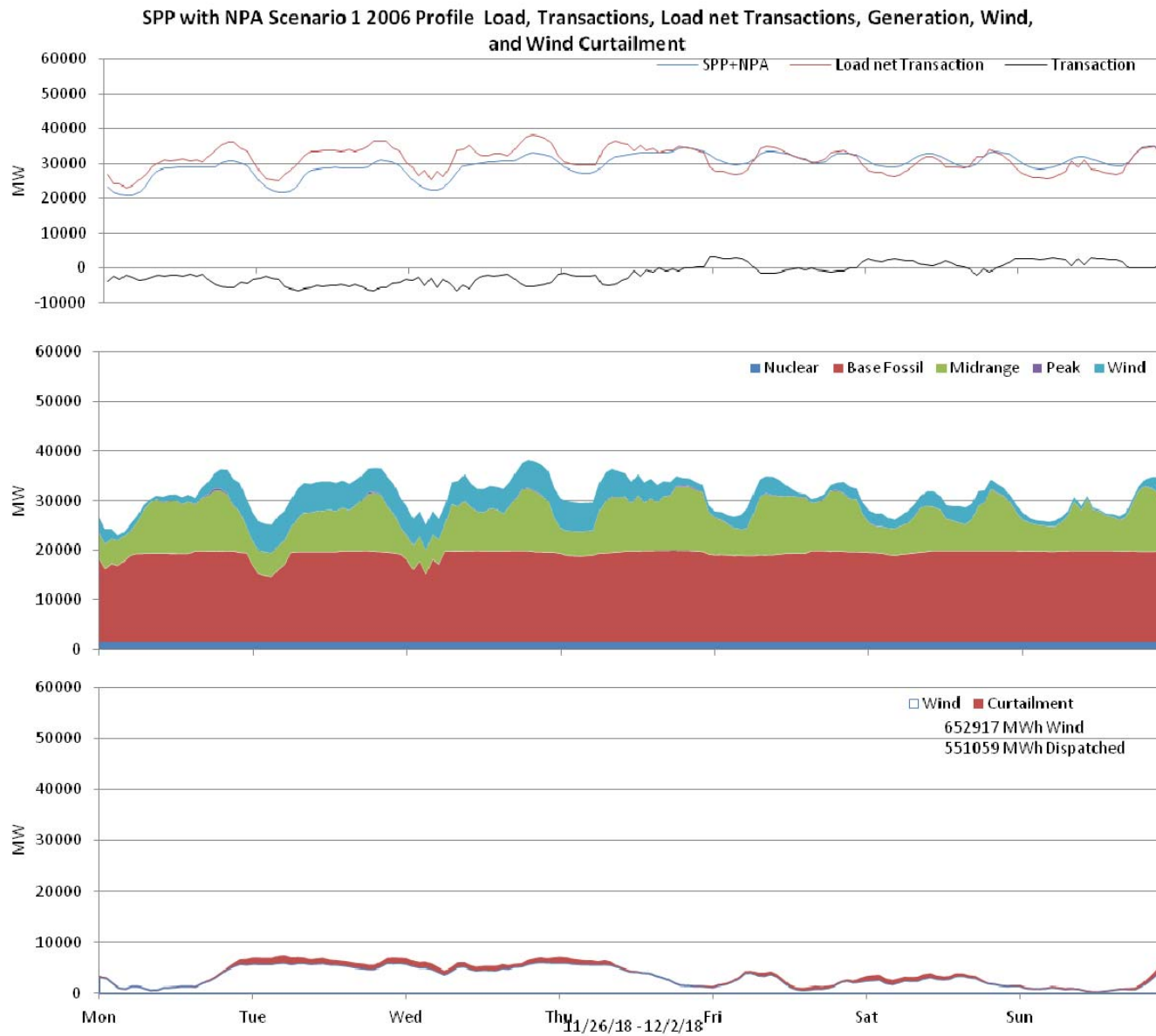
Figure 100: SPP 10% wind Penetration, 2006 Profile week of 11/26/2018
