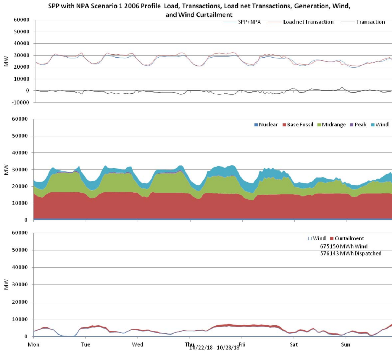
Figure 95: SPP 10% wind Penetration, 2006 Profile week of 10/22/2018
