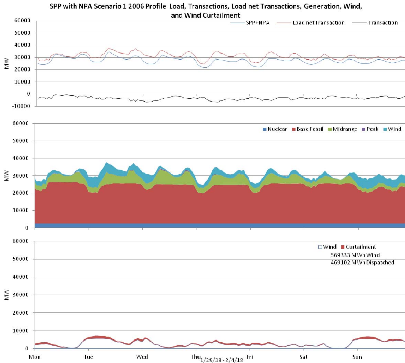
Figure 57: SPP 10% wind Penetration, 2006 Profile week of 1/29/2018
