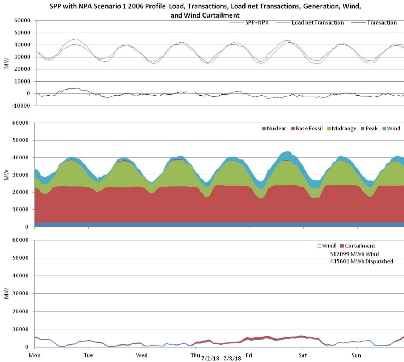
Figure 79: SPP 10% wind Penetration, 2006 Profile week of 7/2/2018
