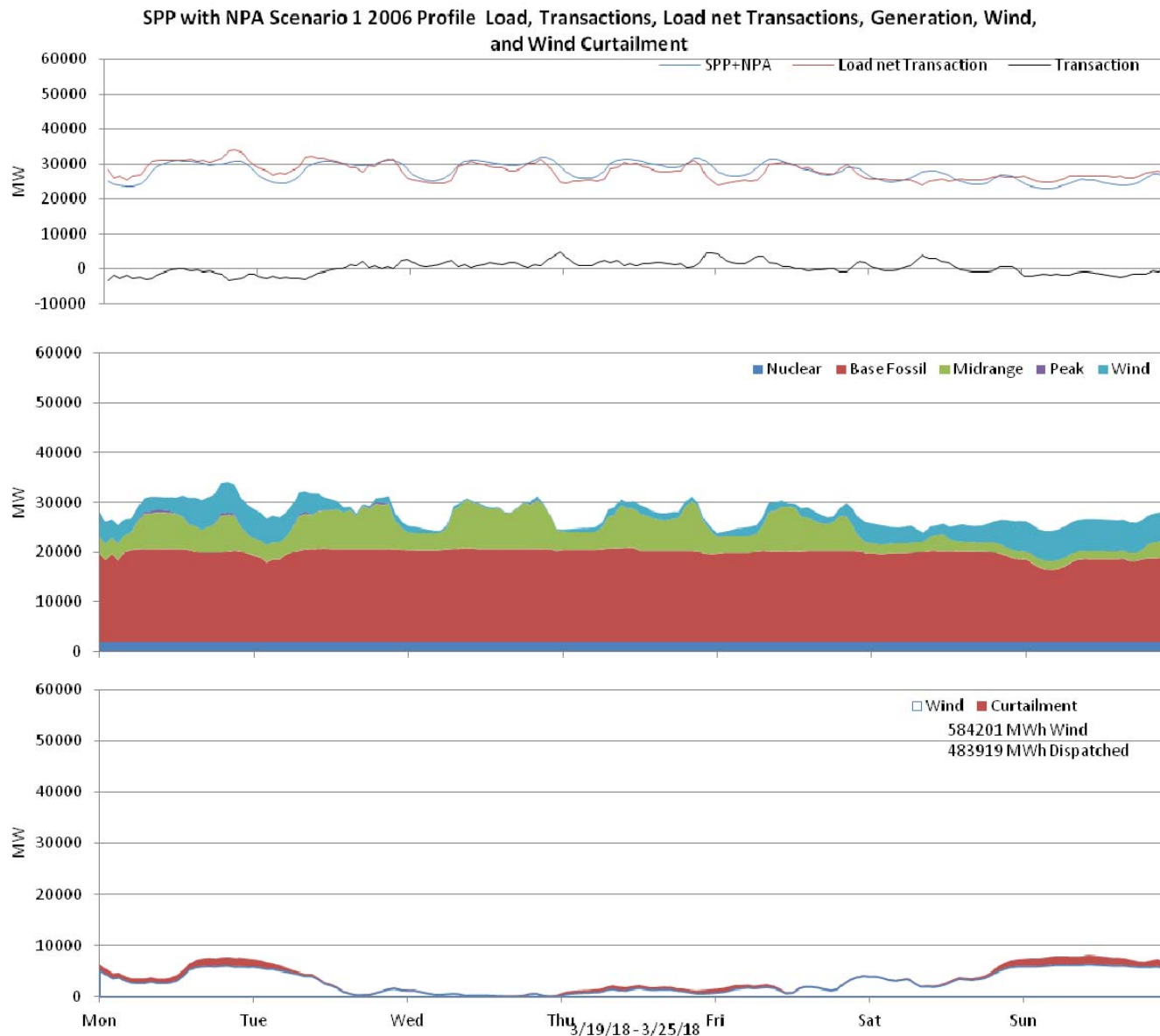
Figure 64: SPP 10% wind Penetration, 2006 Profile week of 3/19/2018
