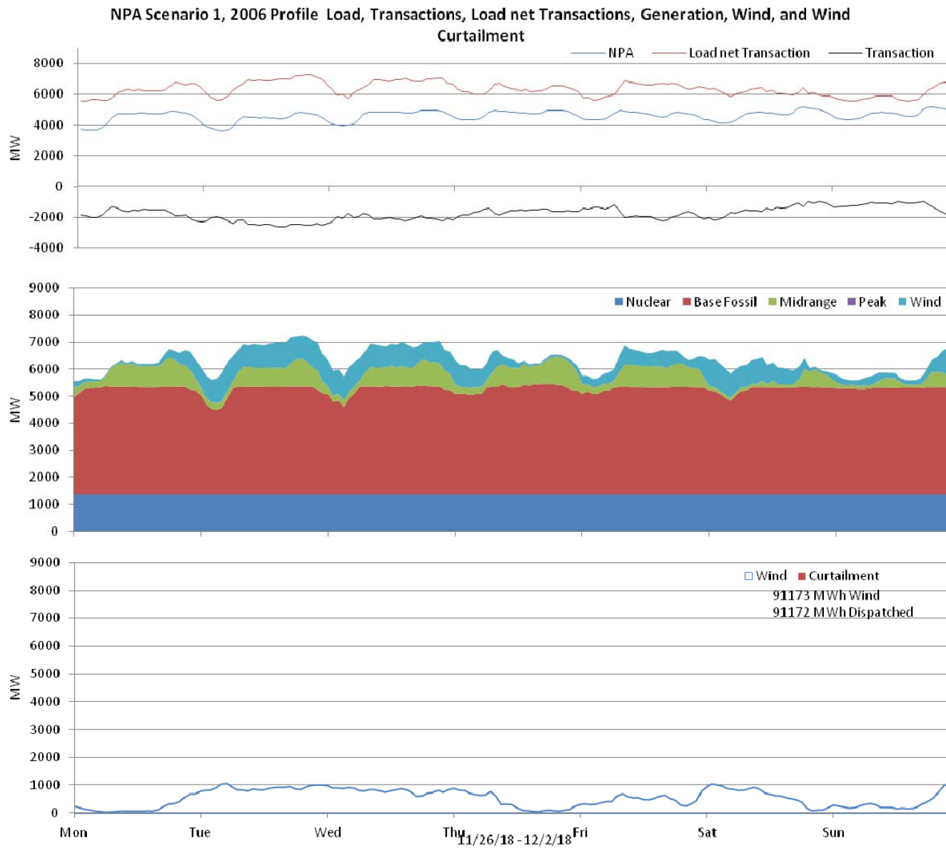
Figure 48: Nebraska 10% wind Penetration, 2006 Profile week of 11/26/2018
