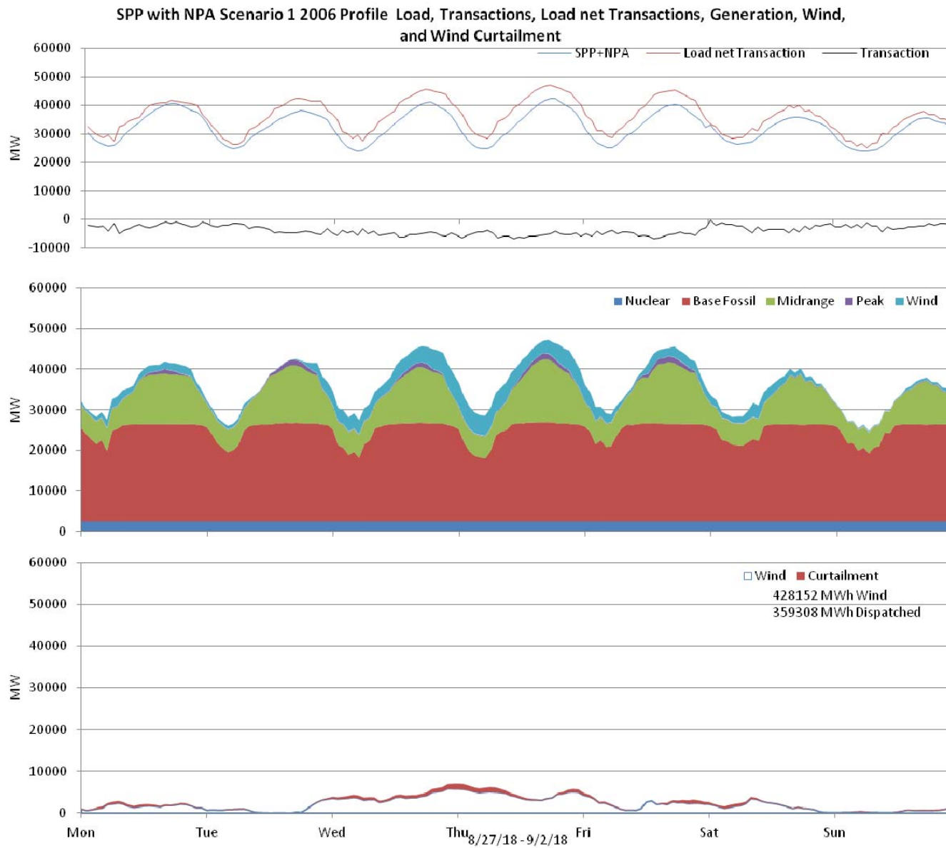
Figure 87: SPP 10% wind Penetration, 2006 Profile week of 8/27/2018
