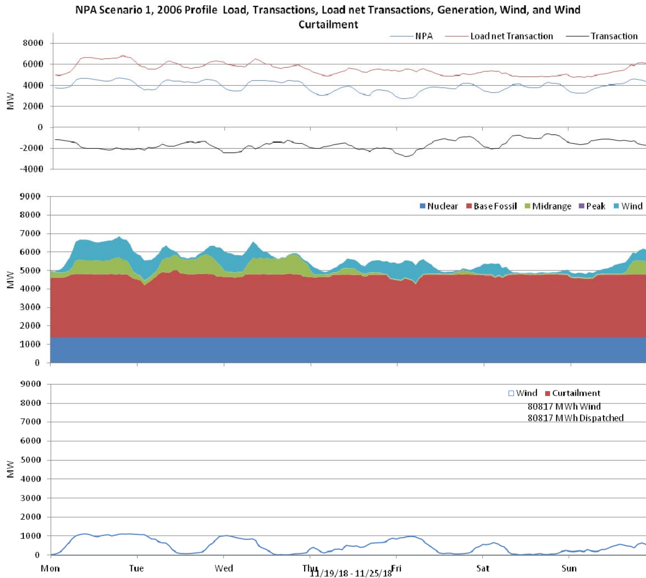
Figure 47: Nebraska 10% wind Penetration, 2006 Profile week of 11/19/2018
