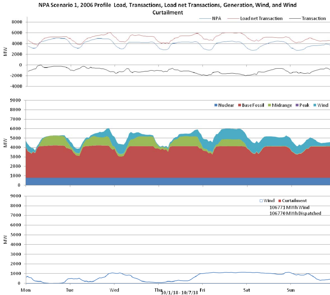
Figure 40: Nebraska 10% wind Penetration, 2006 Profile week of 10/1/2018
