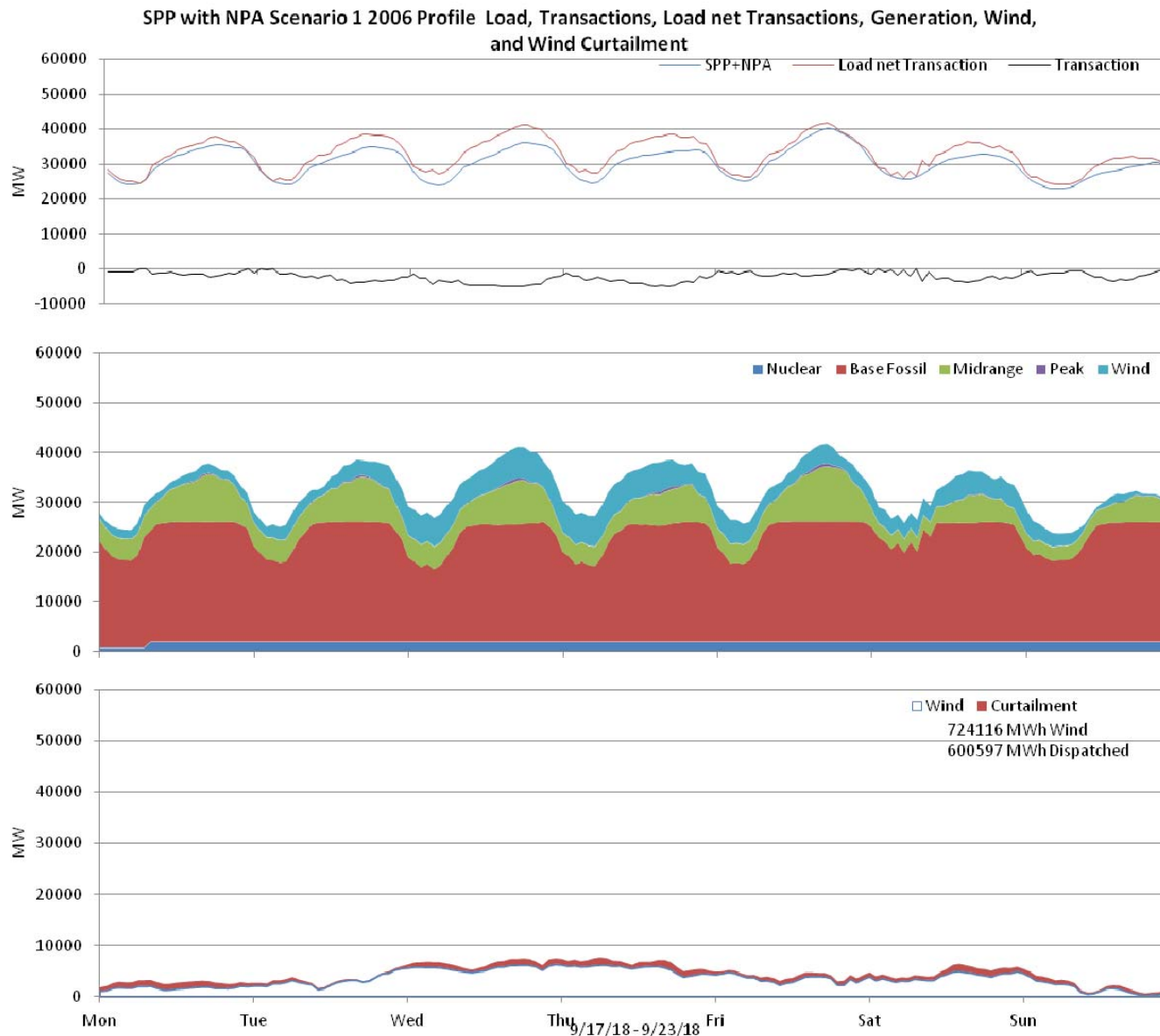
Figure 90: SPP 10% wind Penetration, 2006 Profile week of 9/17/2018
