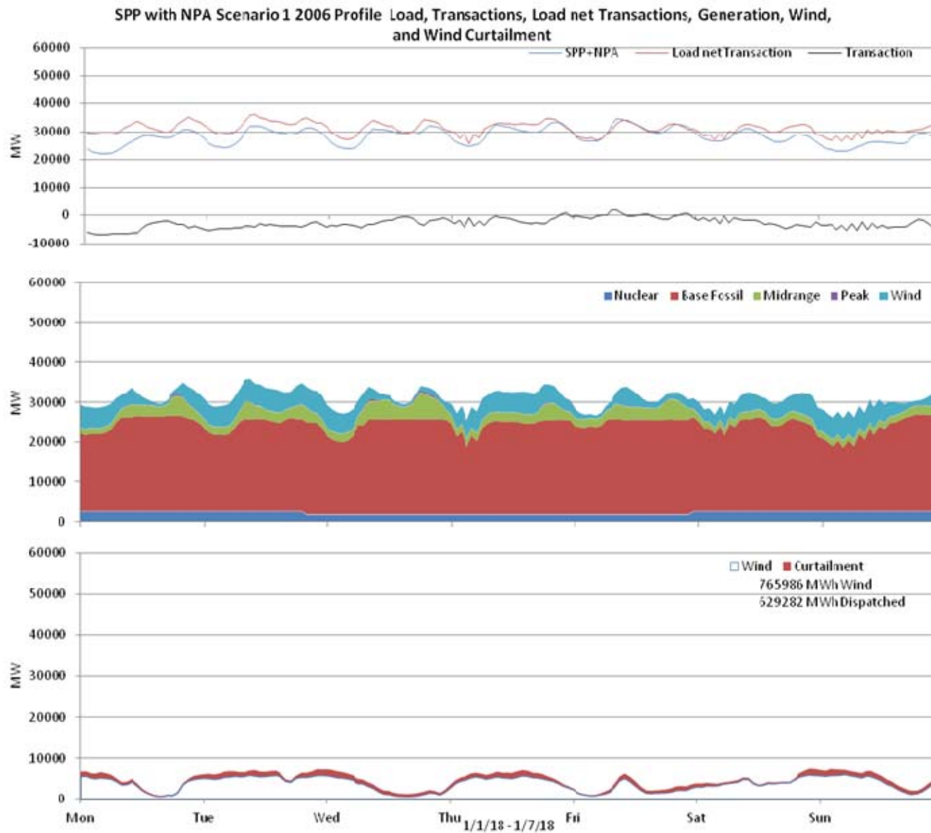
Figure 53: SPP 10% wind Penetration, 2006 Profile week of 1/1/2018
