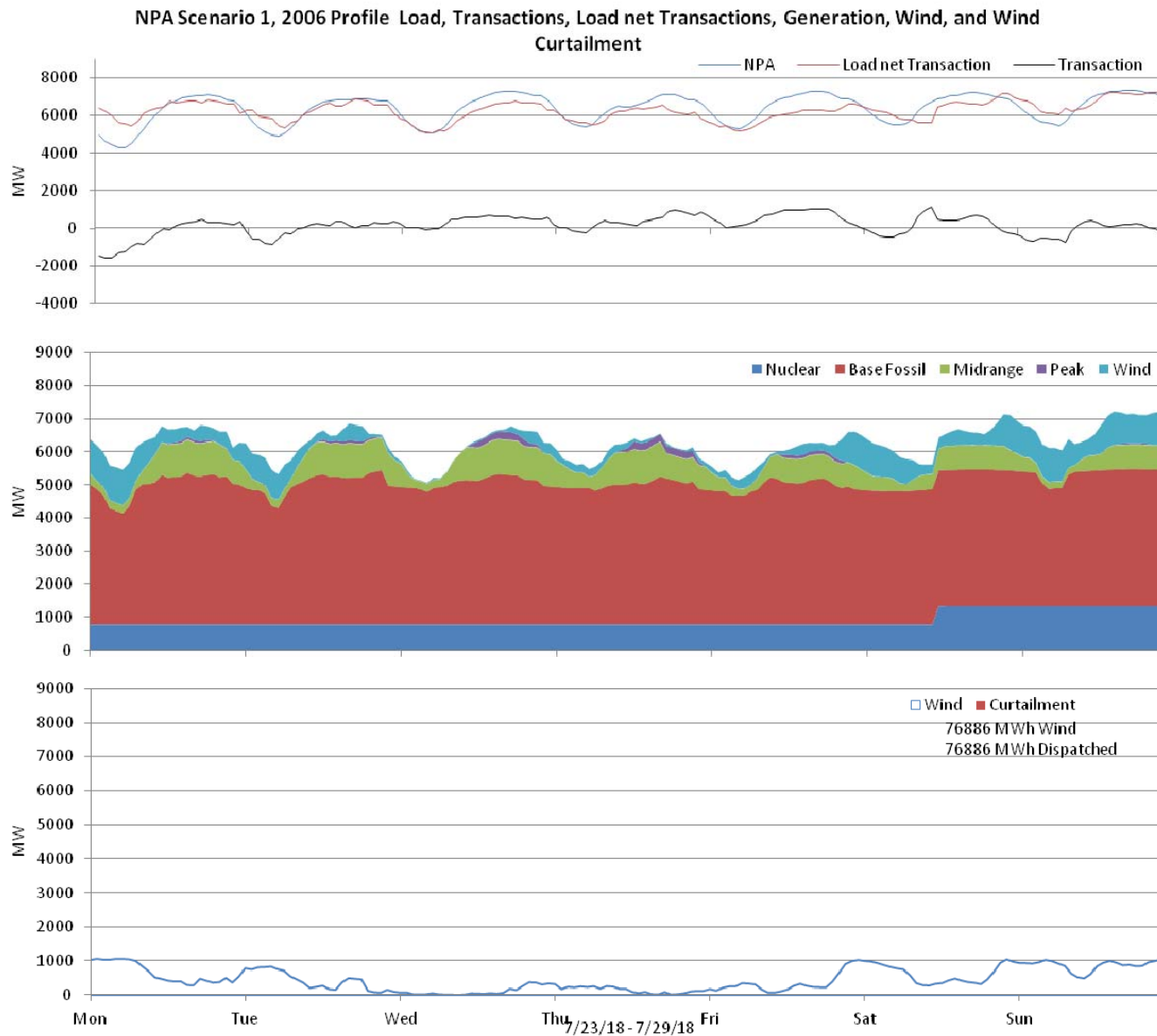
Figure 30: Nebraska 10% wind Penetration, 2006 Profile week of 7/23/2018
