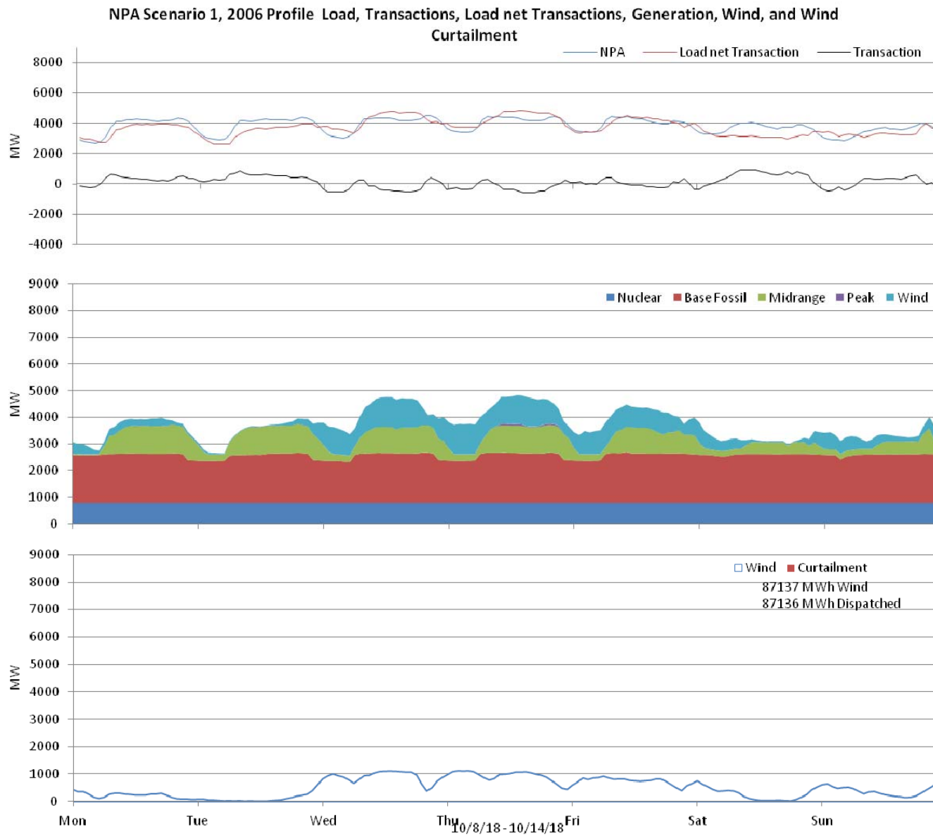
Figure 41: Nebraska 10% wind Penetration, 2006 Profile week of 10/8/2018
