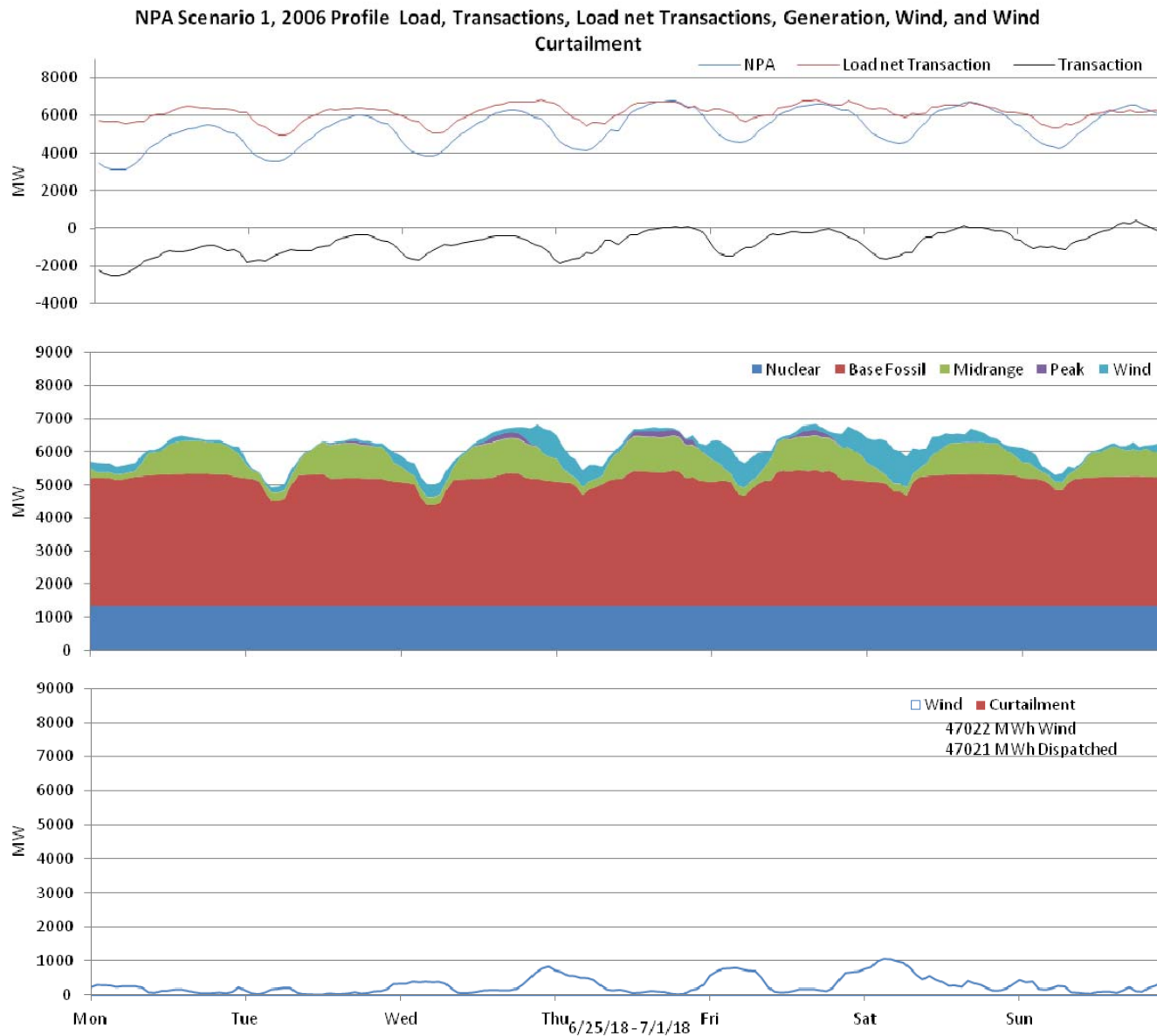
Figure 26: Nebraska 10% wind Penetration, 2006 Profile week of 6/25/2018
