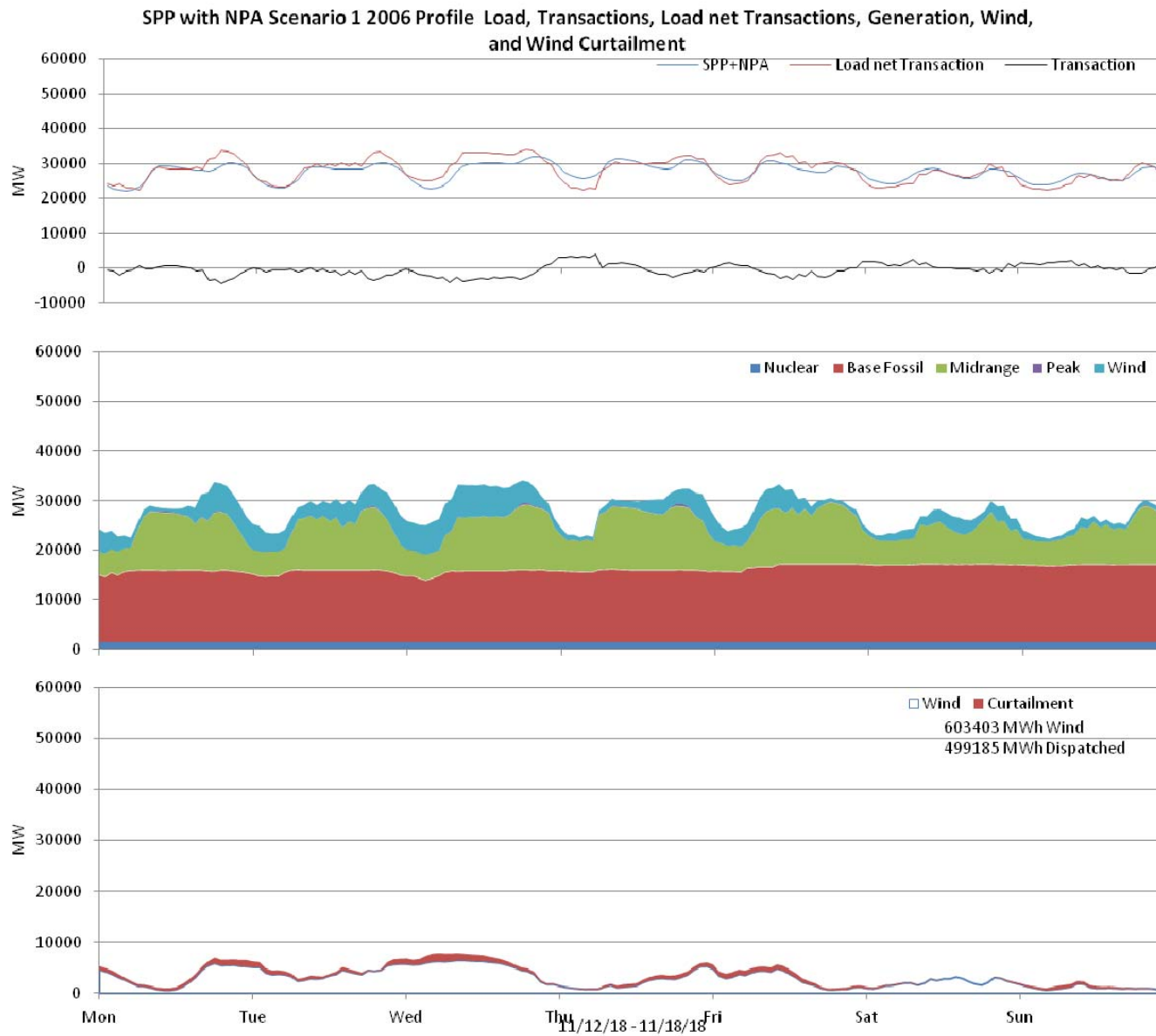
Figure 98: SPP 10% wind Penetration, 2006 Profile week of 11/12/2018
