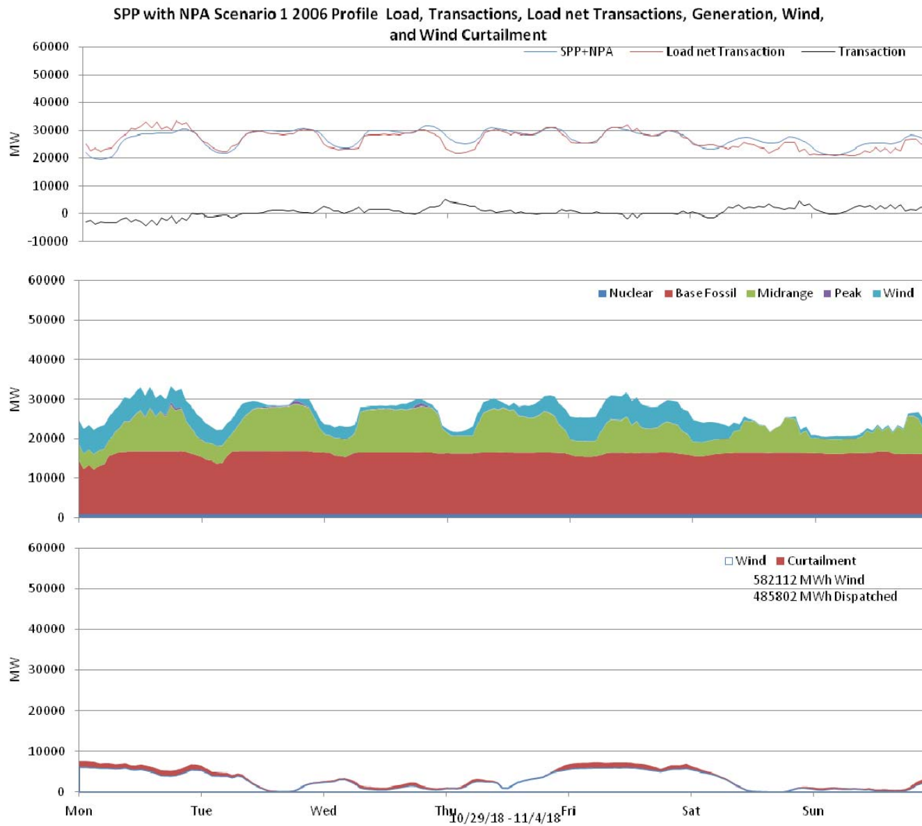
Figure 96: SPP 10% wind Penetration, 2006 Profile week of 10/29/2018
