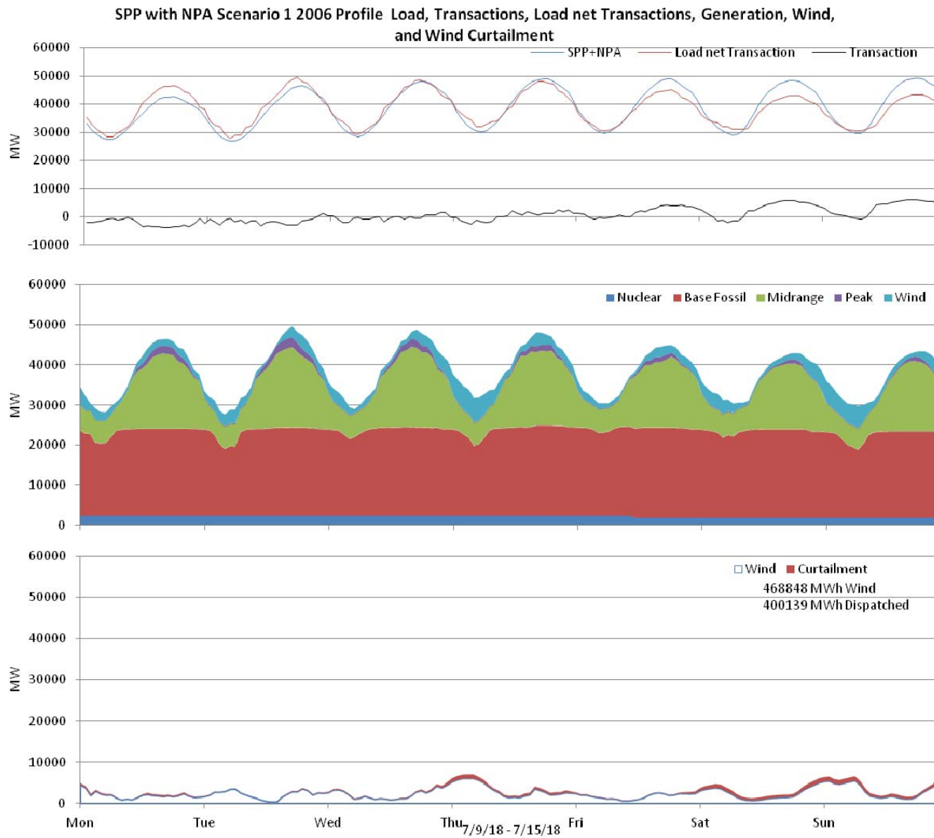
Figure 80: SPP 10% wind Penetration, 2006 Profile week of 7/9/2018
