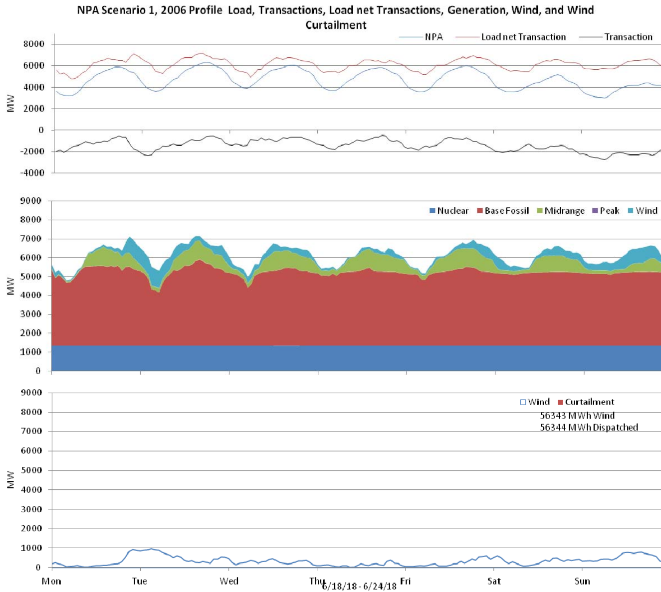
Figure 25: Nebraska 10% wind Penetration, 2006 Profile week of 6/18/2018
