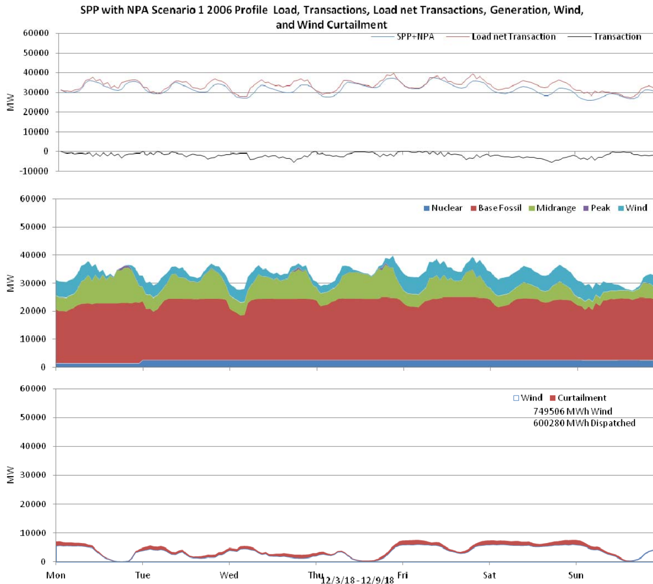
Figure 101: SPP 10% wind Penetration, 2006 Profile week of 12/3/2018
