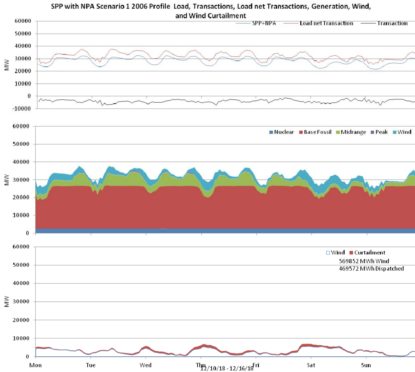
Figure 102: SPP 10% wind Penetration, 2006 Profile week of 12/10/2018
