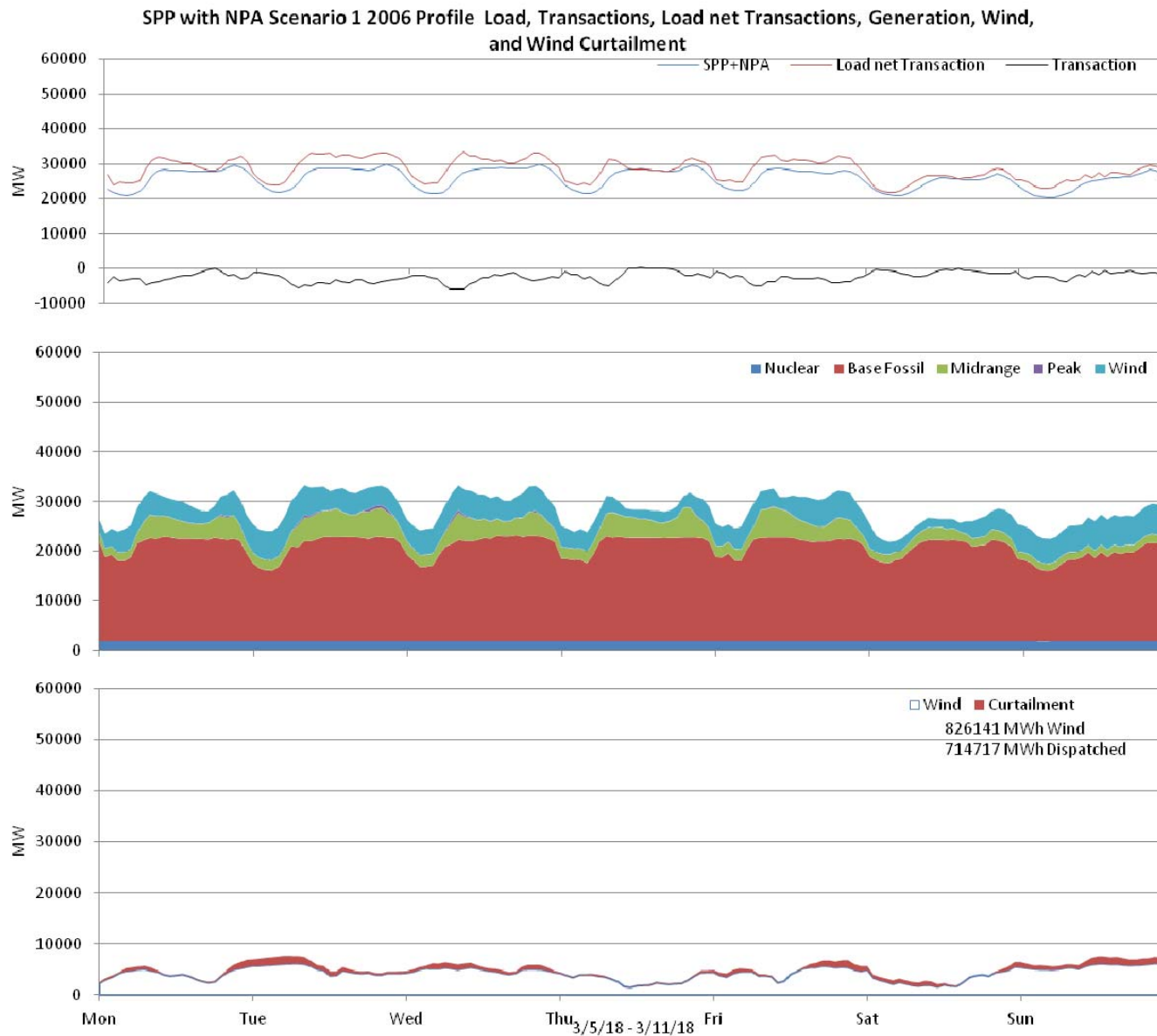
Figure 62: SPP 10% wind Penetration, 2006 Profile week of 3/5/2018
