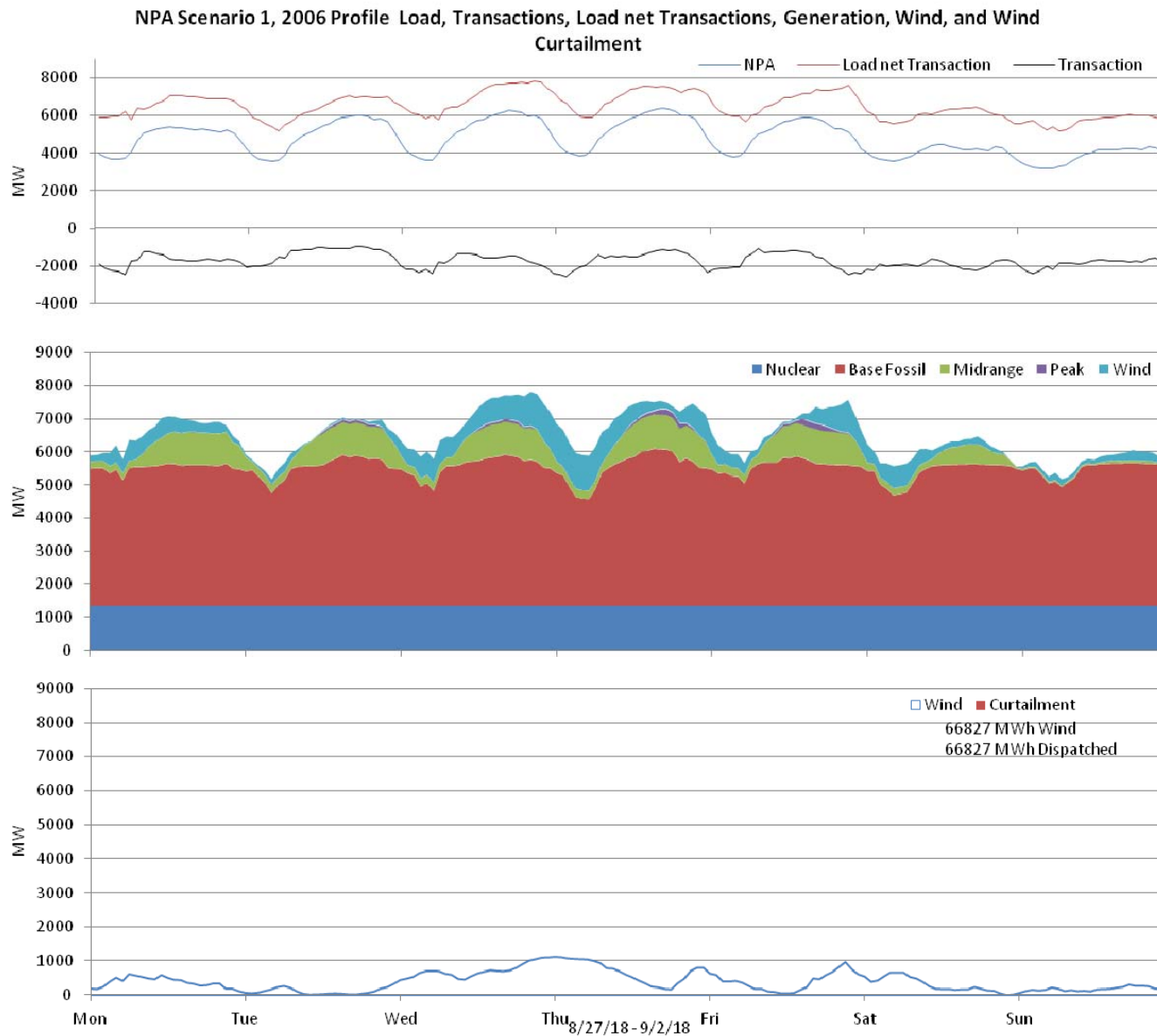
Figure 35: Nebraska 10% wind Penetration, 2006 Profile week of 8/27/2018
