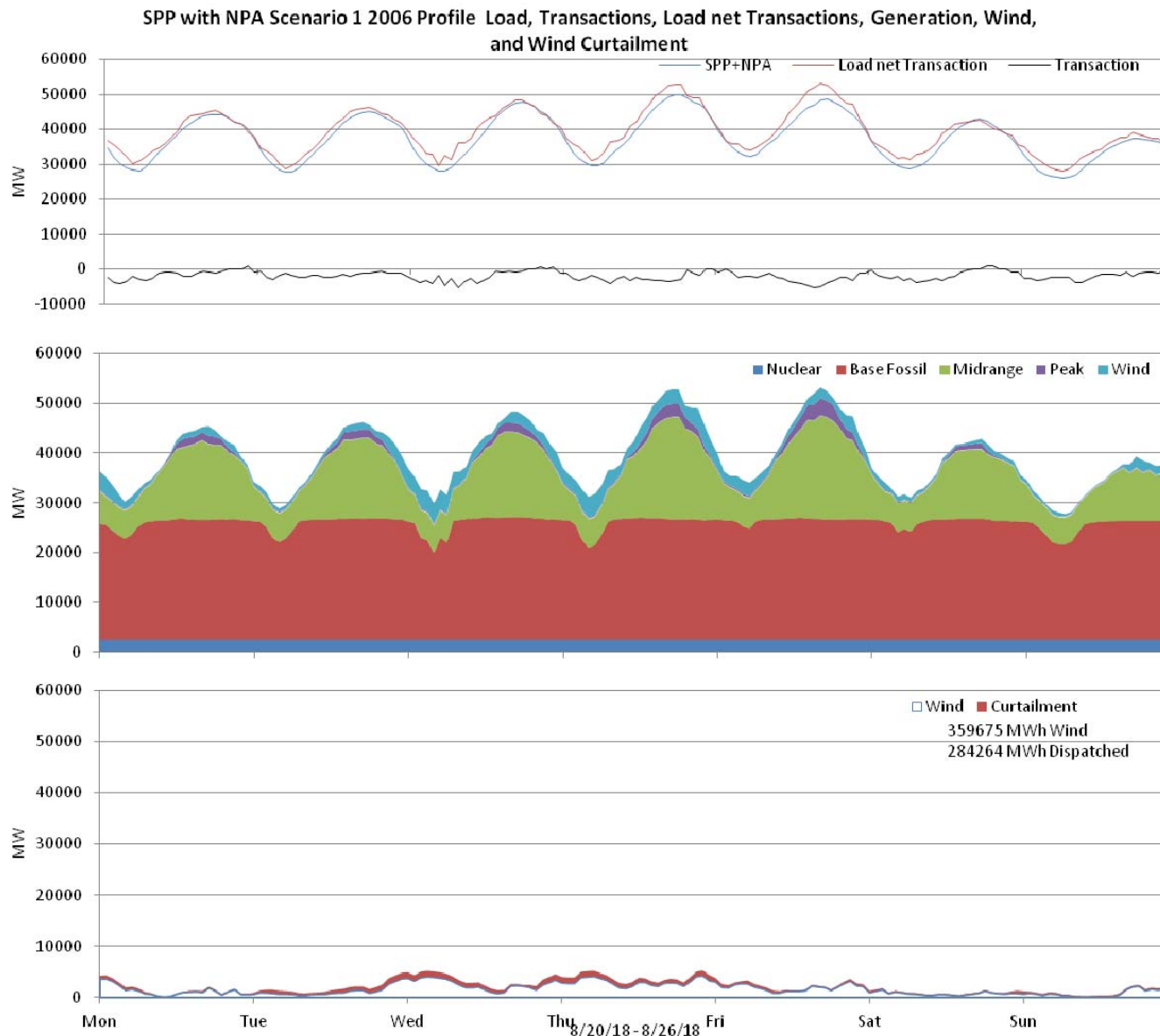
Figure 86: SPP 10% wind Penetration, 2006 Profile week of 8/20/2018
