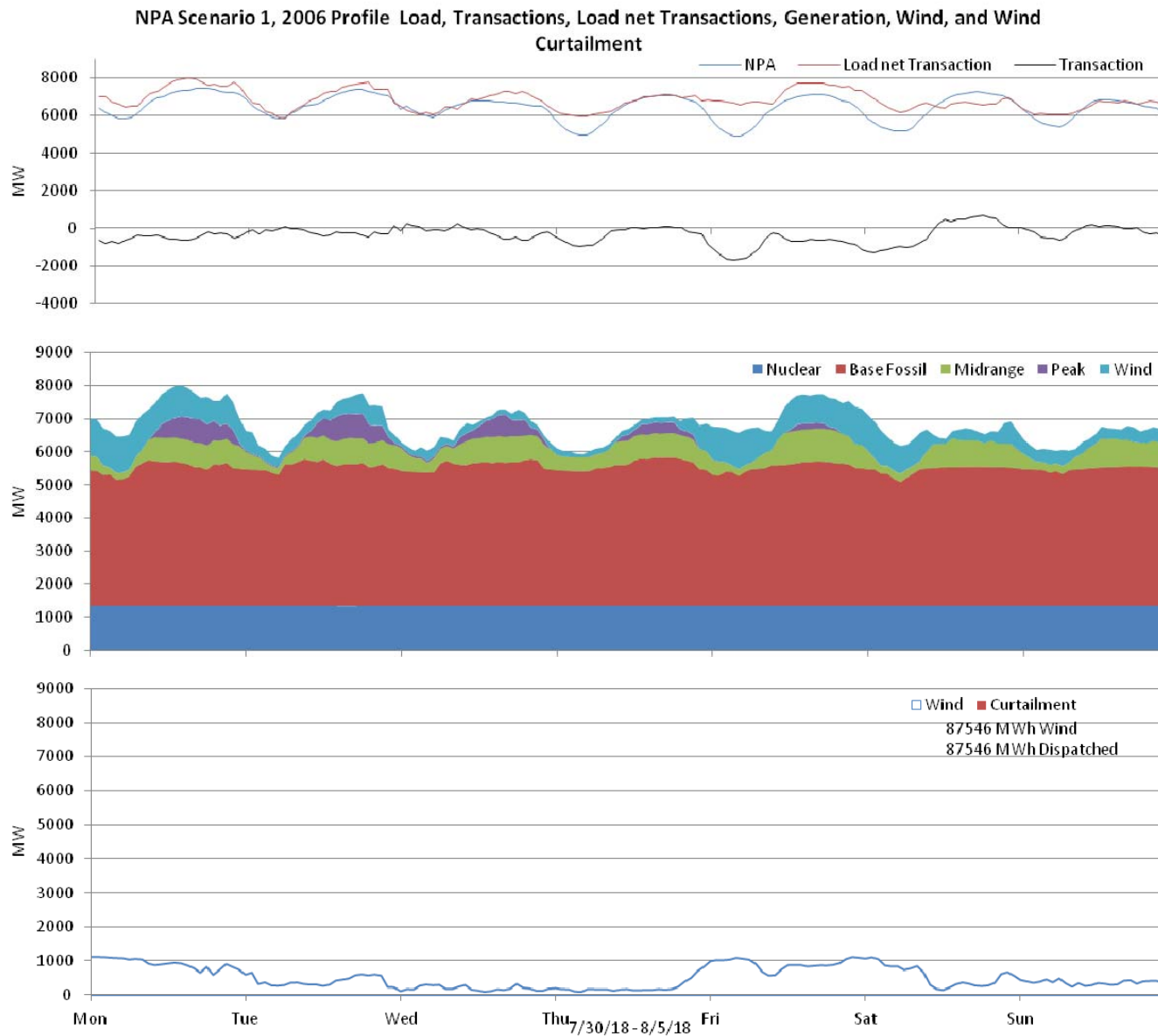
Figure 31: Nebraska 10% wind Penetration, 2006 Profile week of 7/30/2018
