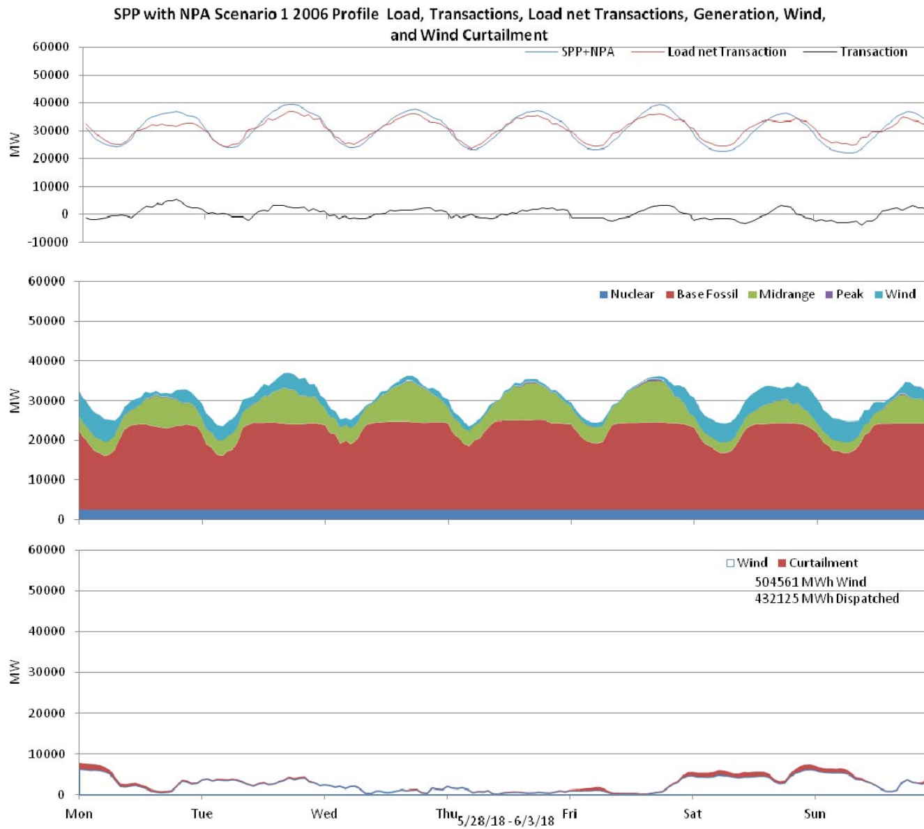
Figure 74: SPP 10% wind Penetration, 2006 Profile week of 5/28/2018
