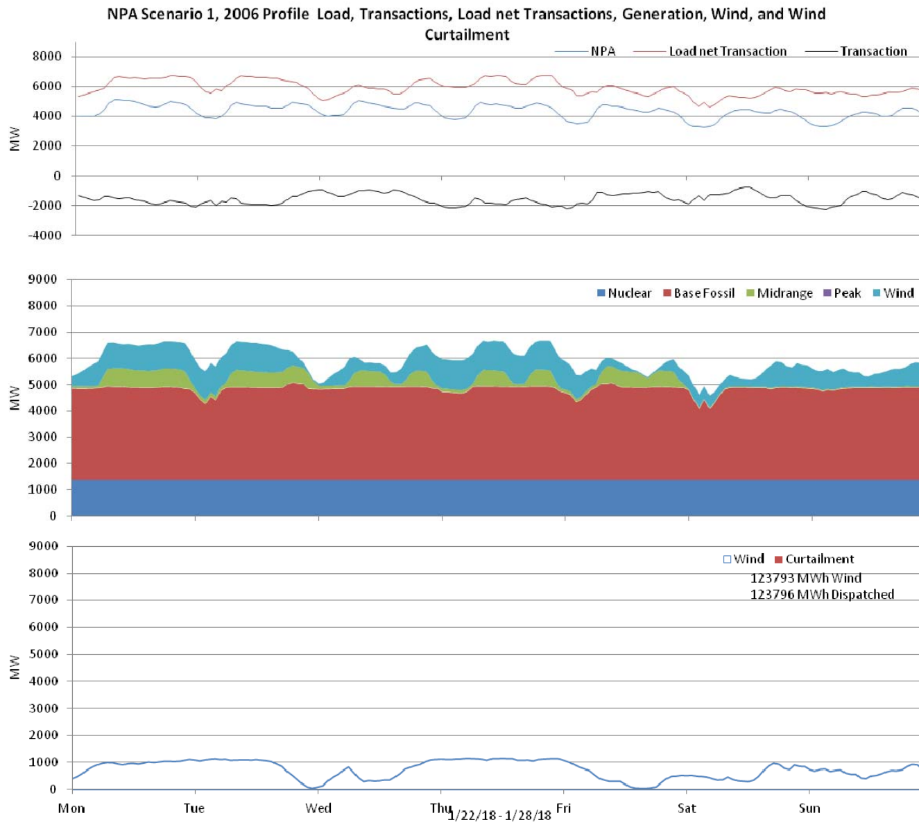
Figure 4: Nebraska 10% wind Penetration, 2006 Profile week of 1/22/2018
