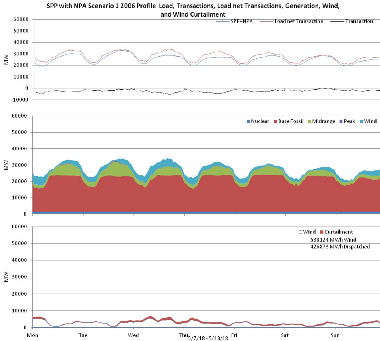
Figure 71: SPP 10% wind Penetration, 2006 Profile week of 5/7/2018
