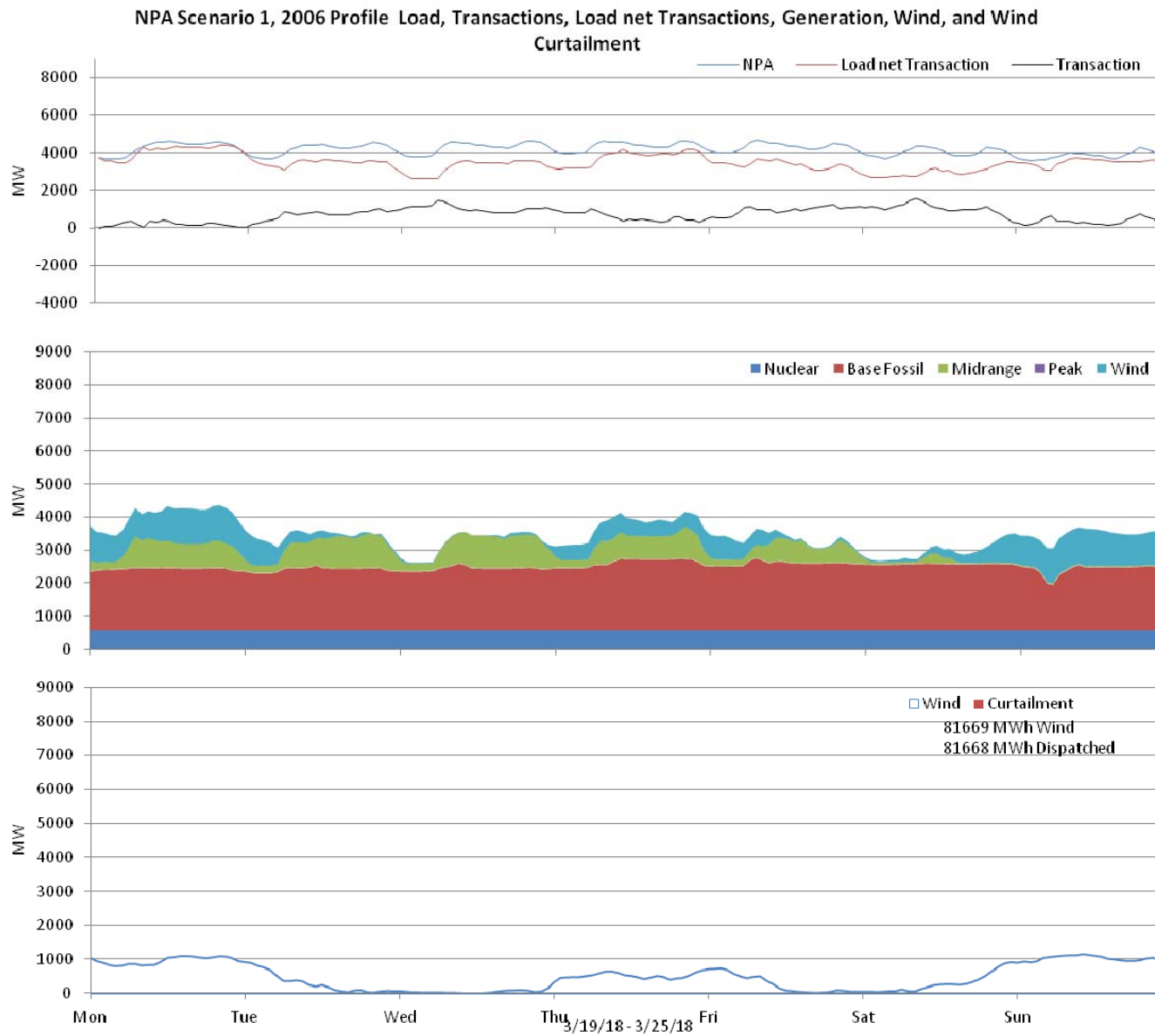
Figure 12: Nebraska 10% wind Penetration, 2006 Profile week of 3/19/2018
