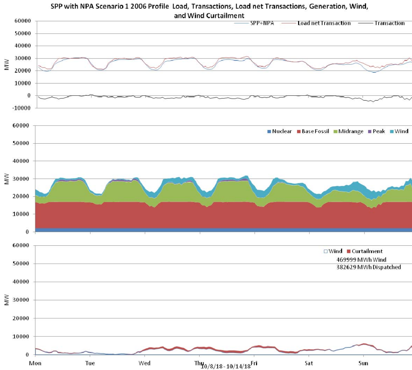
Figure 93: SPP 10% wind Penetration, 2006 Profile week of 10/8/2018
