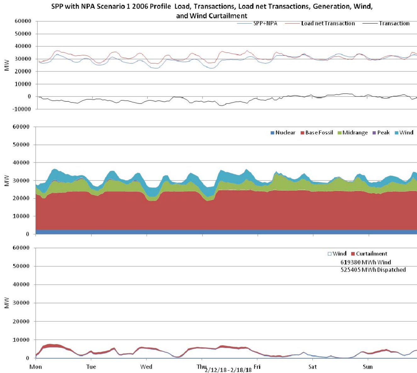
Figure 59: SPP 10% wind Penetration, 2006 Profile week of 2/12/2018
