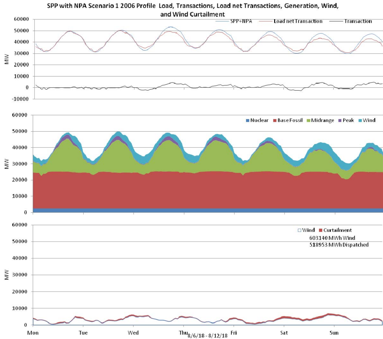
Figure 84: SPP 10% wind Penetration, 2006 Profile week of 8/6/2018
