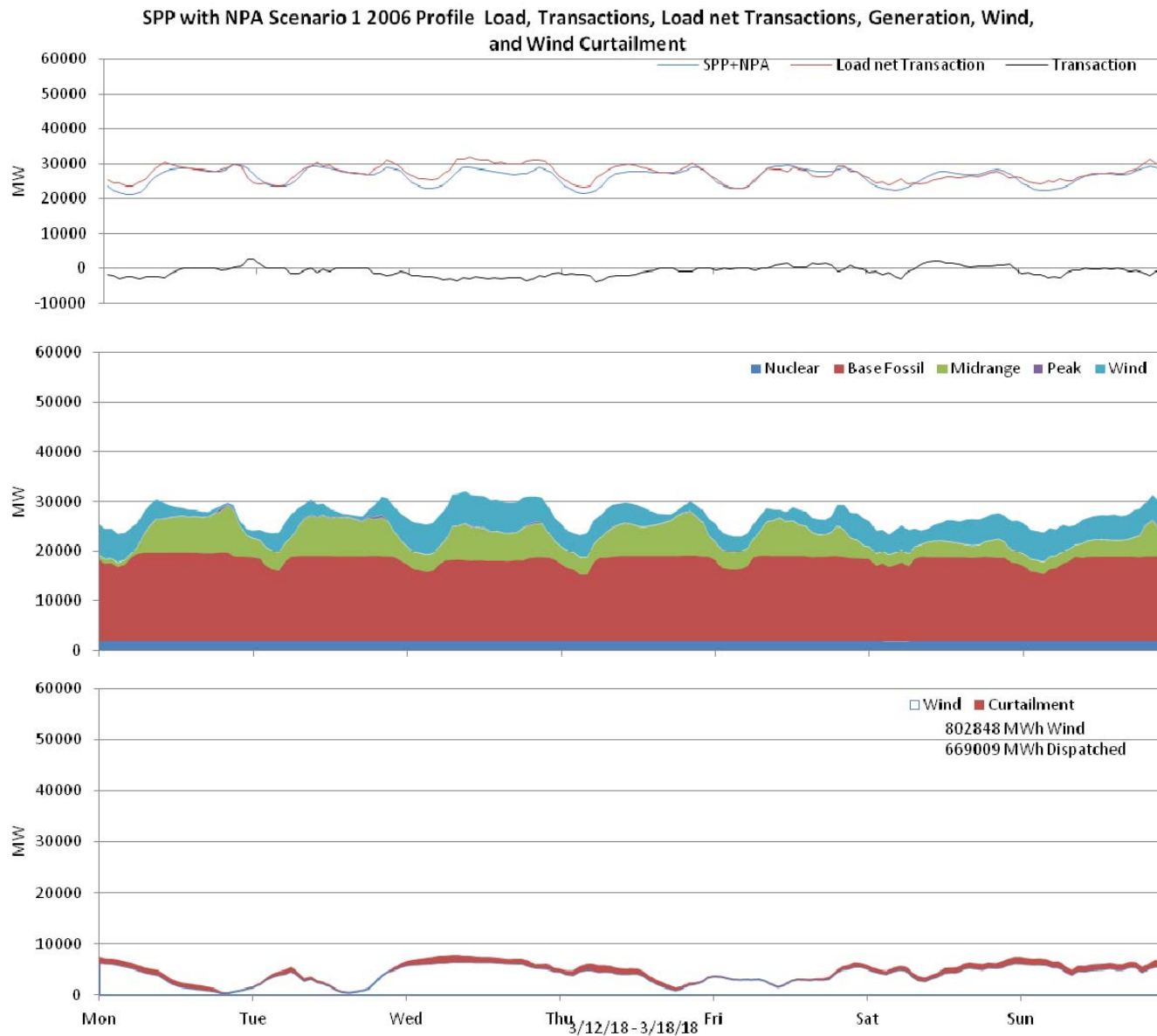
Figure 63: SPP 10% wind Penetration, 2006 Profile week of 3/12/2018
