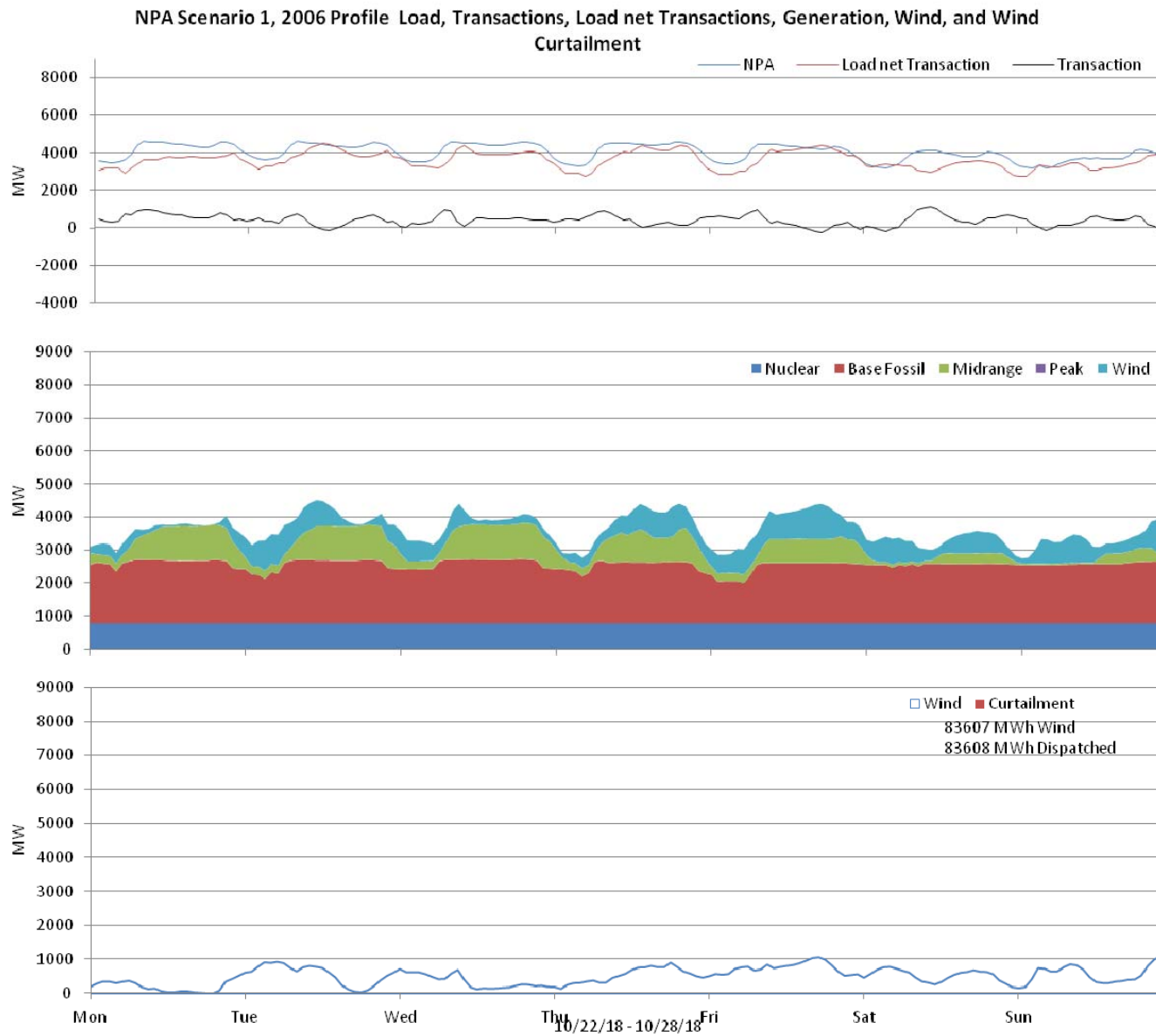
Figure 43 Nebraska 10% wind Penetration, 2006 Profile week of 10/22/2018
