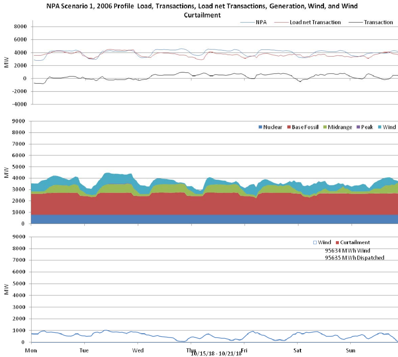
Figure 42: Nebraska 10% wind Penetration, 2006 Profile week of 10/15/2018
