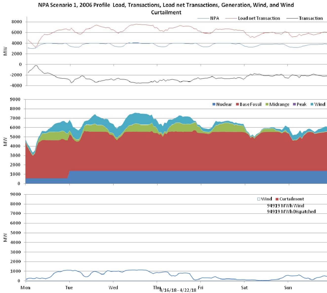
Figure 16: Nebraska 10% wind Penetration, 2006 Profile week of 4/16/2018
