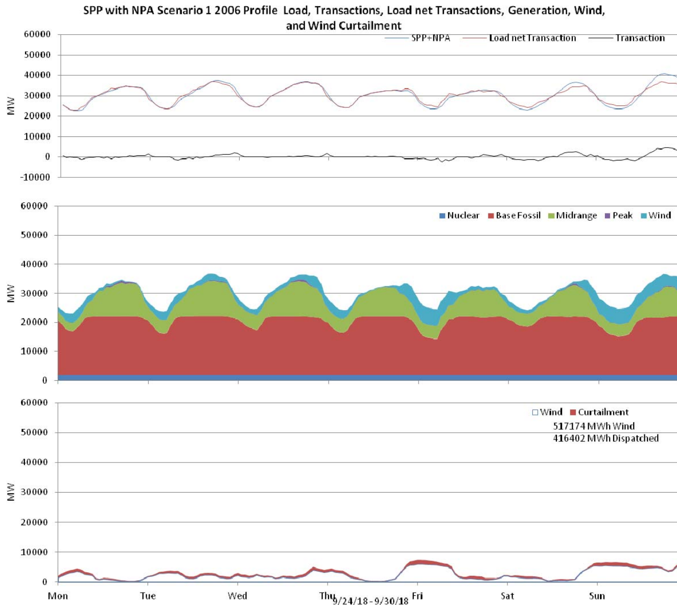
Figure 91: SPP 10% wind Penetration, 2006 Profile week of 9/24/2018
