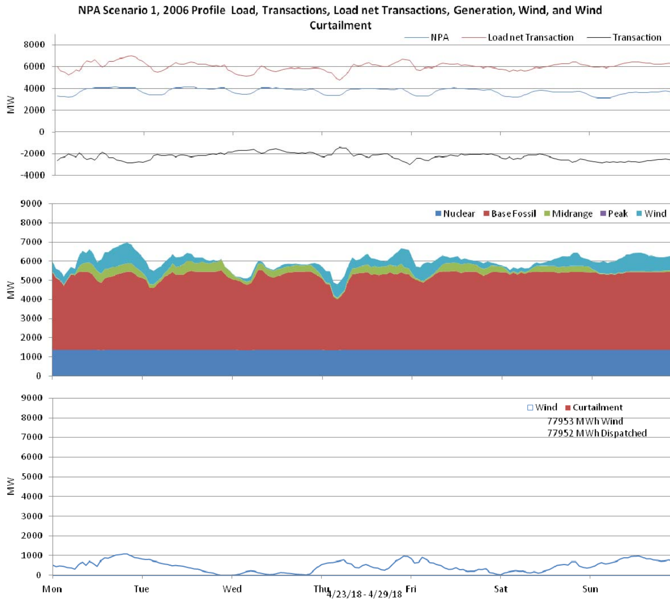
Figure 17: Nebraska 10% wind Penetration, 2006 Profile week of 4/23/2018
