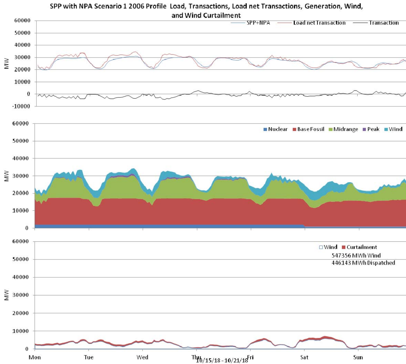
Figure 94: SPP 10% wind Penetration, 2006 Profile week of 10/15/2018
