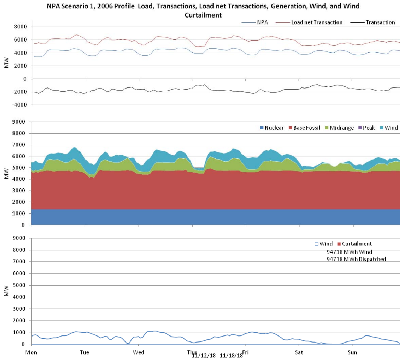
Figure 46: Nebraska 10% wind Penetration, 2006 Profile week of 11/12/2018
