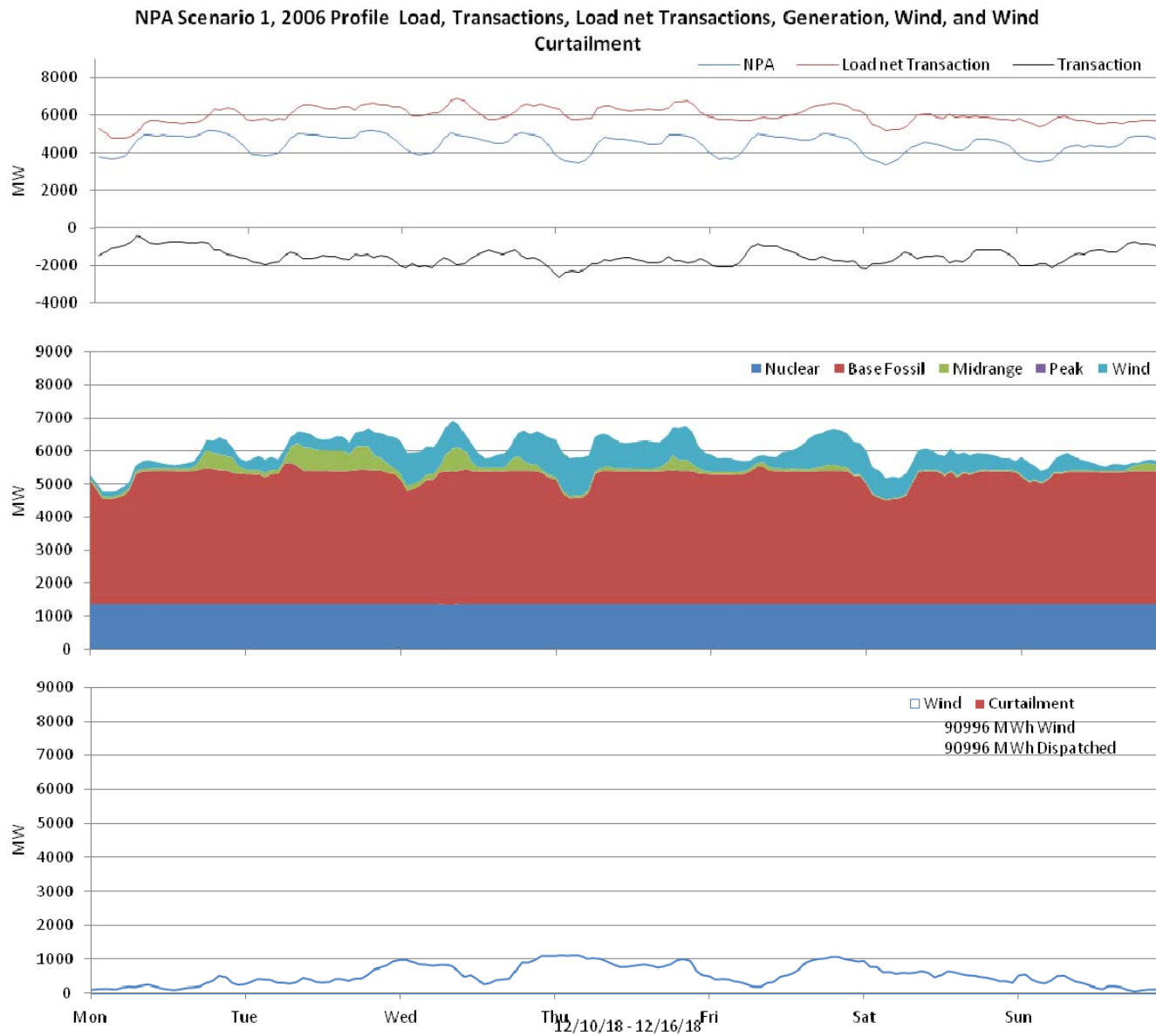
Figure 50: Nebraska 10% wind Penetration, 2006 Profile week of 12/10/2018
