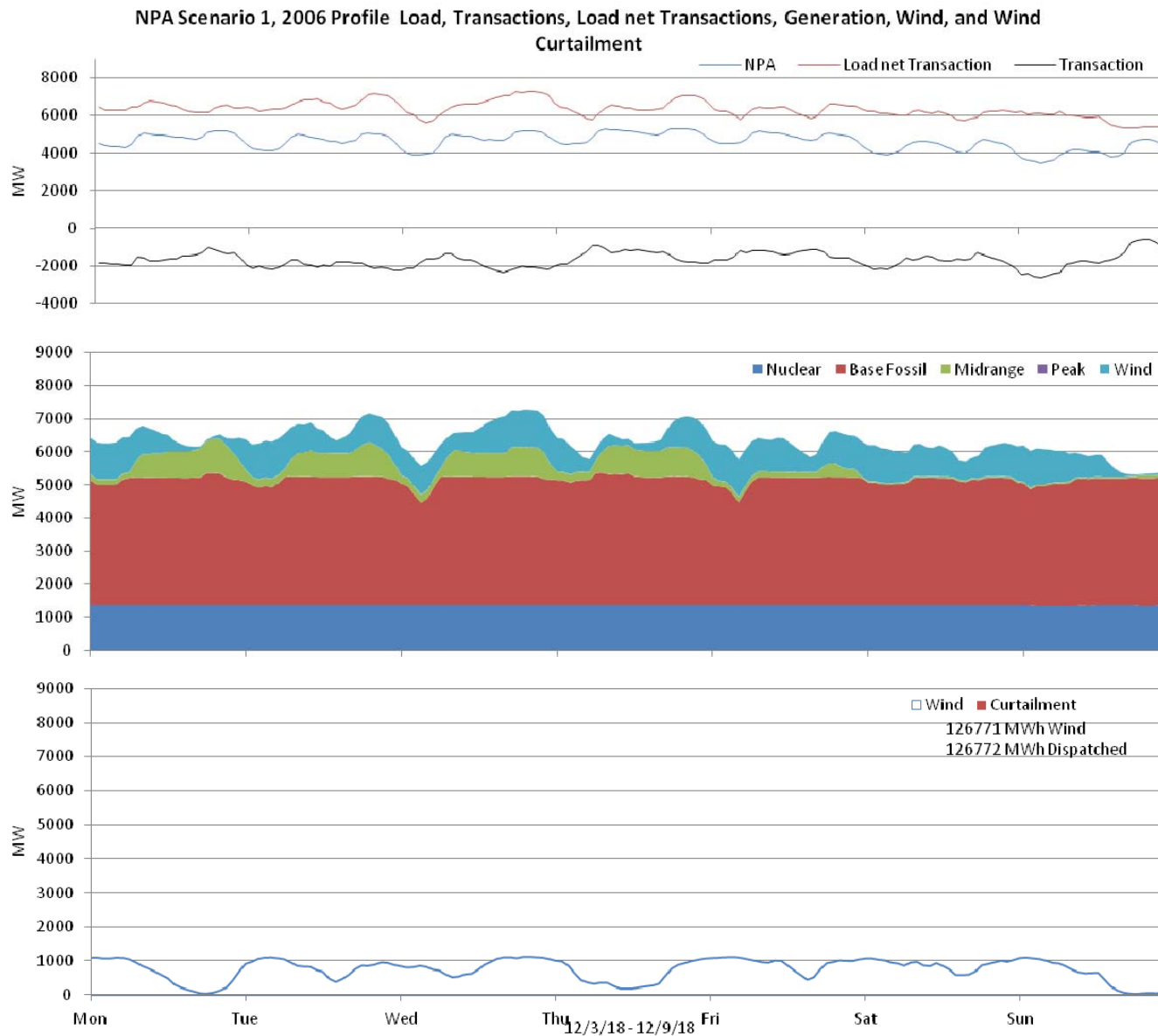
Figure 49: Nebraska 10% wind Penetration, 2006 Profile week of 12/3/2018
