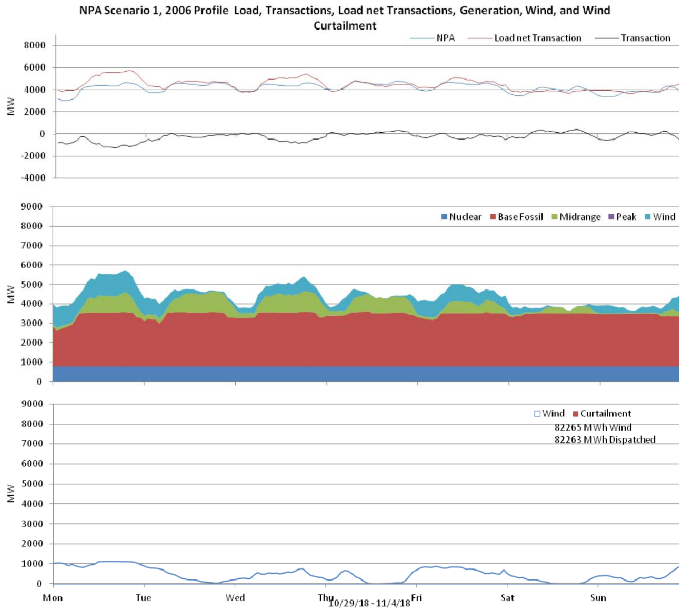
Figure 44: Nebraska 10% wind Penetration, 2006 Profile week of 10/29/2018
