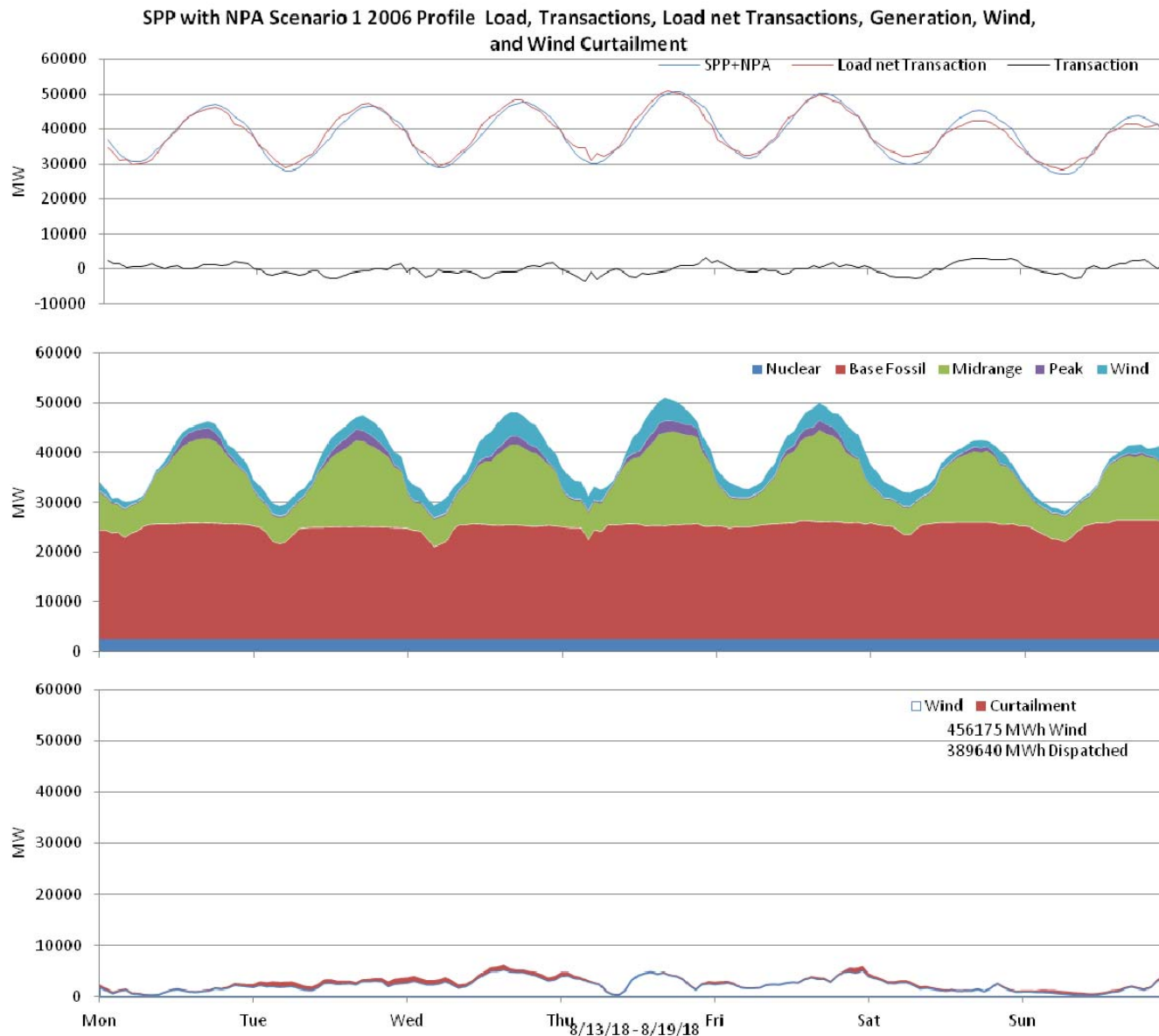
Figure 85: SPP 10% wind Penetration, 2006 Profile week of 8/13/2018
