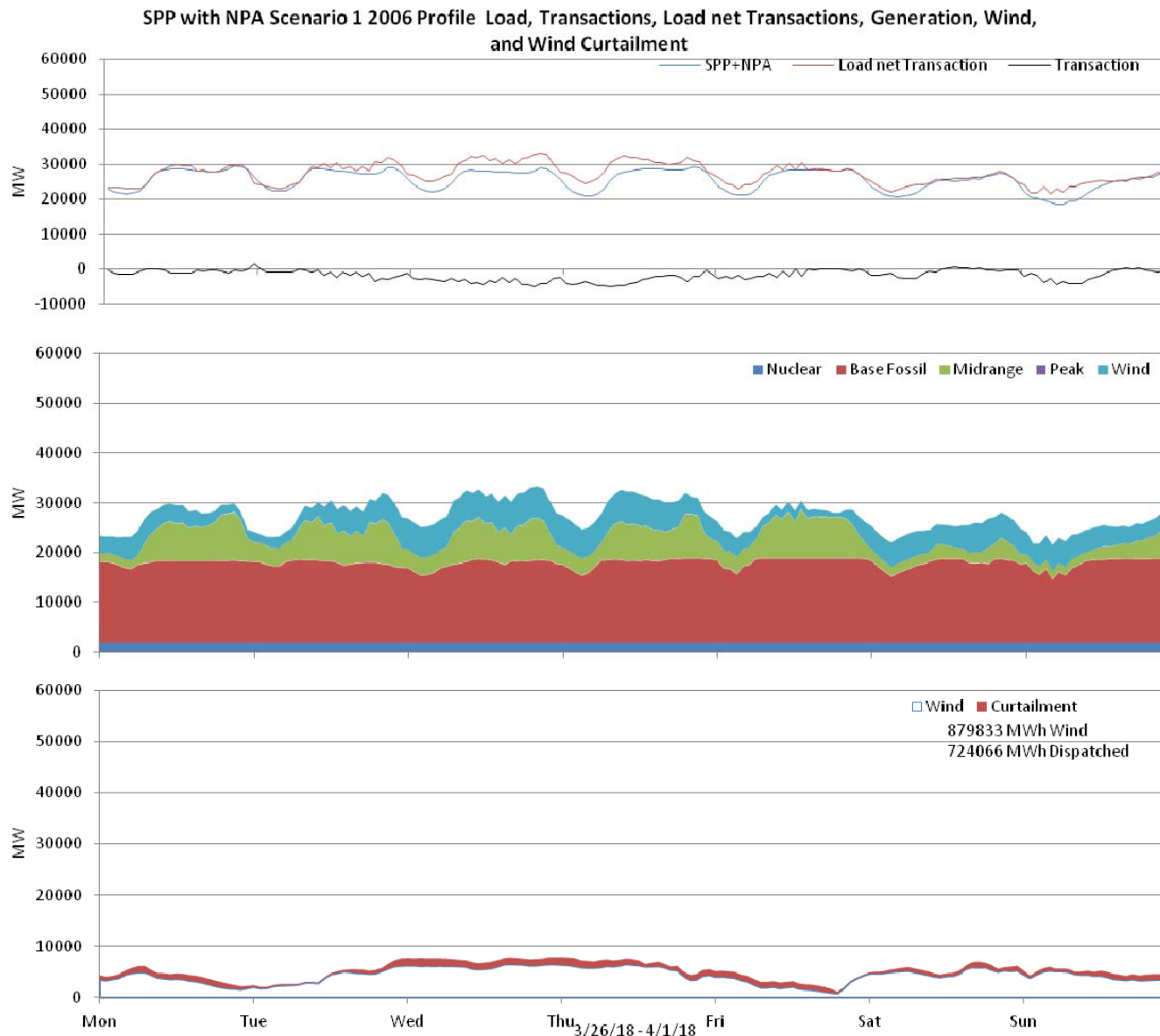
Figure 65: SPP 10% wind Penetration, 2006 Profile week of 3/26/2018
