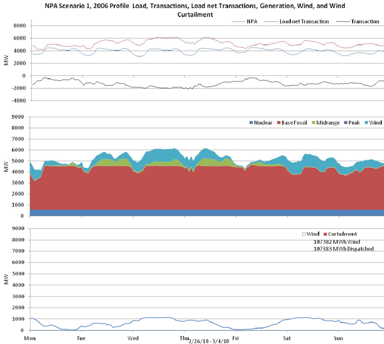
Figure 9: Nebraska 10% wind Penetration, 2006 Profile week of 2/26/2018
