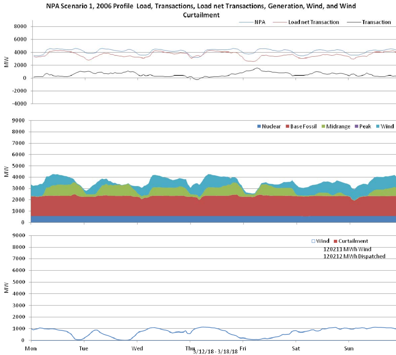
Figure 11: Nebraska 10% wind Penetration, 2006 Profile week of 3/12/2018
