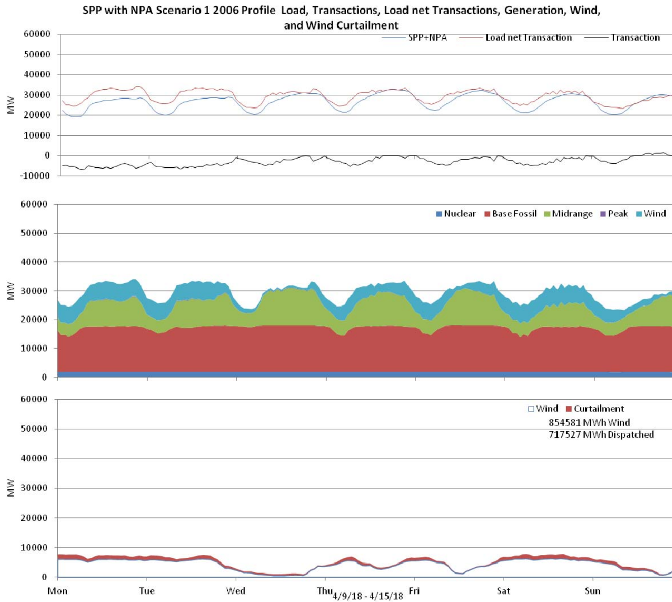
Figure 67: SPP 10% wind Penetration, 2006 Profile week of 4/9/2018
