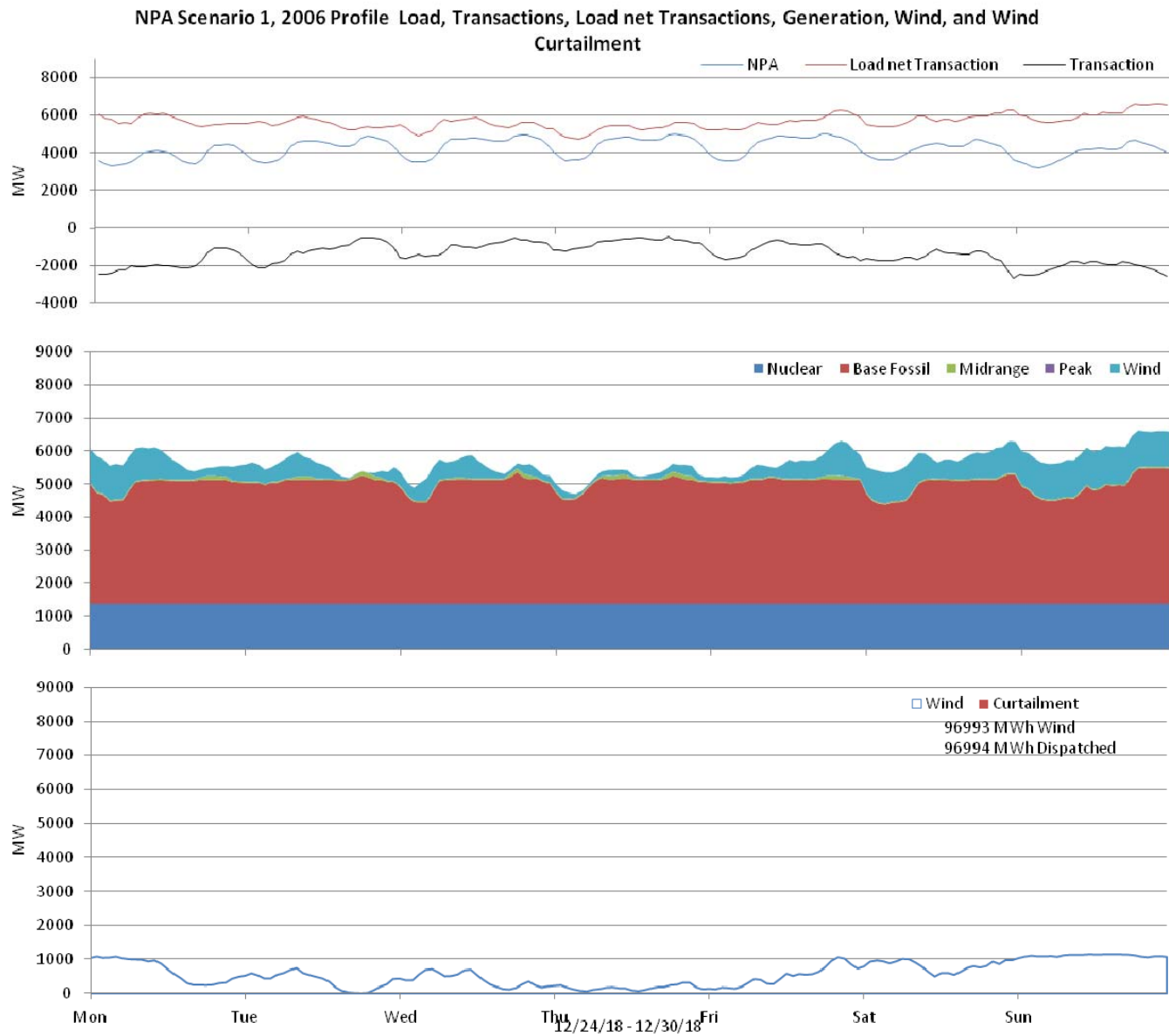
Figure 52: Nebraska 10% wind Penetration, 2006 Profile week of 12/24/2018
