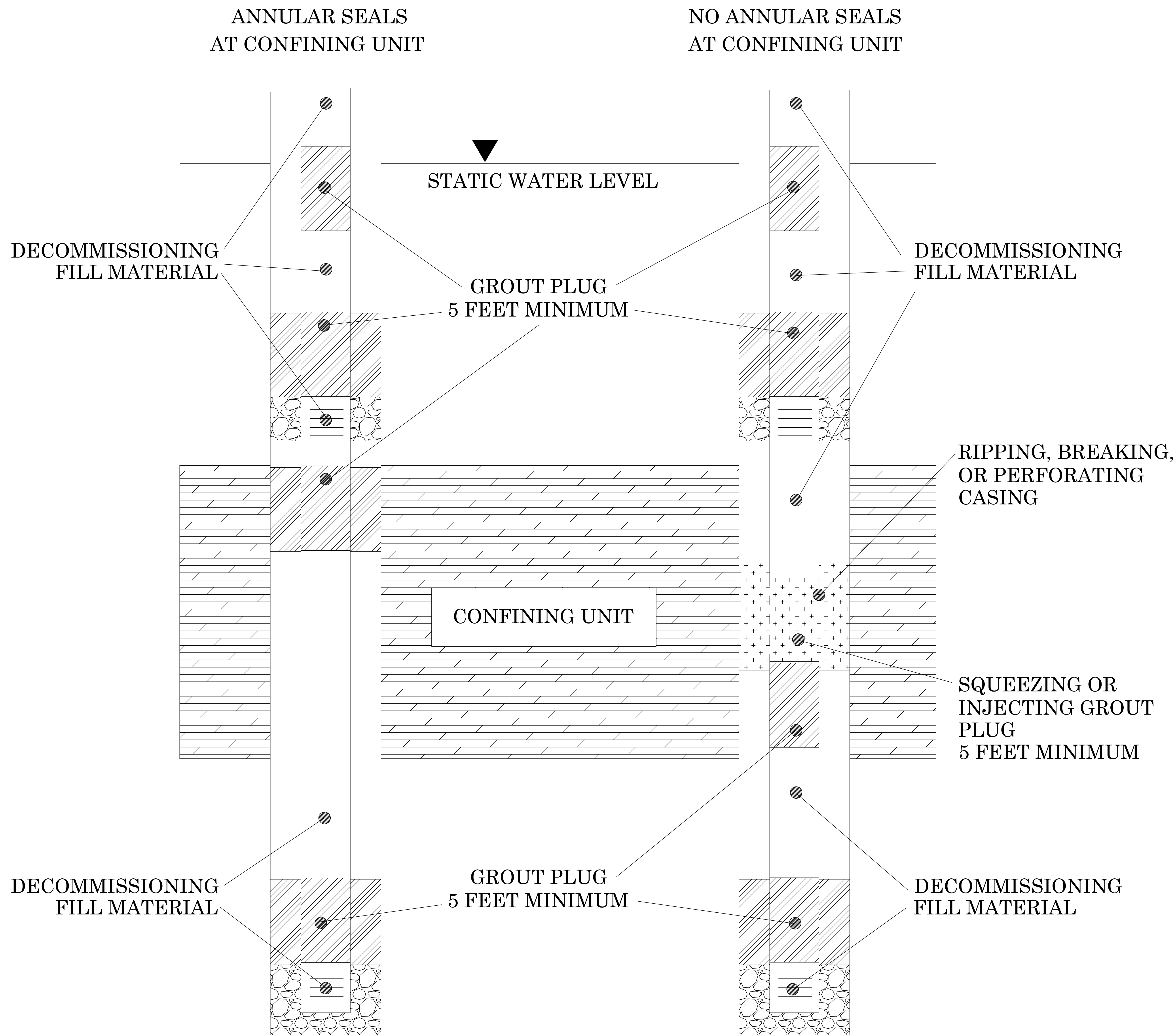
FIGURE 15 DECOMMISSIONING MULTIPLE AQUIFER WELLS/FLOWING WELLS
