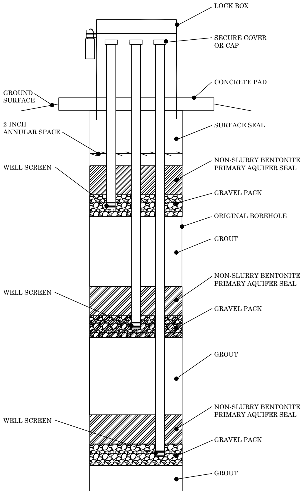
FIGURE 10 NESTED WELL DESIGN
