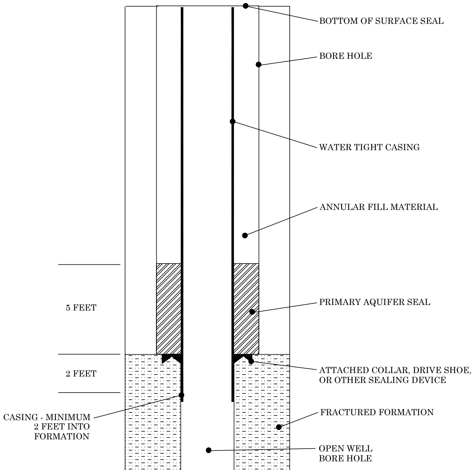
FIGURE 4 OPEN HOLE WELL CONSTRUCTION
